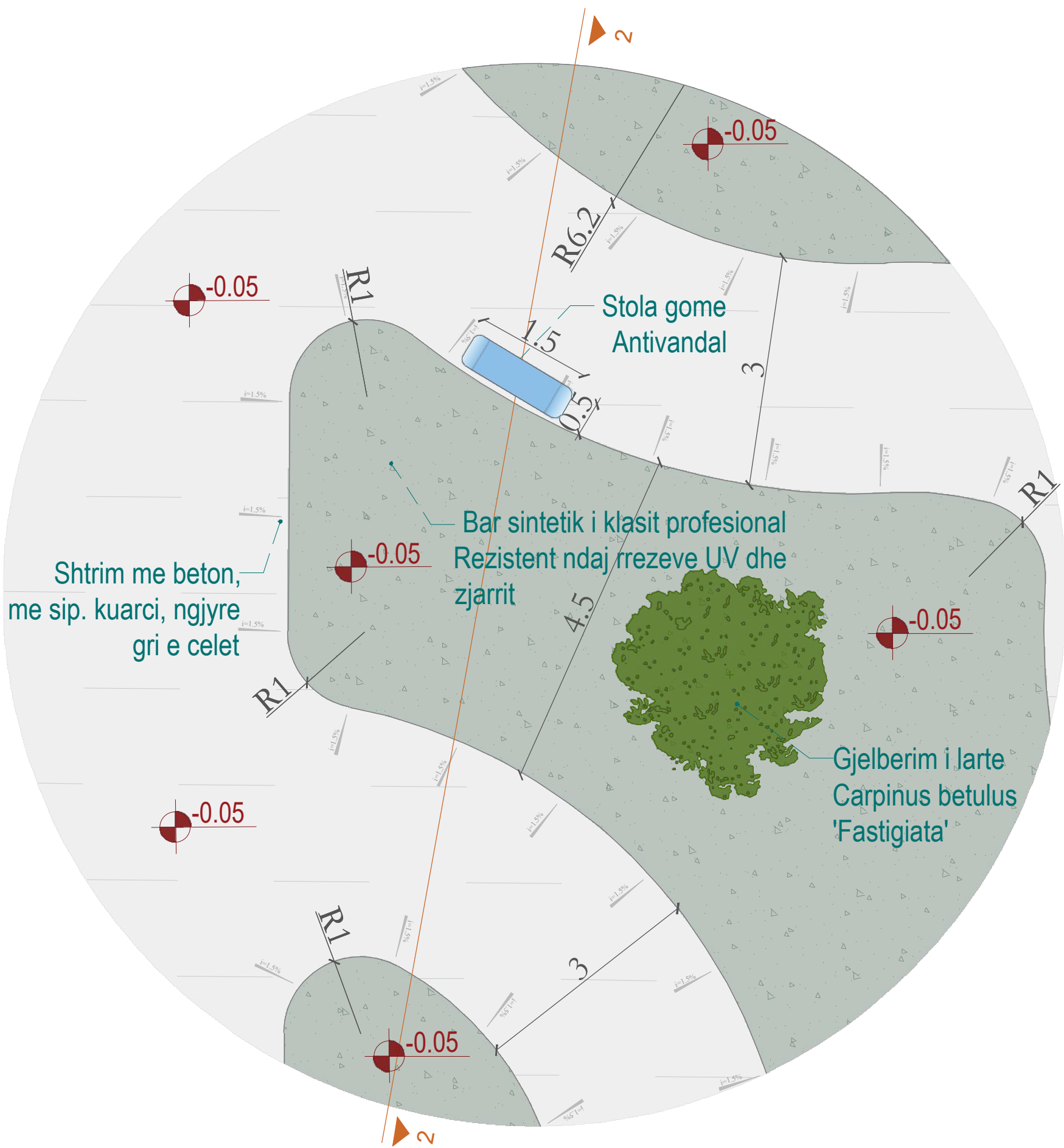
D2 - FRAGMENT PLAN SISTEMIMI - SH. 1:6
