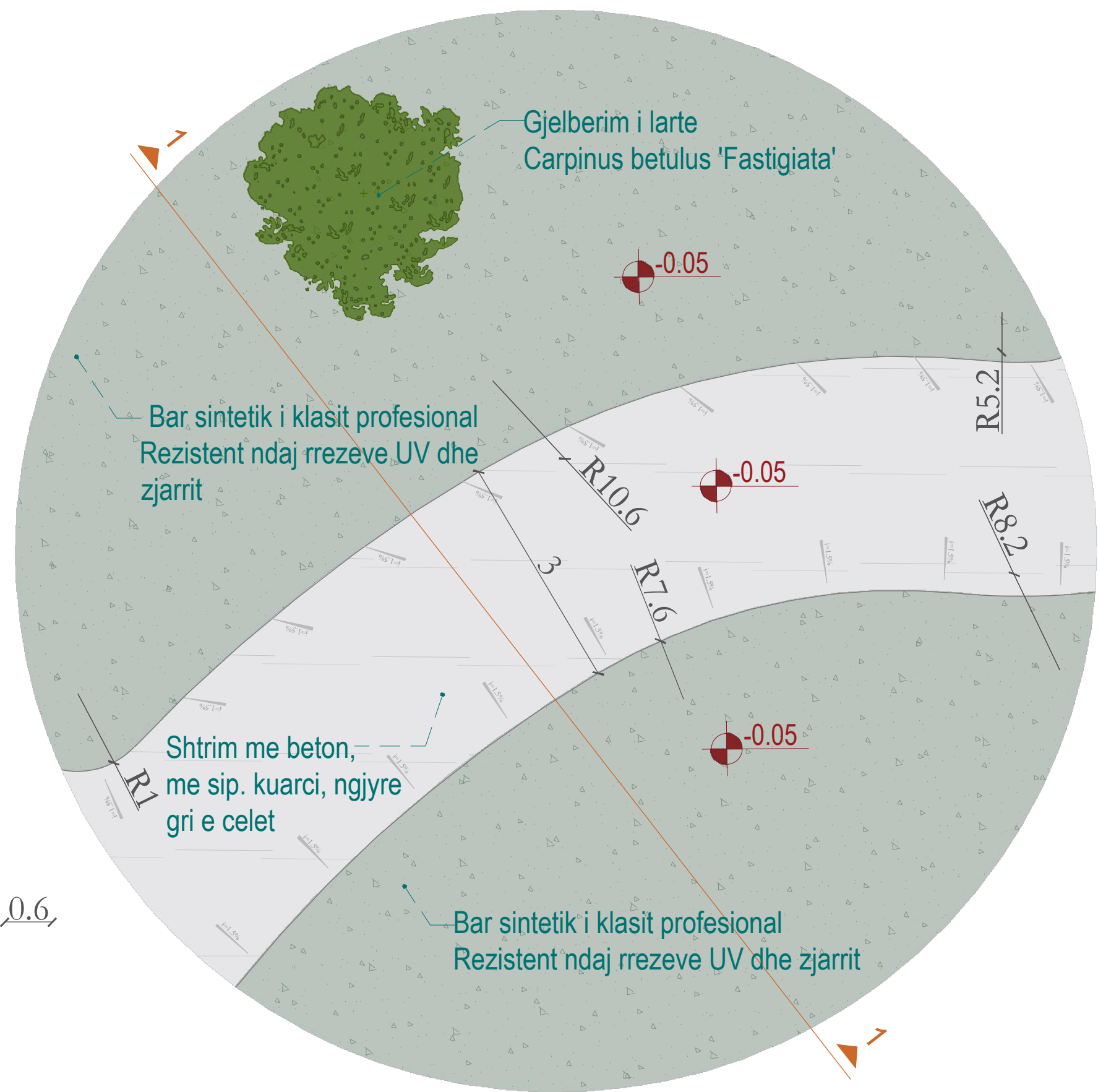
D2 - FRAGMENT PLAN SISTEMIMI - SH. 1:6
