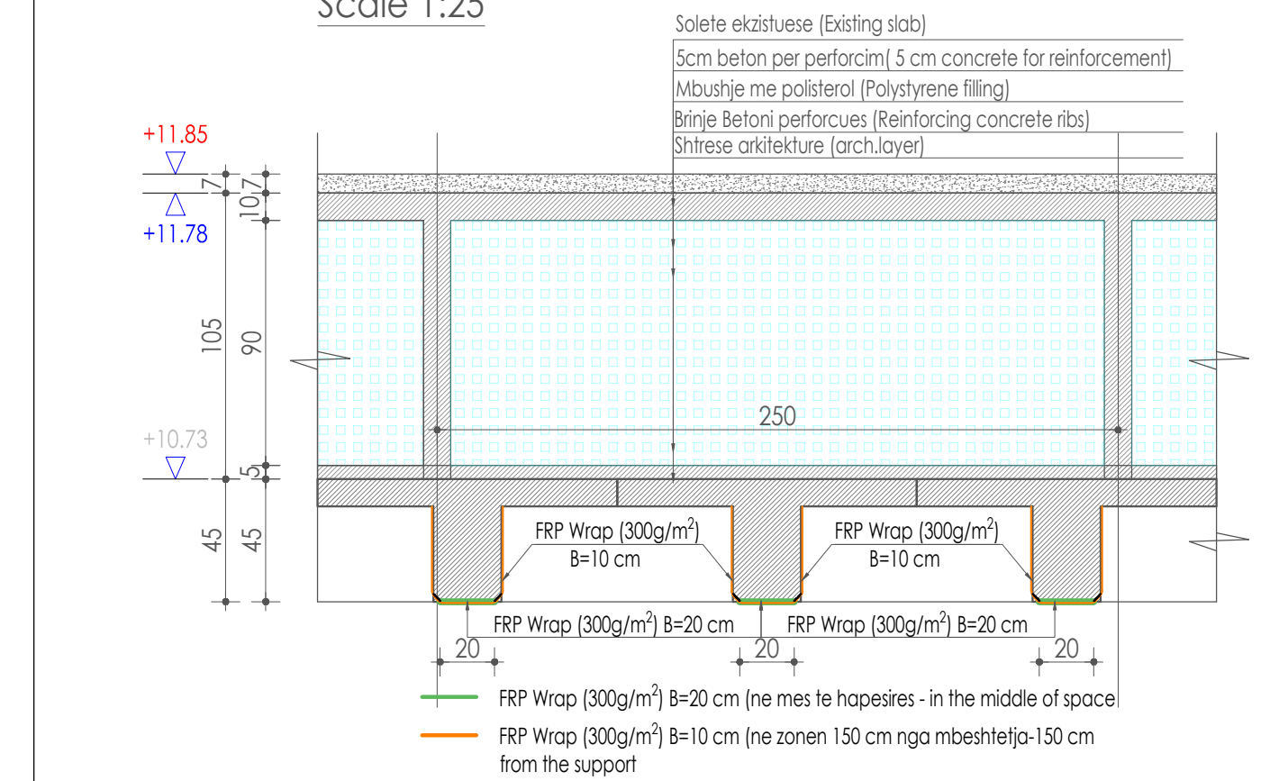
DETAJI 5 NE SOLETE Shkalla 1:25 DETAIL 5 IN R/C SLAB Scale 1:25
