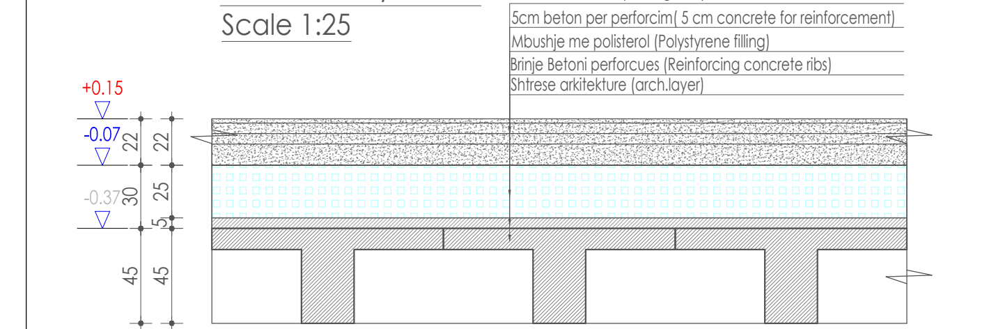
DETAJI 2 NE SOLETE Shkalla 1:25 DETAIL 2 IN R/C SLAB Scale 1:25
