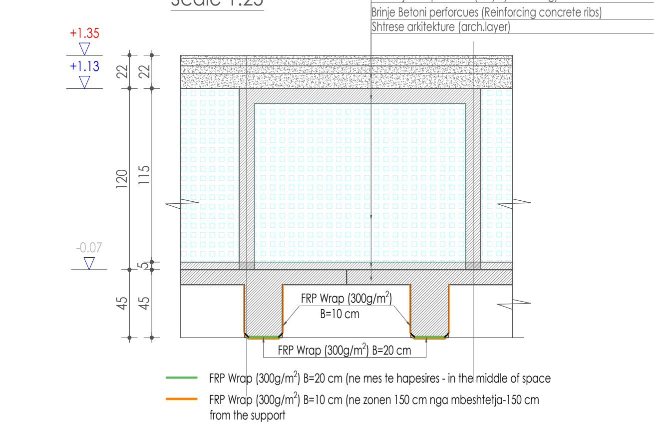
DETAJI 4 NE SOLETE Shkalla 1:25 DETAIL 4 IN R/C SLAB Scale 1:25
