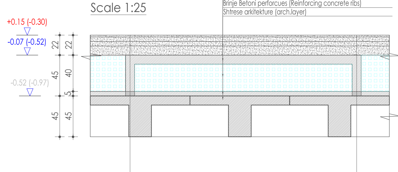
DETAJI 4 NE SOLETE Shkalla 1:25 DETAIL 4 IN R/C SLAB Scale 1:25
