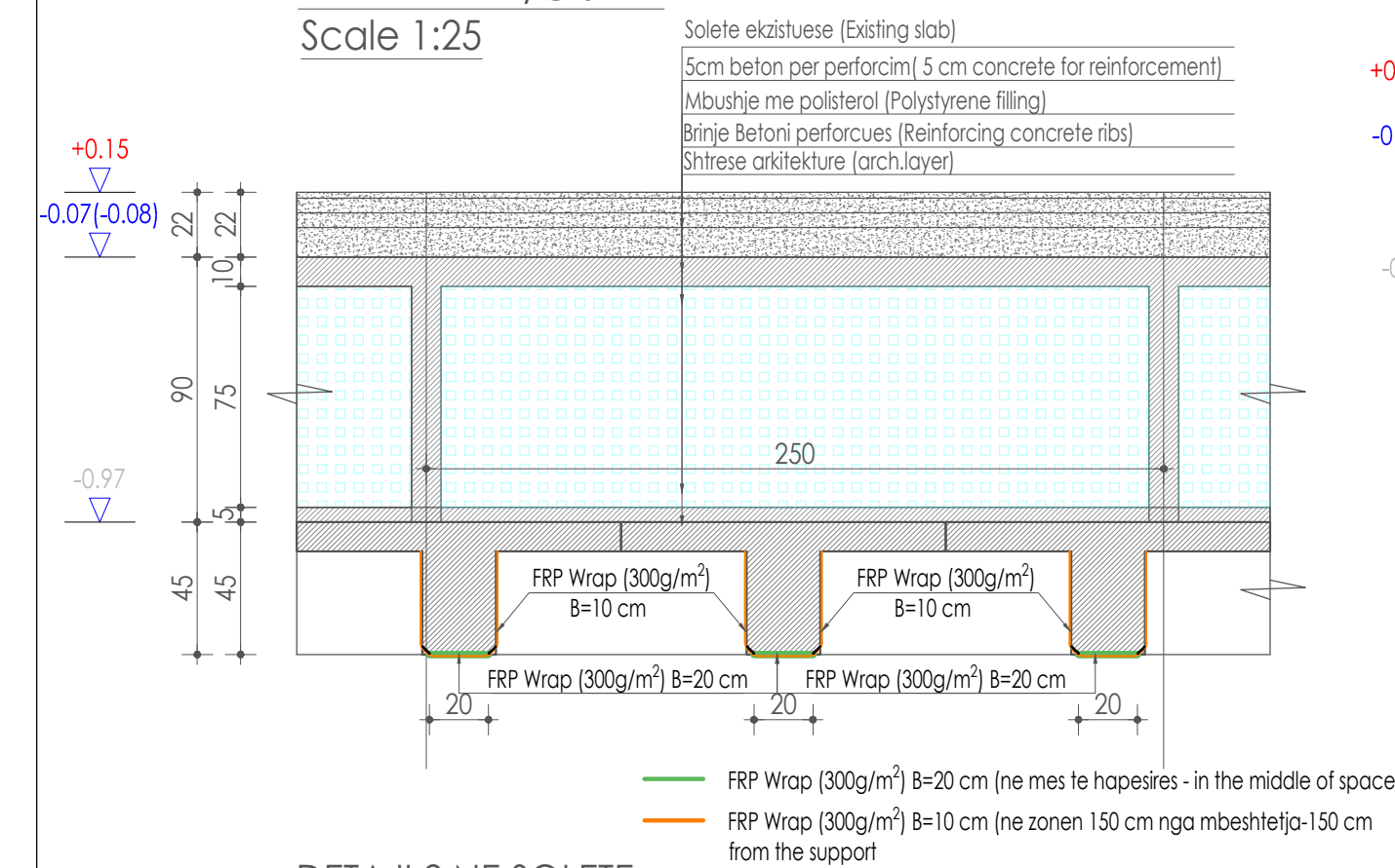
DETAJI 2 NE SOLETE Shkalla 1:25 DETAIL 2 IN R/C SLAB Scale 1:25
