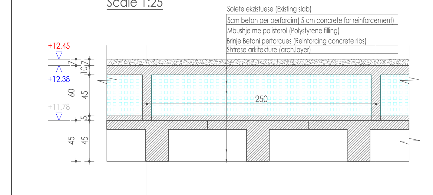
DETAJI 6 NE SOLETE Shkalla 1:25 DETAIL 6 IN R/C SLAB Scale 1:25
