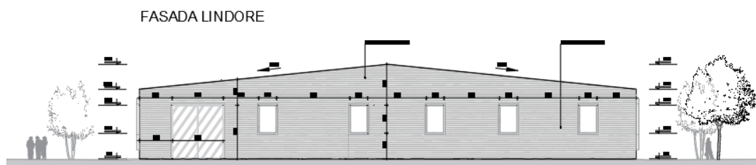
Figure 12. Fasada Perendimore, Objekti i Perpunitimit
