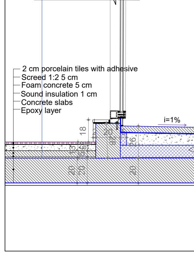
DF-06 FACADE DETAIL
