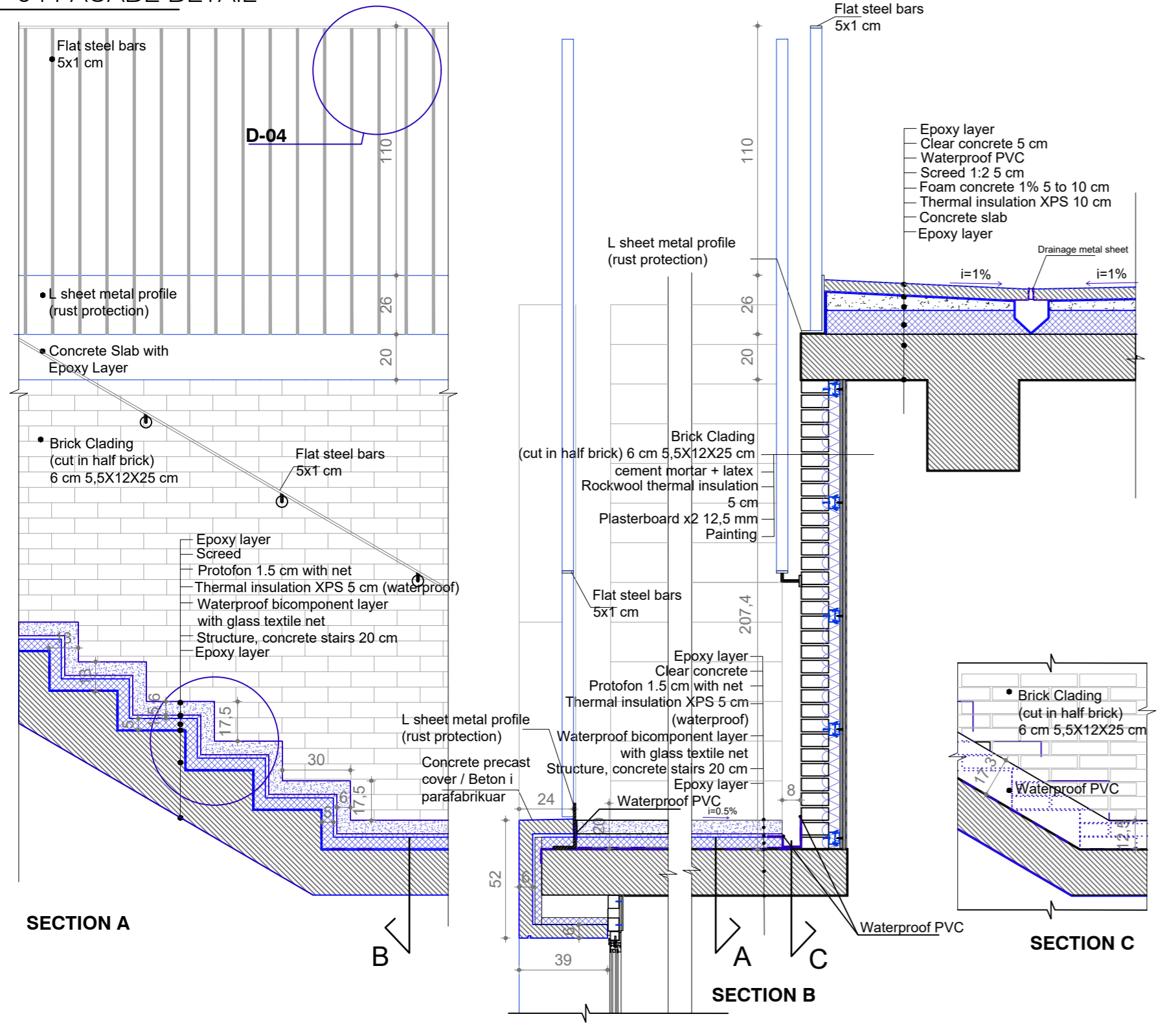
DF-01 FACADE DETAIL
