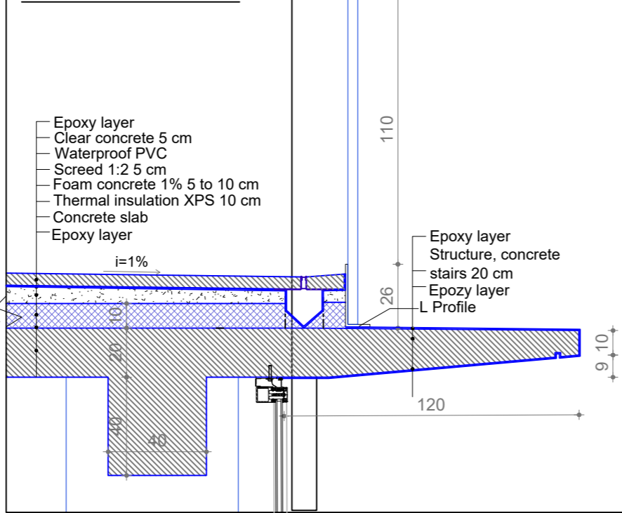
DF-03 FACADE DETAIL
