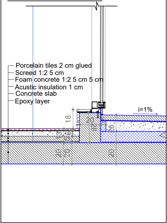
DF-01 FACADE DETAIL
