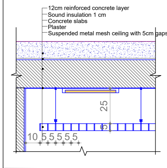
T-01 SUSPENDED MESH CEILING HALLWAY
