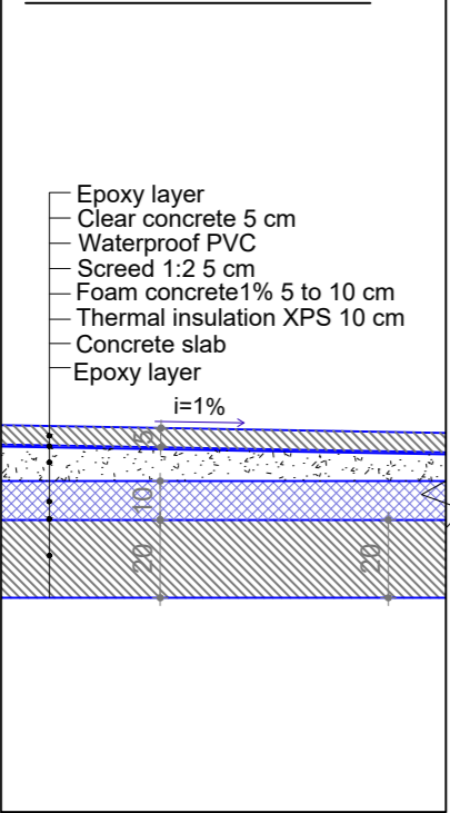
DF-02 DETAIL
