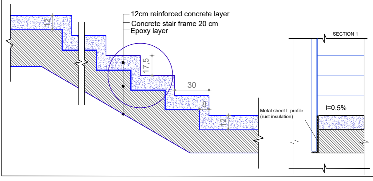
F-02B POLISHED CONCRETE ENTRANCE STAIRS
