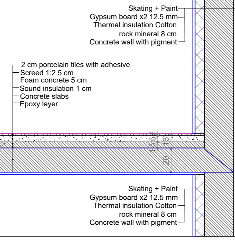
DF-07 FACADE DETAIL
