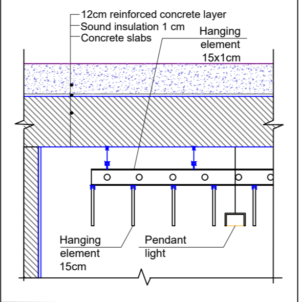
T-03 SUSPENDED CEILING-HALL
