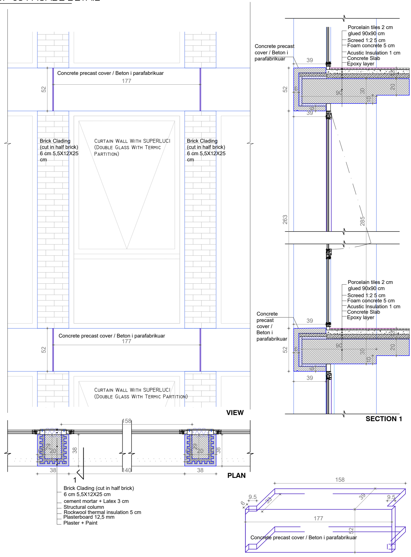
DF-05 FACADE DETAIL
