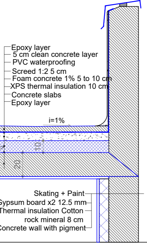
DF-08 FACADE DETAIL
