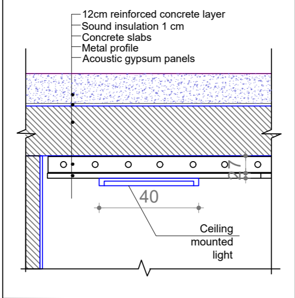
T-02 ACOUSTICAL CEILING-CLASS
