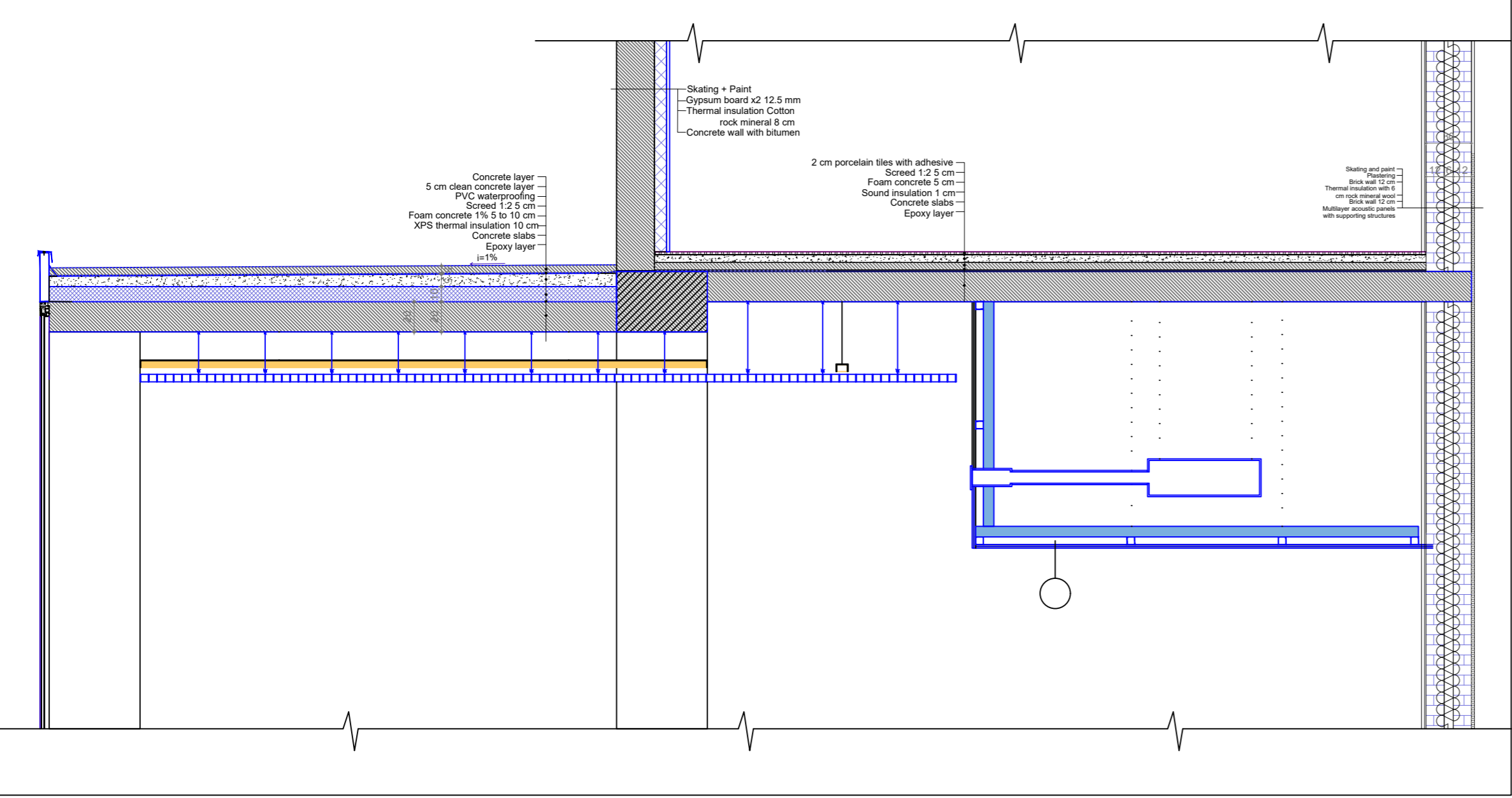
T-03 CEILING DETAIL IN THE CANTEN AREA
