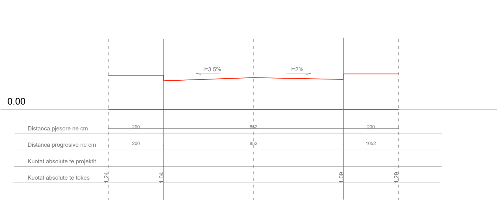
Prerja 14-14
