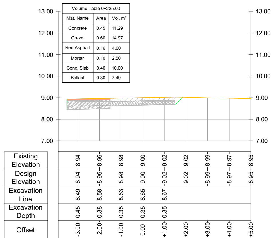
CROSS SECTION Road Nr. 7 - Recreational Park - Prog.: 0+225.00
