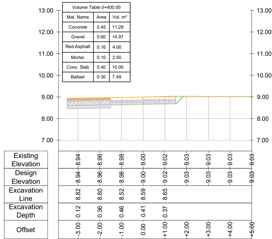
CROSS SECTION Road Nr. 7 - Recreational Park - Prog.: 0+400.00
