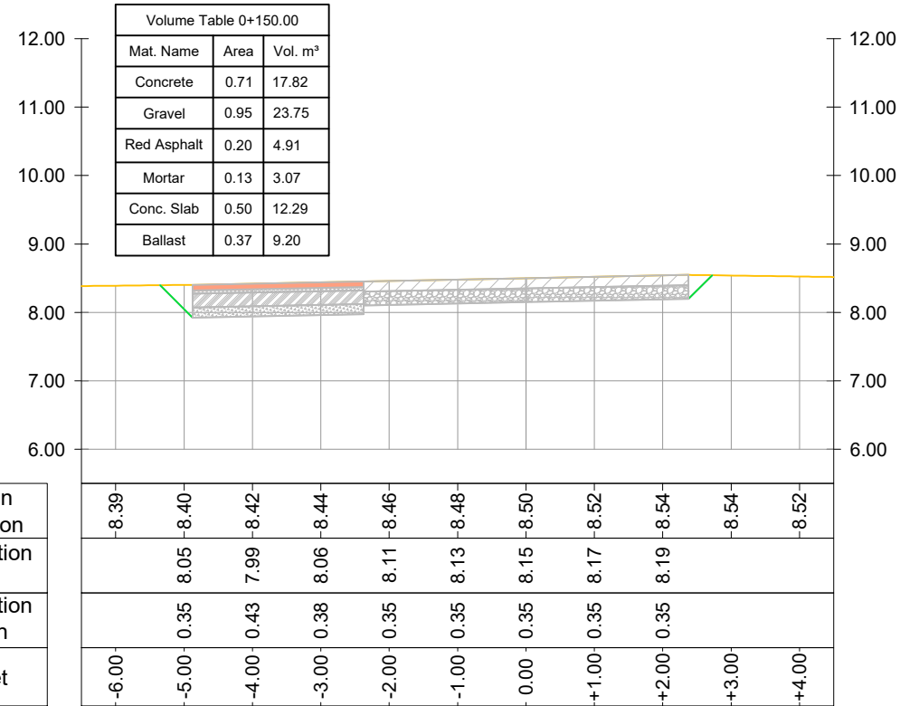
CROSS SECTION Road Nr. 8 - Recreational Park - Prog.: 0+150.00
