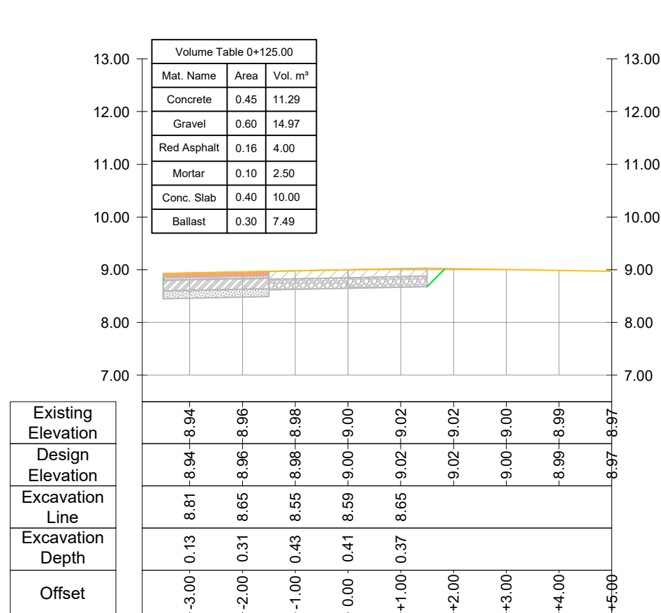
CROSS SECTION Road Nr. 7 - Recreational Park - Prog.: 0+125.00
