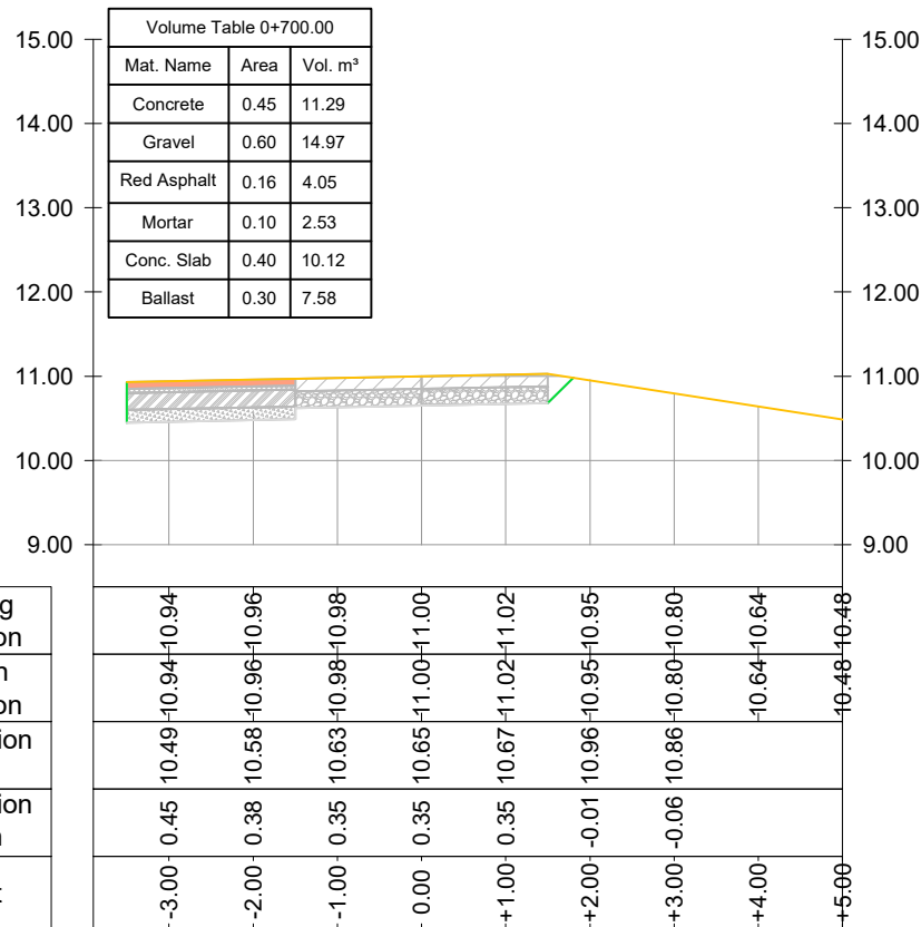
CROSS SECTION Road Nr. 7 - Recreational Park - Prog.: 0+700.00
