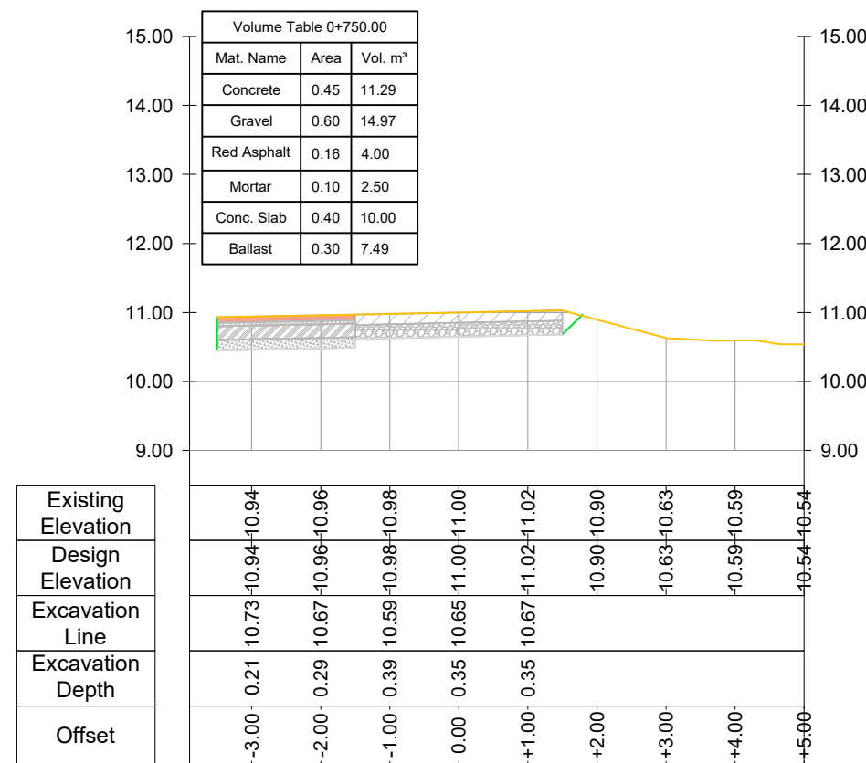
CROSS SECTION Road Nr. 7 - Recreational Park - Prog.: 0+750.00
