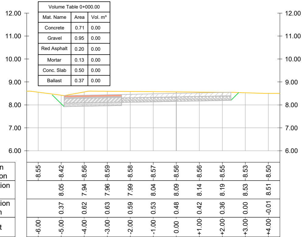
CROSS SECTION Road Nr. 8 - Recreational Park - Prog.: 0+000.00
