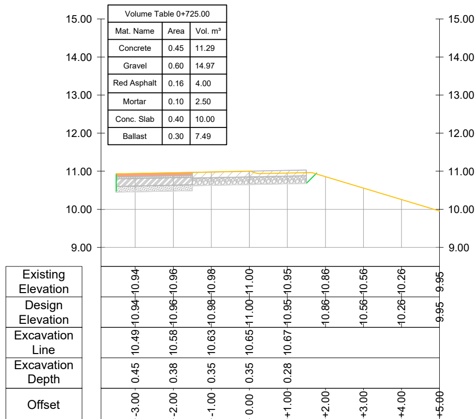
CROSS SECTION Road Nr. 7 - Recreational Park - Prog.: 0+725.00
