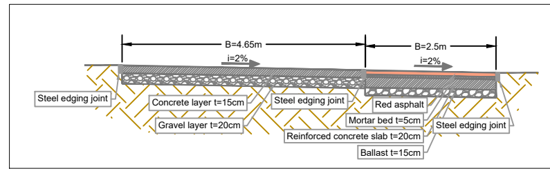
TYPICAL SECTION Prog. 0+234.00 - 0+477.00 SCALE 1:100
