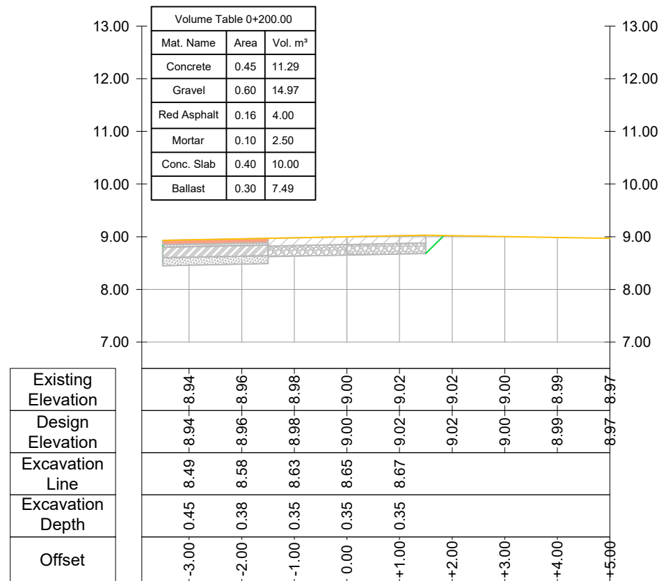
CROSS SECTION Road Nr. 7 - Recreational Park - Prog.: 0+200.00
