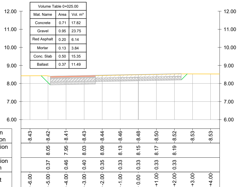
CROSS SECTION Road Nr. 8 - Recreational Park - Prog.: 0+025.00
