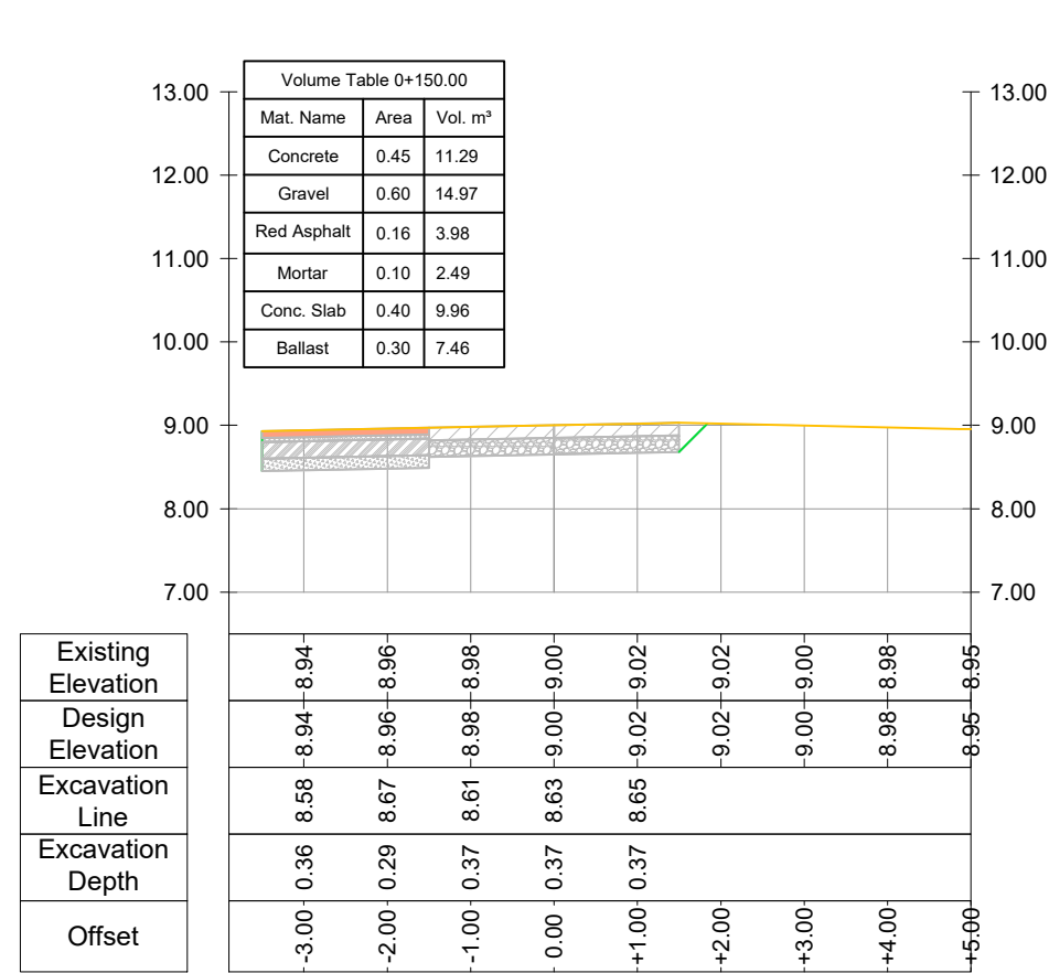
CROSS SECTION Road Nr. 7 - Recreational Park - Prog.: 0+150.00
