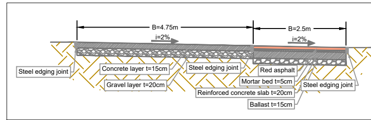
TYPICAL SECTION Prog. 0+000.00 - 0+234.00 SCALE 1:100
