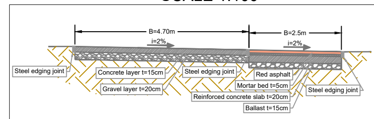
TYPICAL SECTION Prog. 0+477.00 - 0+569.00 SCALE 1:100
