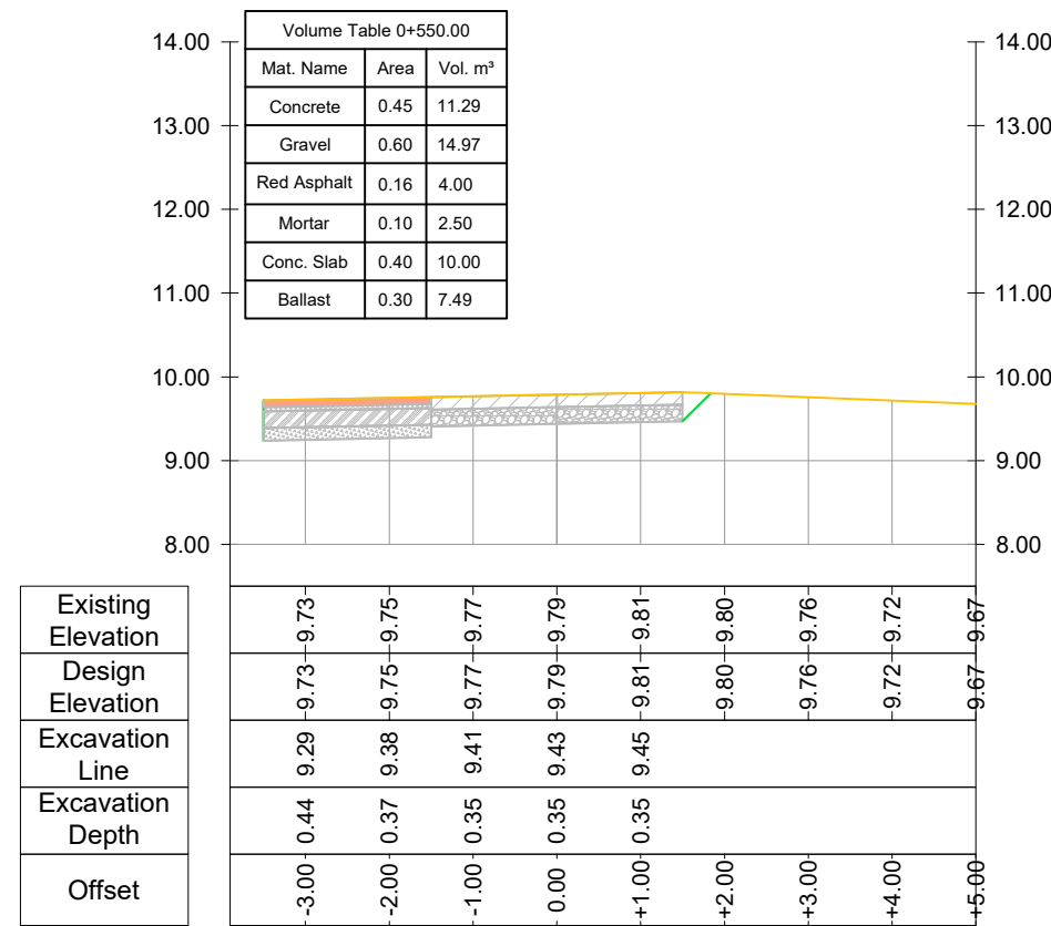
CROSS SECTION Road Nr. 7 - Recreational Park - Prog.: 0+550.00
