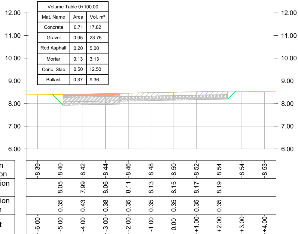
CROSS SECTION Road Nr. 8 - Recreational Park - Prog.: 0+100.00
