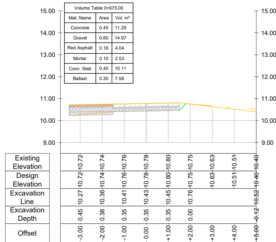
CROSS SECTION Road Nr. 7 - Recreational Park - Prog.: 0+675.00
