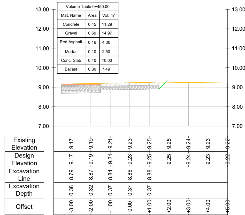
CROSS SECTION Road Nr. 7 - Recreational Park - Prog.: 0+450.00
