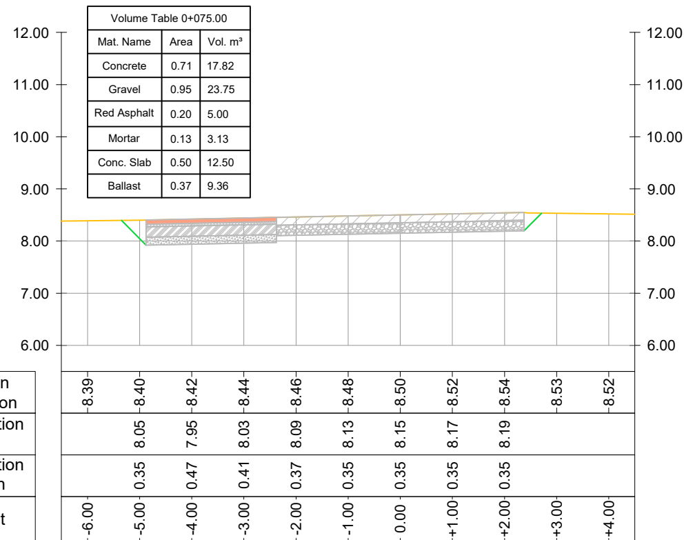
CROSS SECTION Road Nr. 8 - Recreational Park - Prog.: 0+075.00
