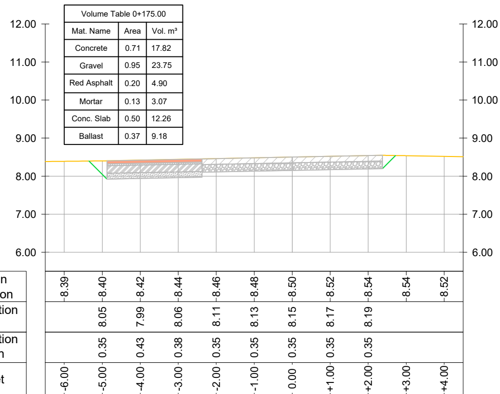
CROSS SECTION Road Nr. 8 - Recreational Park - Prog.: 0+175.00
