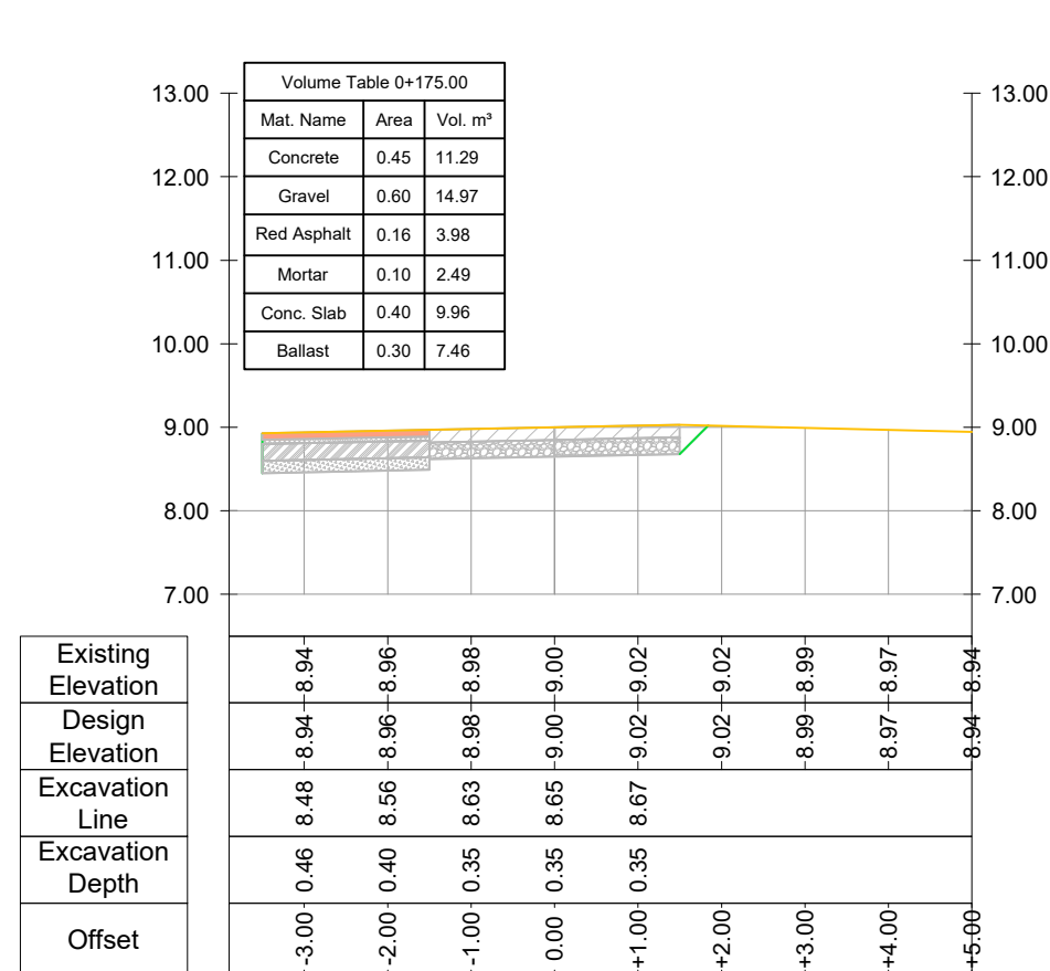
CROSS SECTION Road Nr. 7 - Recreational Park - Prog.: 0+175.00
