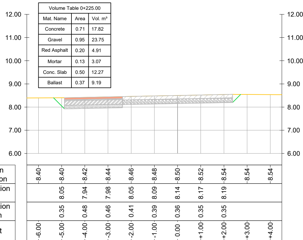
CROSS SECTION Road Nr. 8 - Recreational Park - Prog.: 0+225.00
