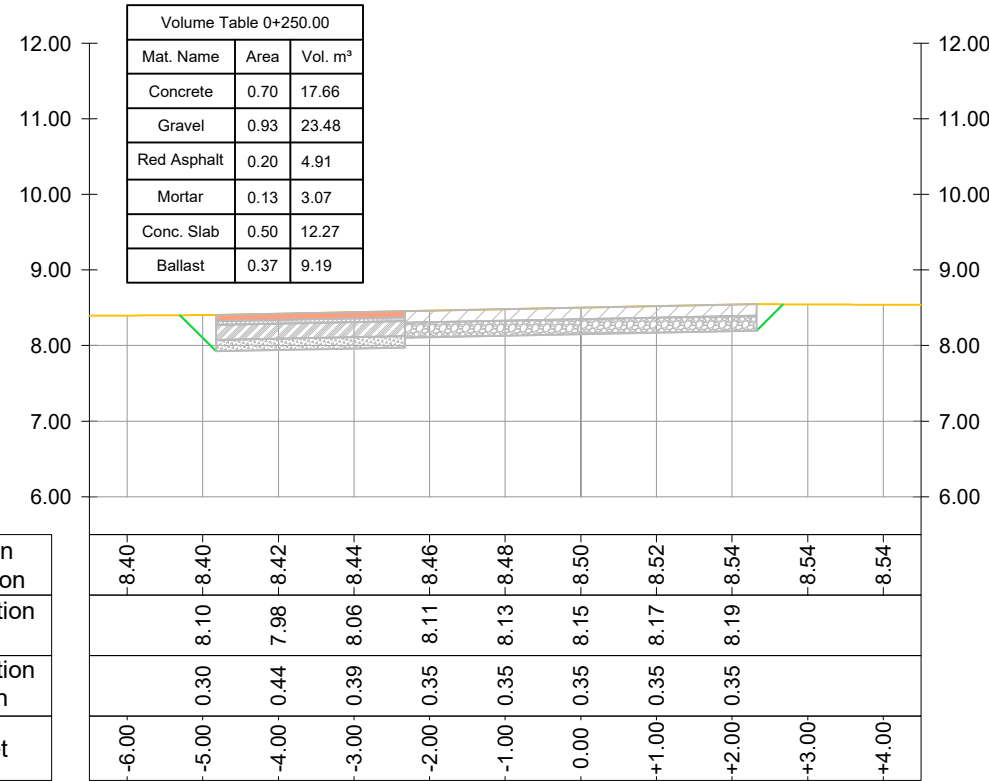
CROSS SECTION Road Nr. 8 - Recreational Park - Prog.: 0+250.00
