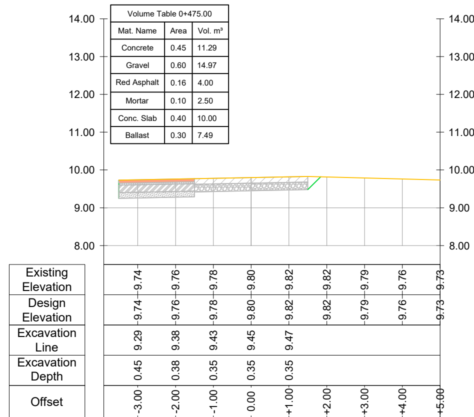
CROSS SECTION Road Nr. 7 - Recreational Park - Prog.: 0+475.00
