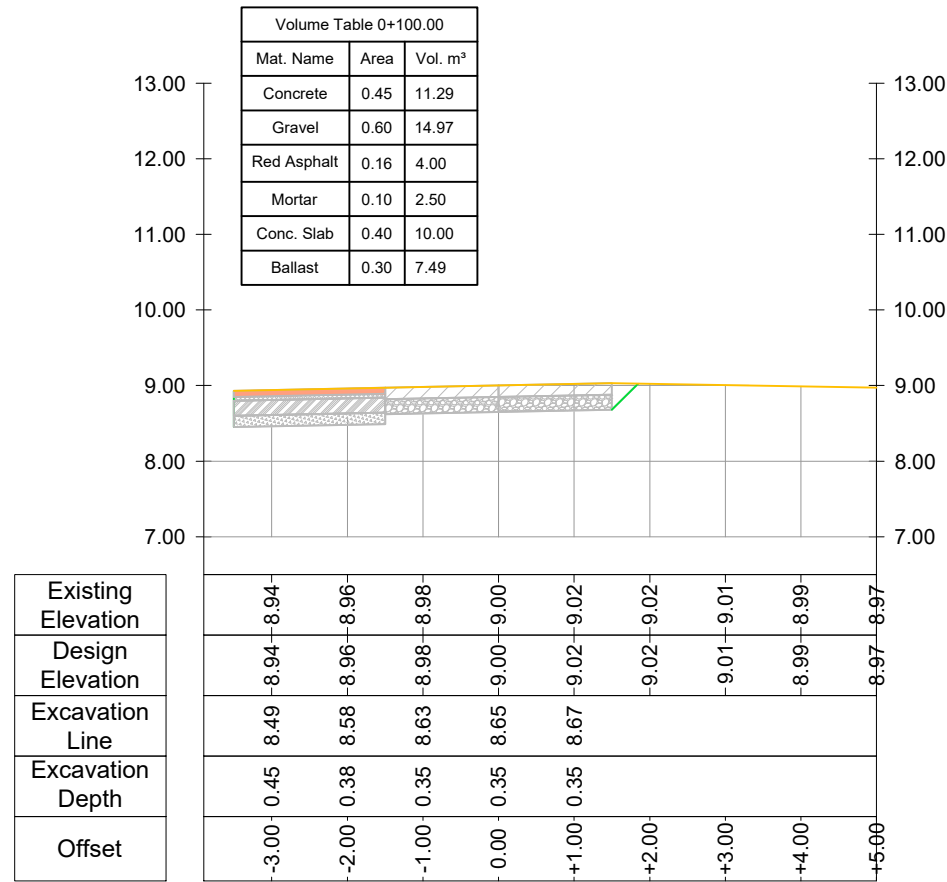
CROSS SECTION Road Nr. 7 - Recreational Park - Prog.: 0+100.00
