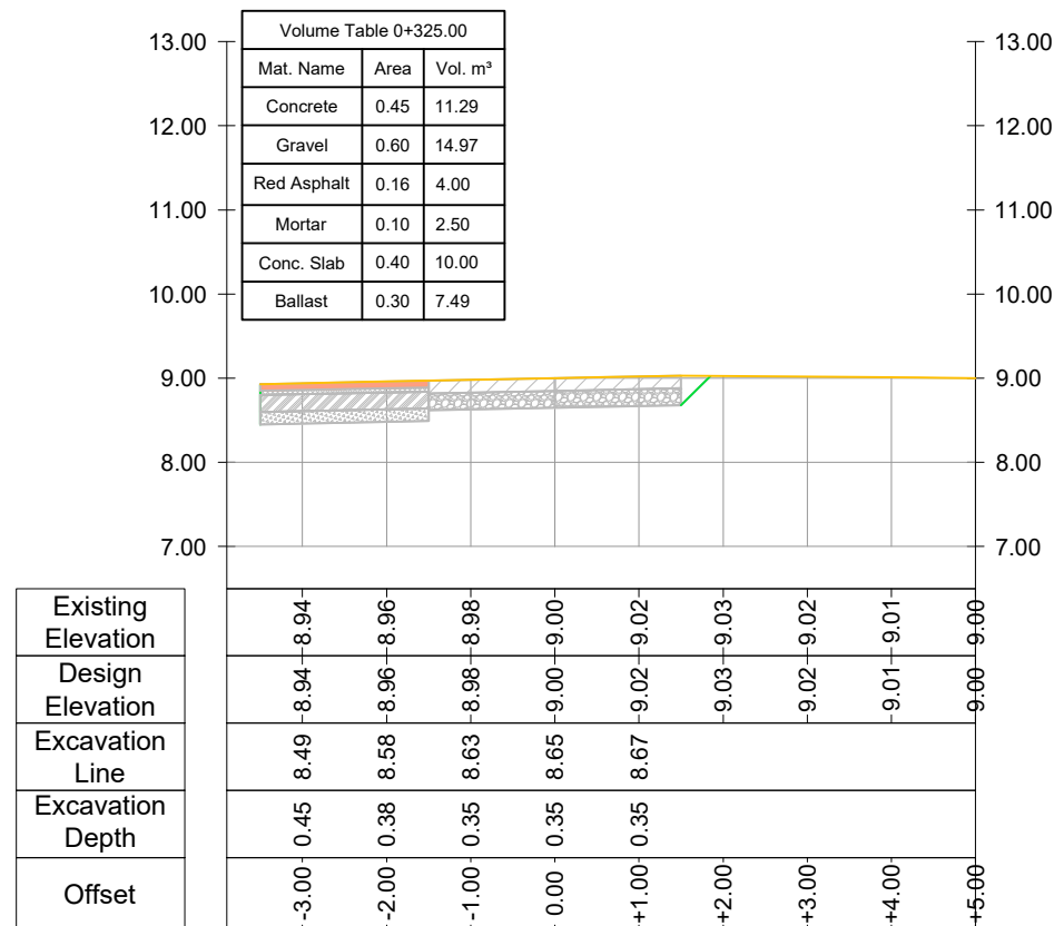
CROSS SECTION Road Nr. 7 - Recreational Park - Prog.: 0+325.00
