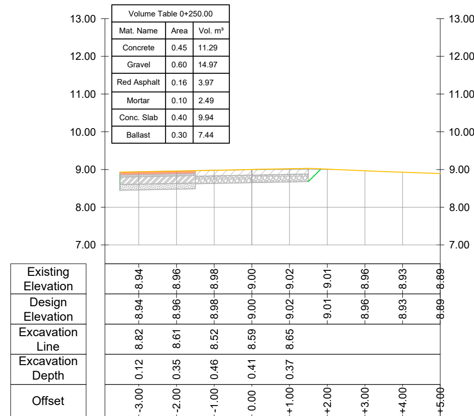
CROSS SECTION Road Nr. 7 - Recreational Park - Prog.: 0+250.00
