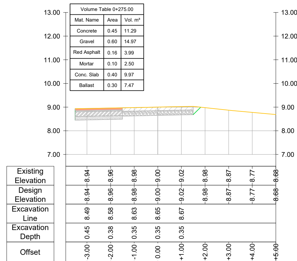
CROSS SECTION Road Nr. 7 - Recreational Park - Prog.: 0+275.00
