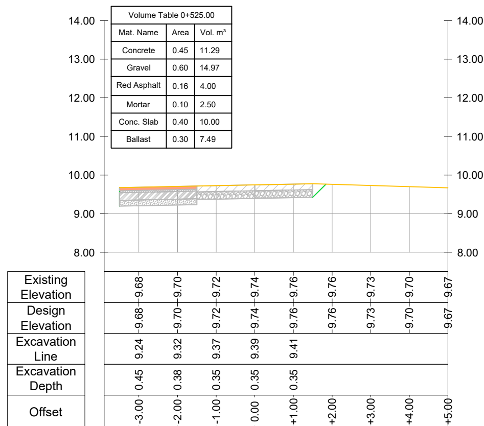
CROSS SECTION Road Nr. 7 - Recreational Park - Prog.: 0+525.00
