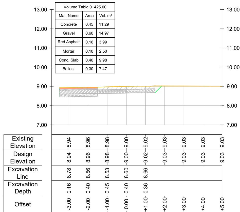
CROSS SECTION Road Nr. 7 - Recreational Park - Prog.: 0+425.00
