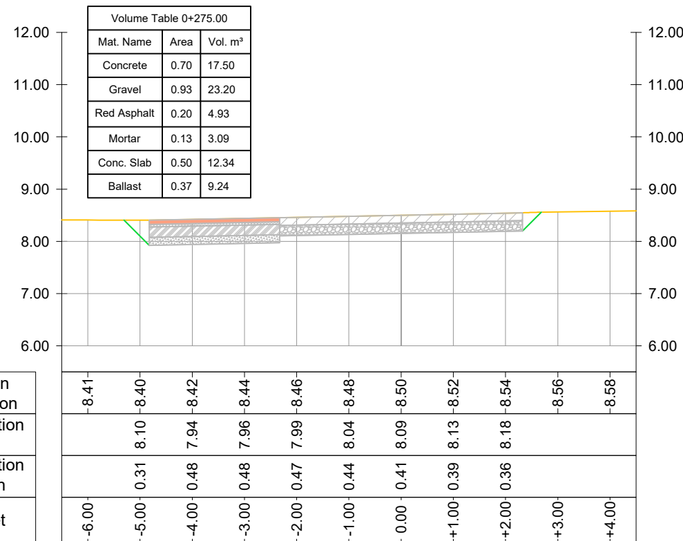
CROSS SECTION Road Nr. 8 - Recreational Park - Prog.: 0+275.00
