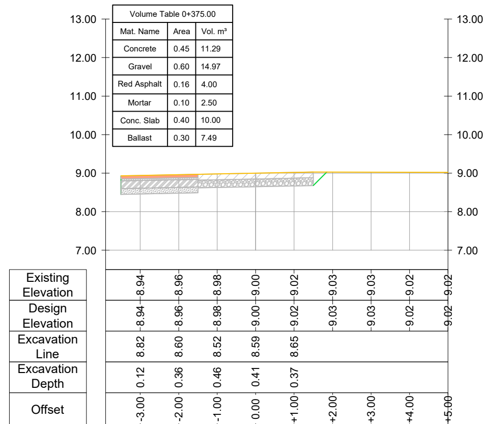
CROSS SECTION Road Nr. 7 - Recreational Park - Prog.: 0+375.00
