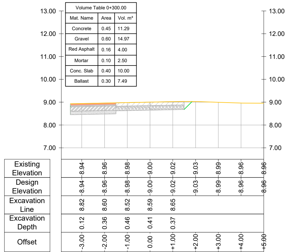
CROSS SECTION Road Nr. 7 - Recreational Park - Prog.: 0+300.00
