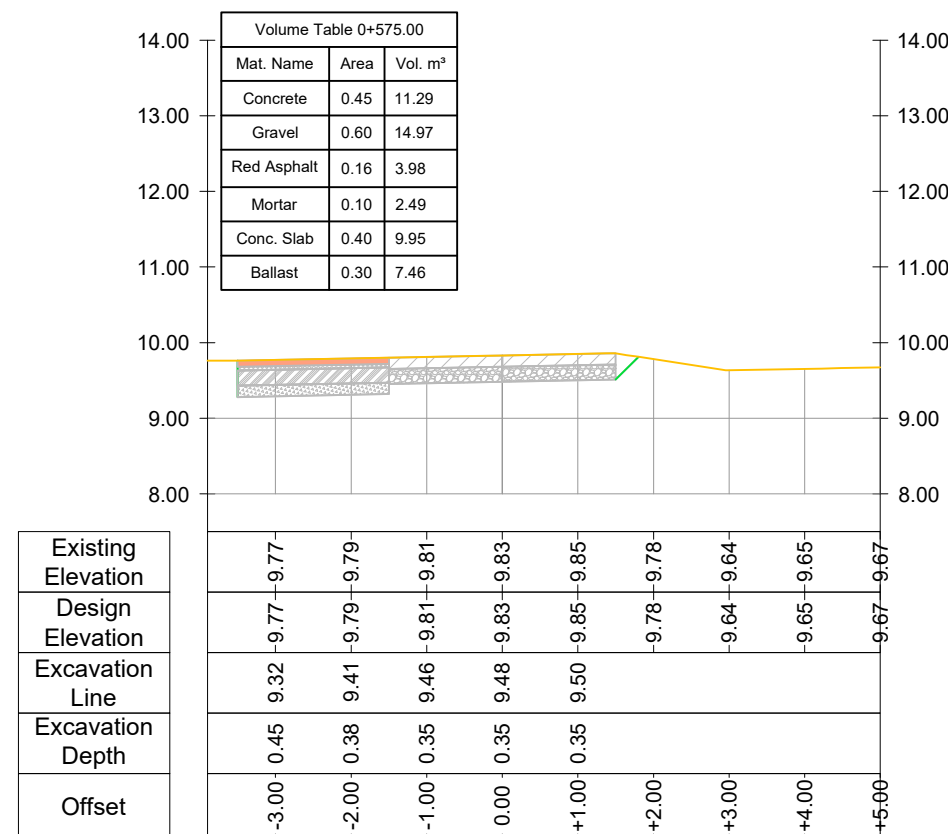
CROSS SECTION Road Nr. 7 - Recreational Park - Prog.: 0+575.00
