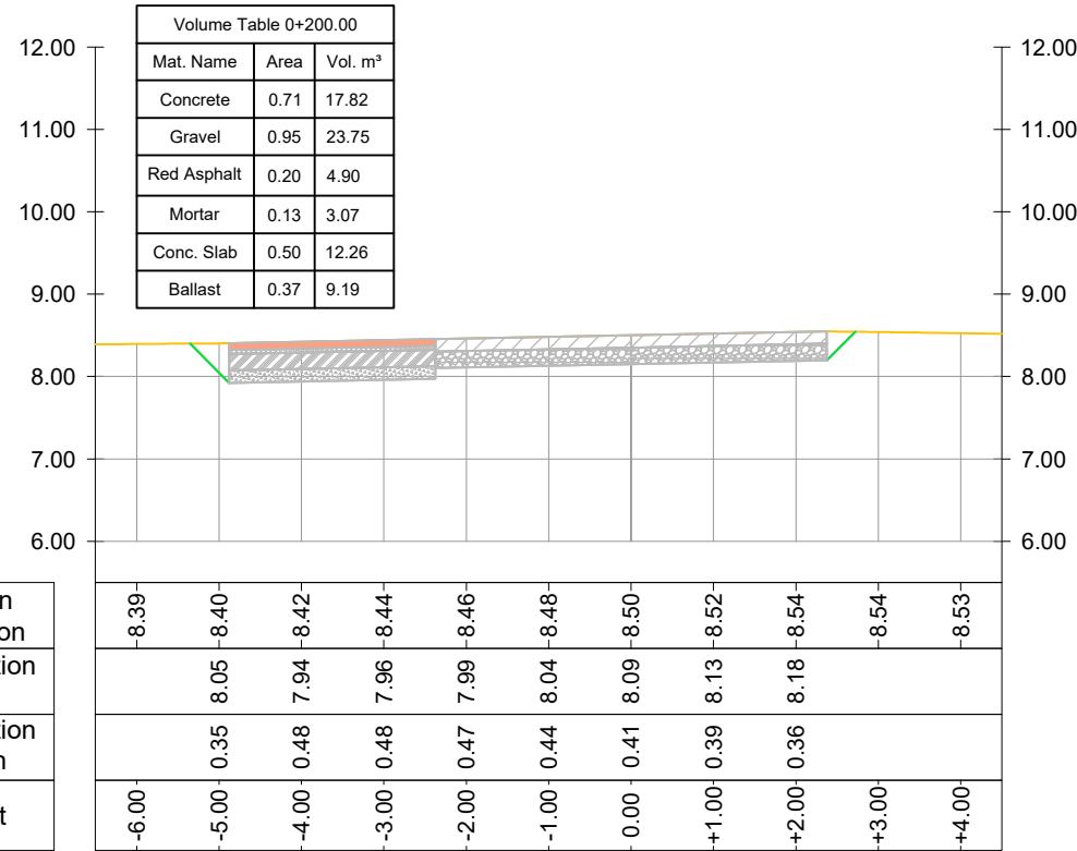
CROSS SECTION Road Nr. 8 - Recreational Park - Prog.: 0+200.00
