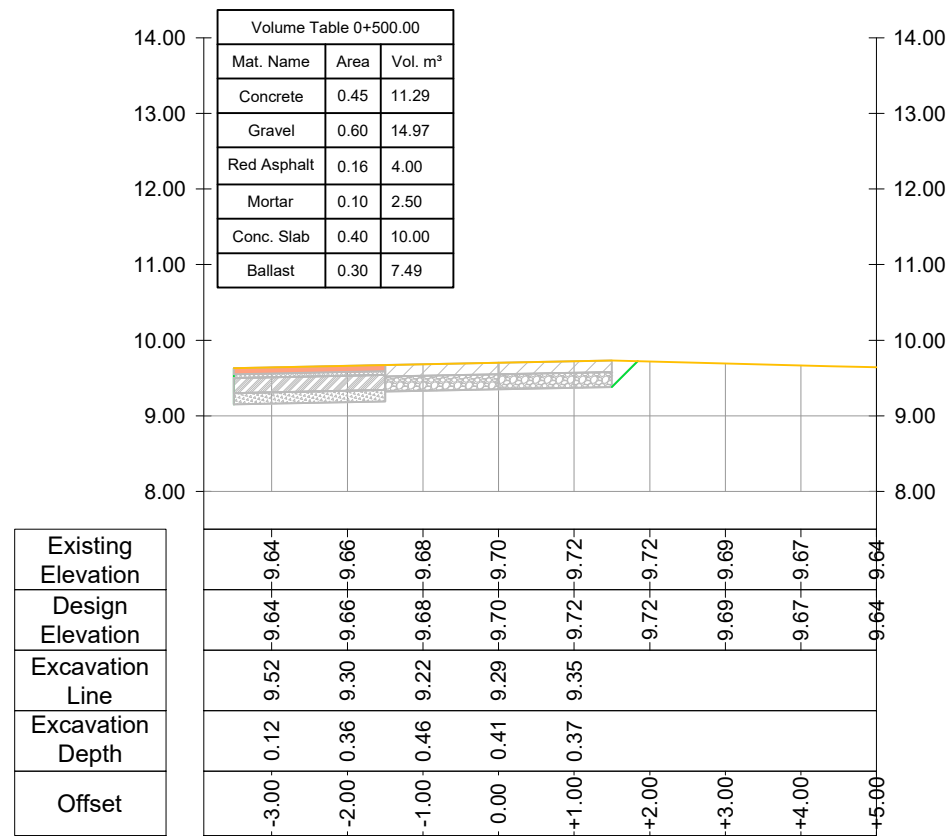
CROSS SECTION Road Nr. 7 - Recreational Park - Prog.: 0+500.00
