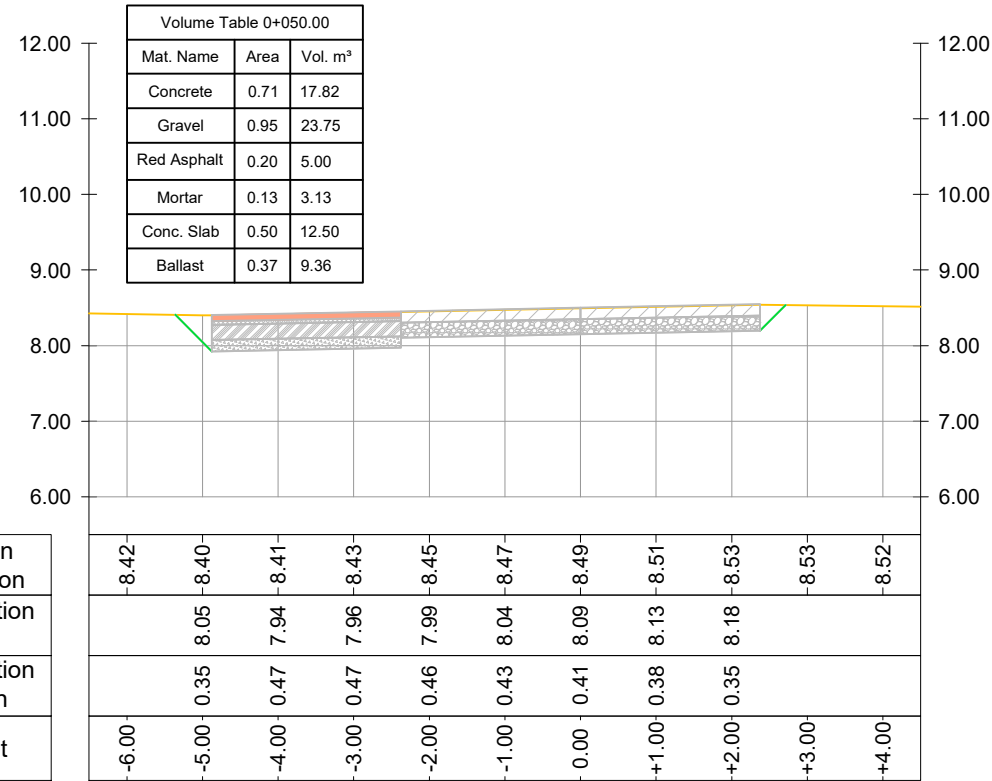
CROSS SECTION Road Nr. 8 - Recreational Park - Prog.: 0+050.00
