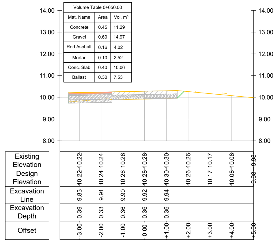
CROSS SECTION Road Nr. 7 - Recreational Park - Prog.: 0+650.00
