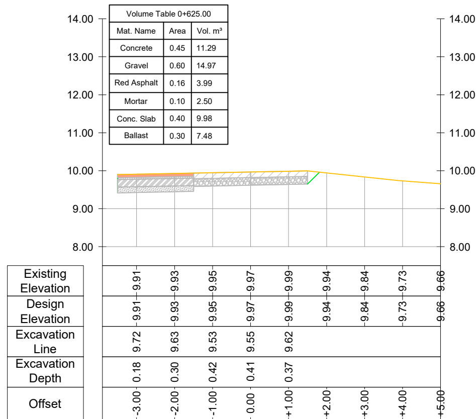
CROSS SECTION Road Nr. 7 - Recreational Park - Prog.: 0+625.00
