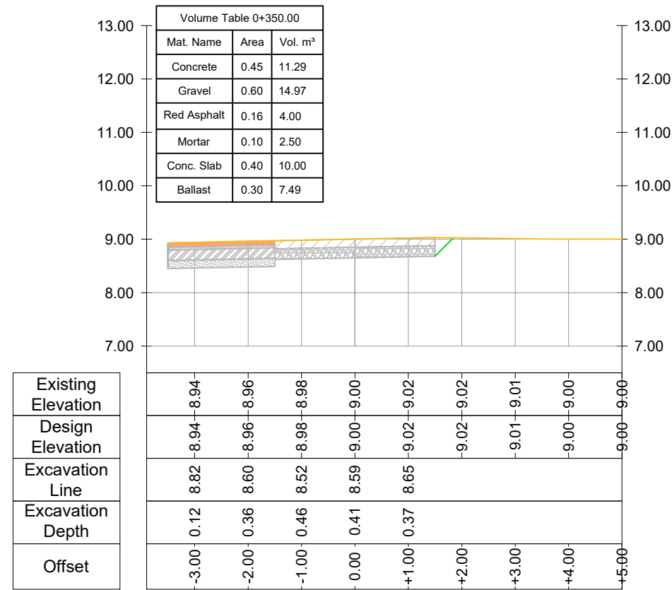
CROSS SECTION Road Nr. 7 - Recreational Park - Prog.: 0+350.00
