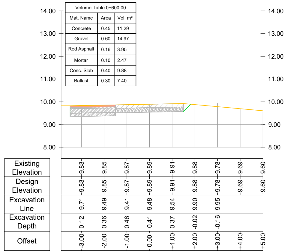
CROSS SECTION Road Nr. 7 - Recreational Park - Prog.: 0+600.00
