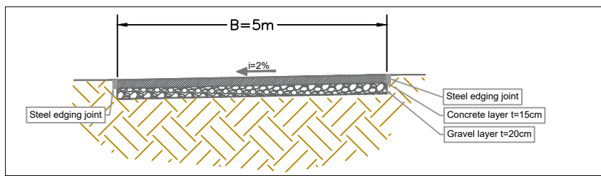
TYPICAL SECTION Prog. 0+000.00 - 0+139.90 SCALE 1:100
