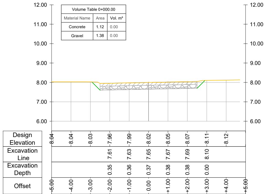
CROSS SECTION Road Nr.11-Recreational Park - Prog.: 0+000.00
