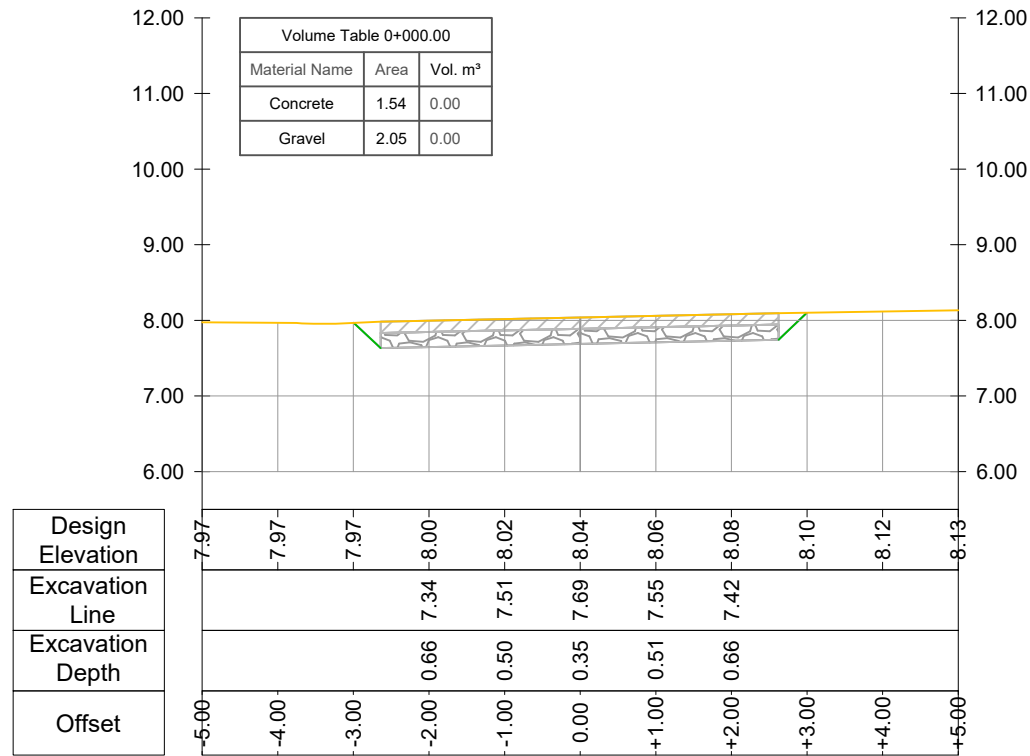
CROSS SECTION Road Nr.13-Recreational Park - Prog.: 0+000.00
