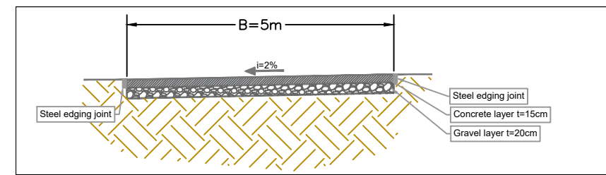
TYPICAL SECTION Prog. 0+000.00 - 0+100.20 SCALE 1:100
