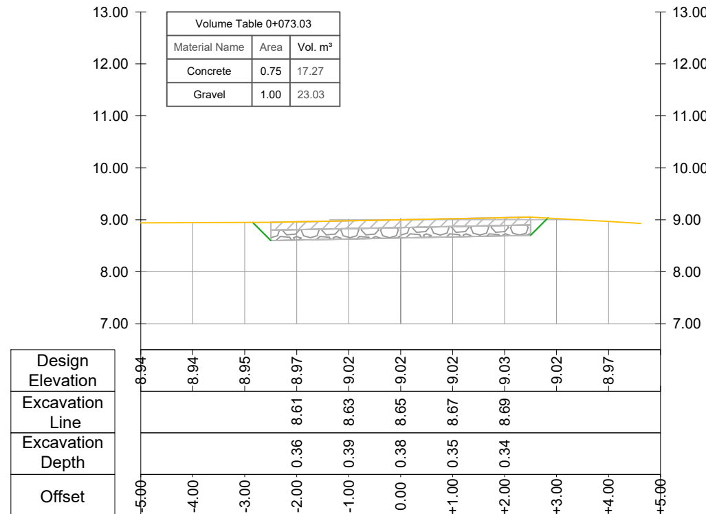
CROSS SECTION Road Nr.10-Recreational Park - Prog.: 0+073.03
