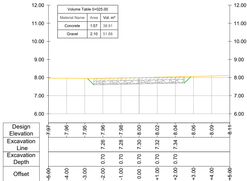
CROSS SECTION Road Nr.13-Recreational Park - Prog.: 0+025.00
