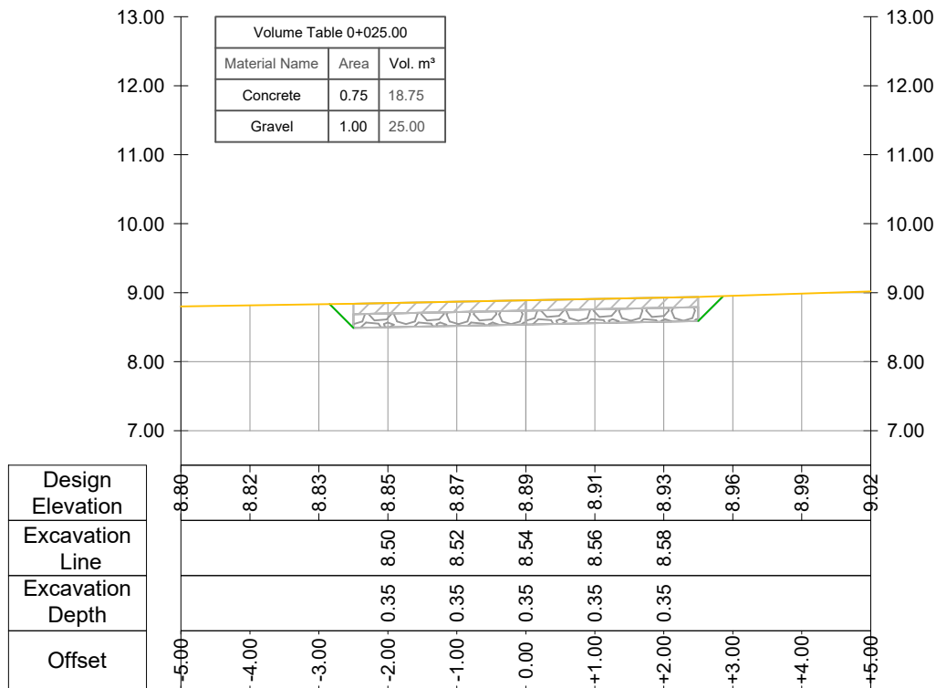
CROSS SECTION Road Nr.12-Recreational Park - Prog.: 0+025.00
