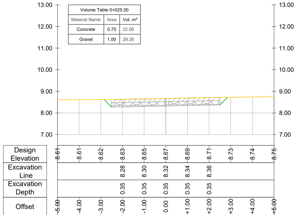
CROSS SECTION Road Nr.10-Recreational Park - Prog.: 0+025.00
