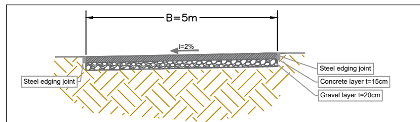
TYPICAL SECTION Prog. 0+000.00 - 0+112.90 SCALE 1:100
