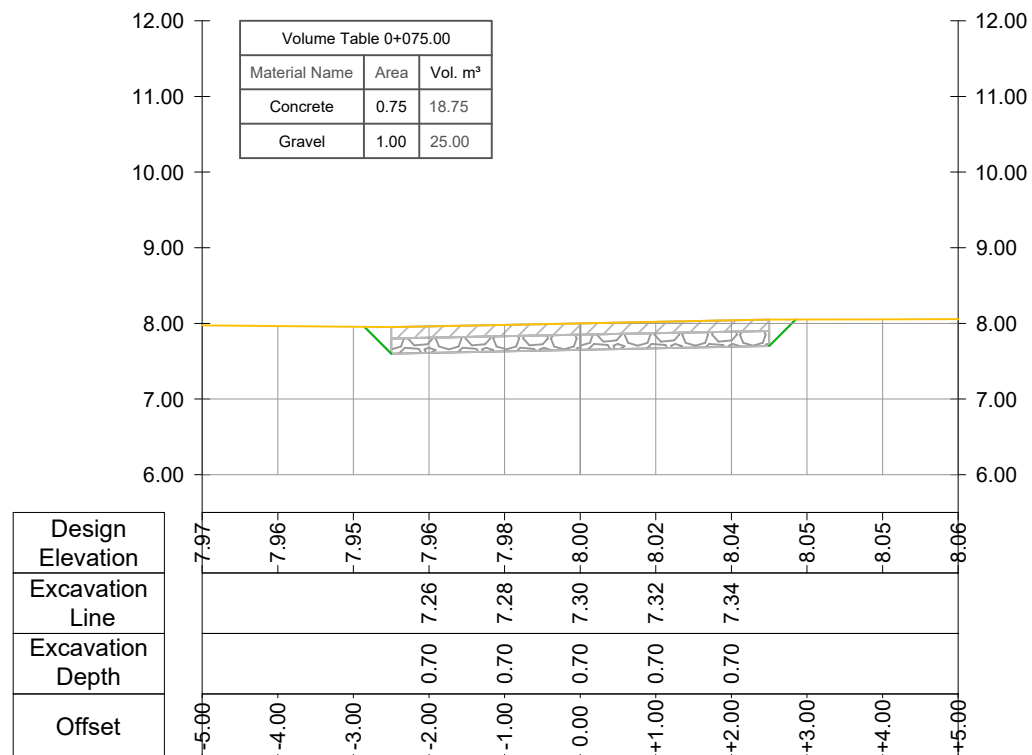
CROSS SECTION Road Nr.13-Recreational Park - Prog.: 0+075.00
