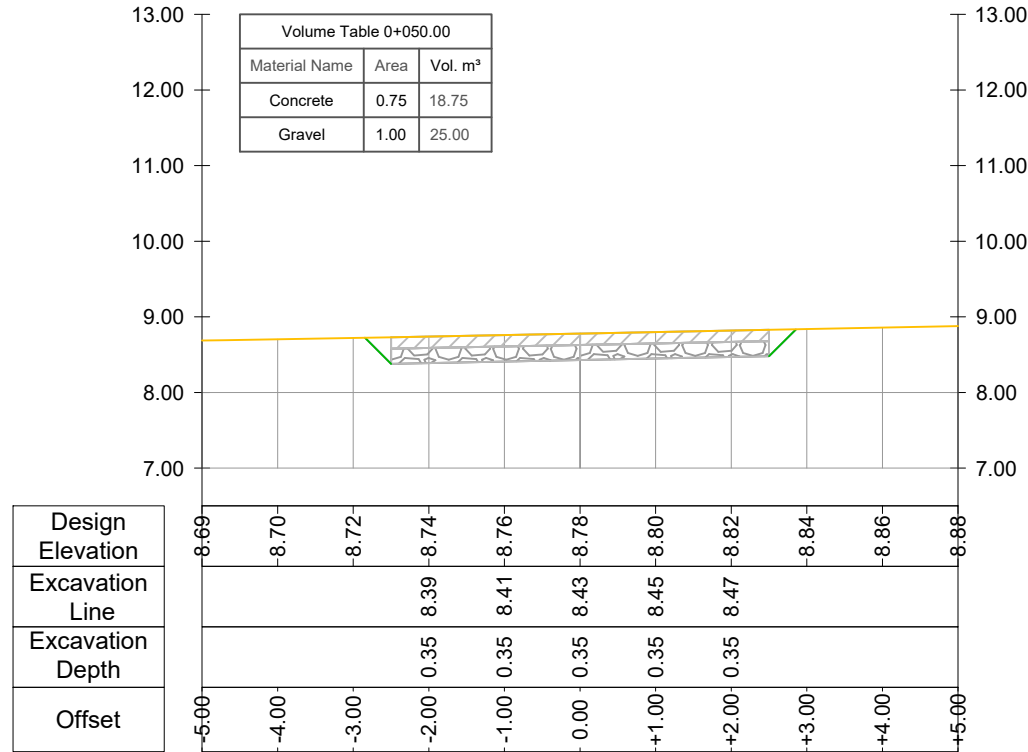
CROSS SECTION Road Nr.12-Recreational Park - Prog.: 0+050.00
