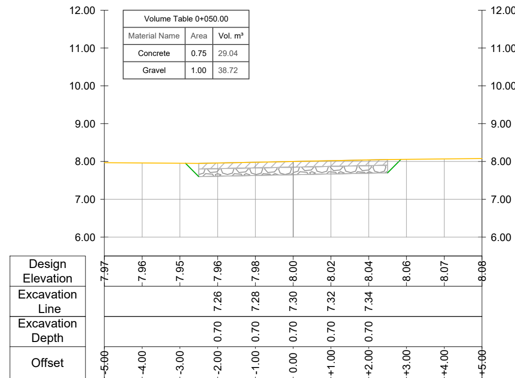
CROSS SECTION Road Nr.13-Recreational Park - Prog.: 0+050.00
