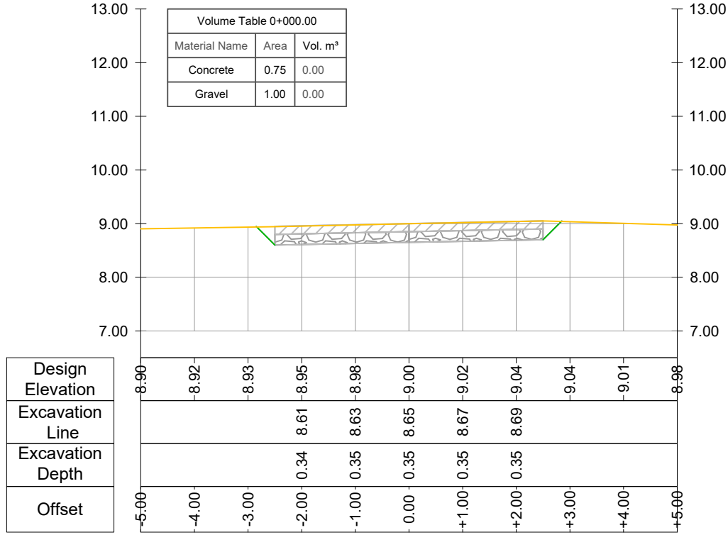
CROSS SECTION Road Nr.12-Recreational Park - Prog.: 0+000.00
