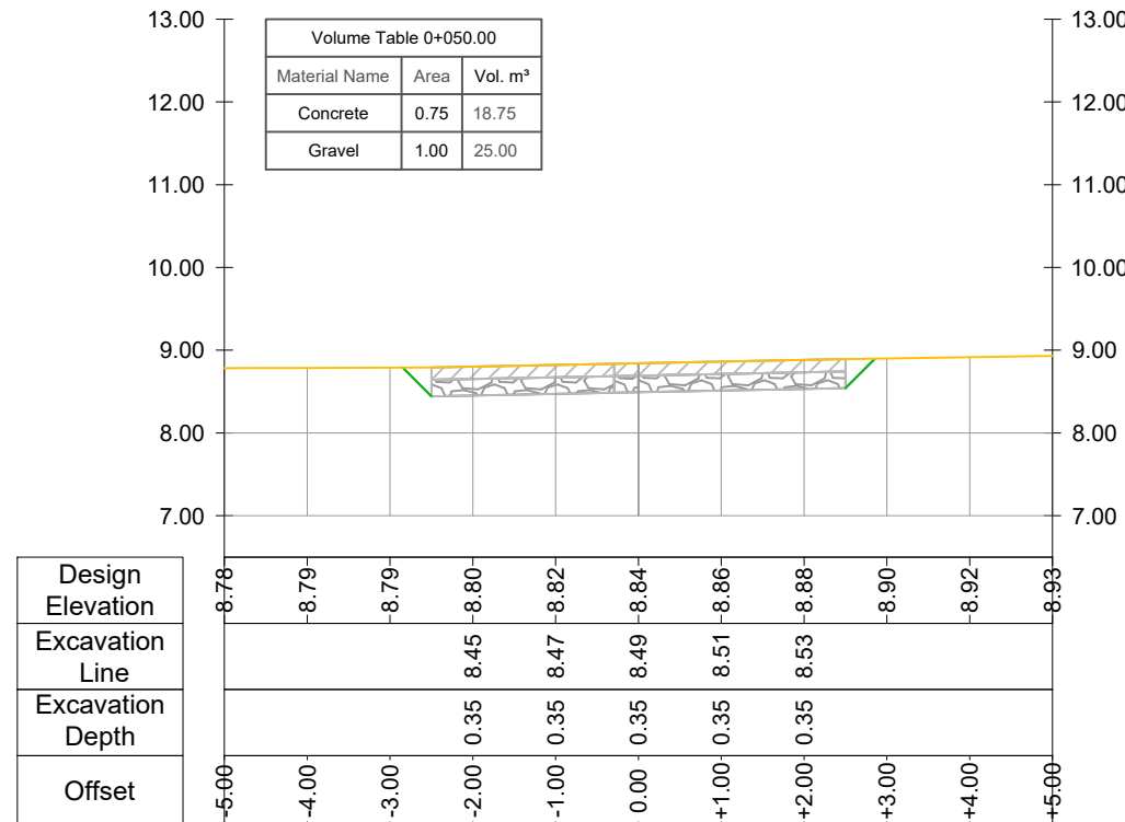
CROSS SECTION Road Nr.10-Recreational Park - Prog.: 0+050.00
