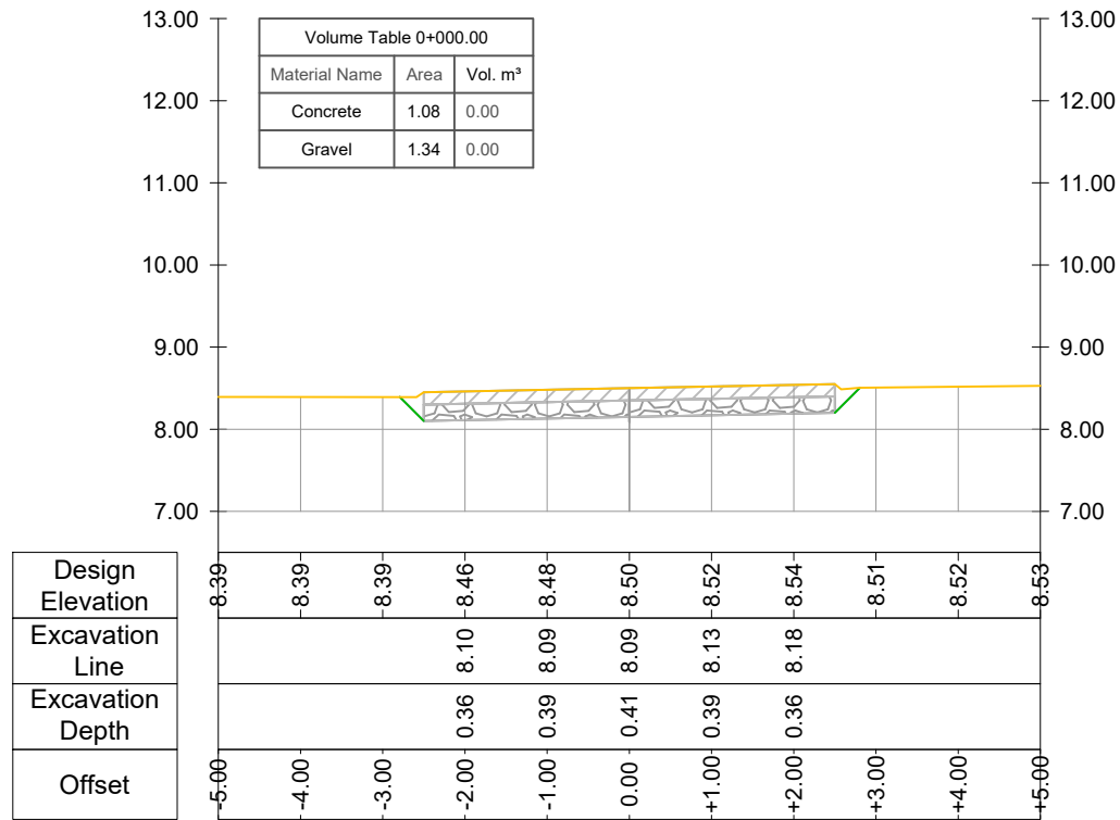
CROSS SECTION Road Nr.10-Recreational Park - Prog.: 0+000.00
