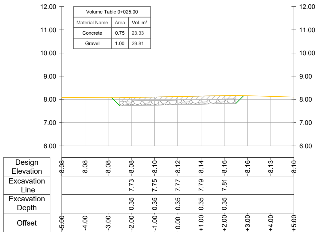
CROSS SECTION Road Nr.11-Recreational Park - Prog.: 0+025.00
