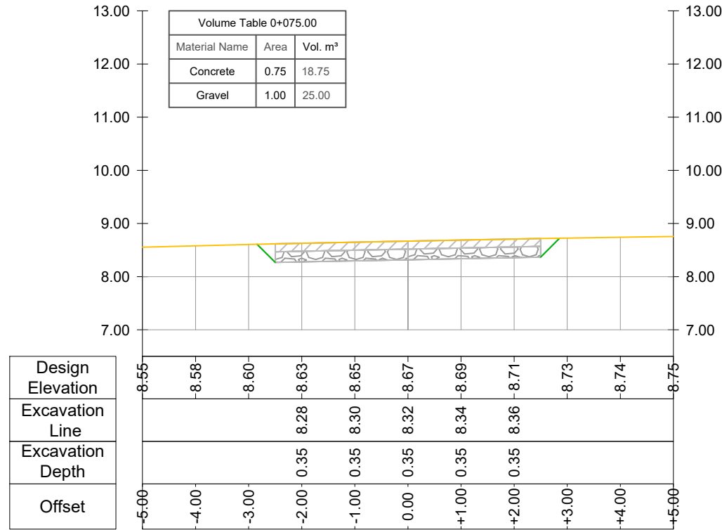
CROSS SECTION Road Nr.12-Recreational Park - Prog.: 0+075.00
