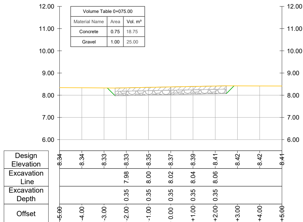
CROSS SECTION Road Nr.11-Recreational Park - Prog.: 0+075.00
