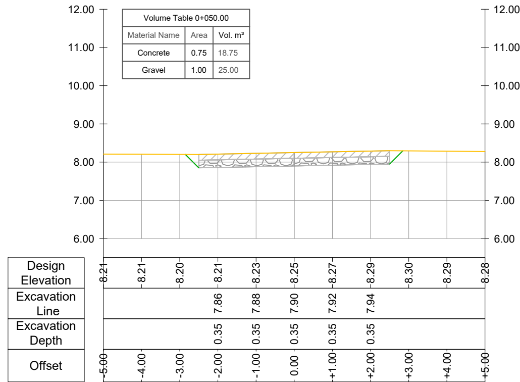
CROSS SECTION Road Nr.11-Recreational Park - Prog.: 0+050.00
