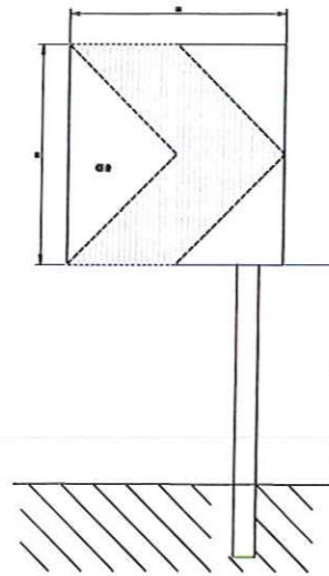
Chevron sign Kthese e menjehershme
