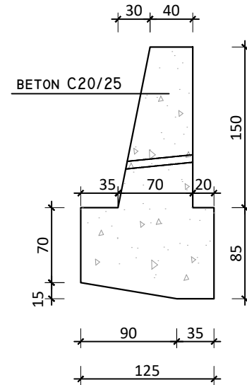
Mur prites C20/25 h=1.5m Sh 1:50
