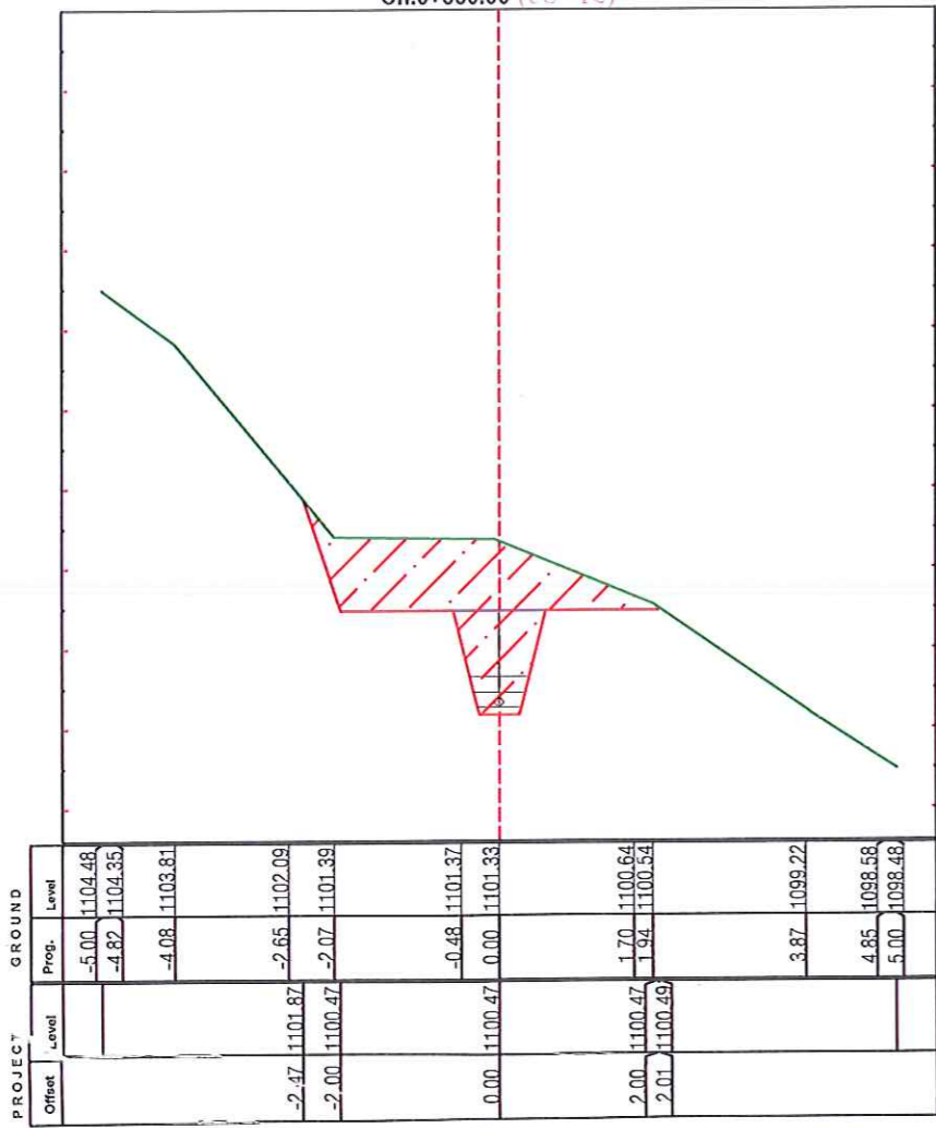
Ch.0+550.00 (CS-12)
