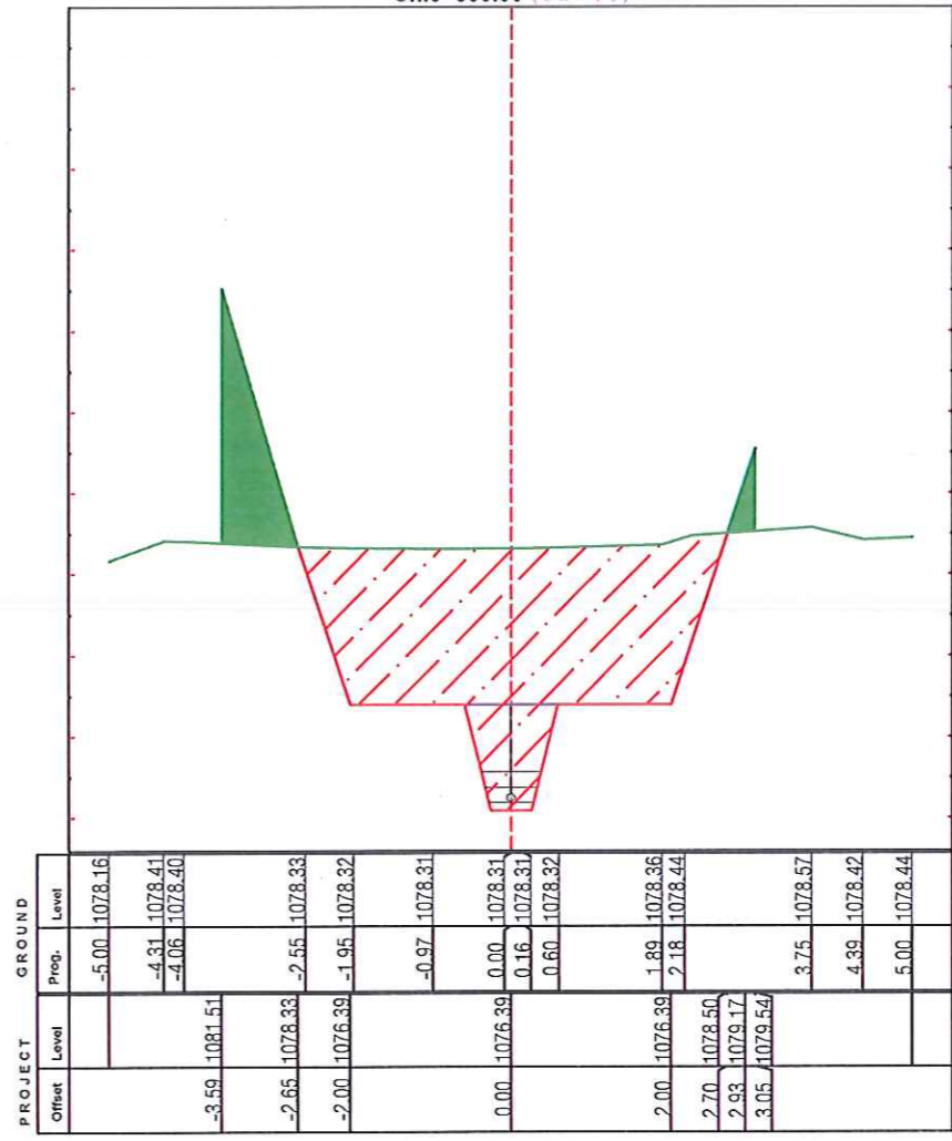
Ch.0+500.00 (CS-11)
