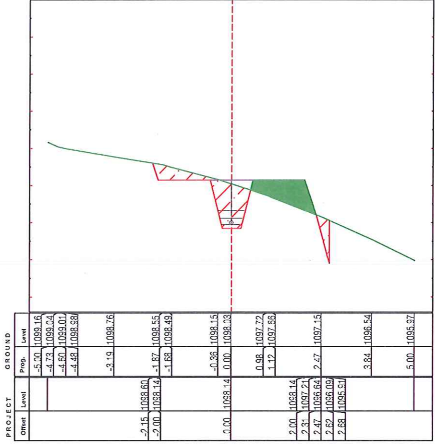
Ch.1+100.00 (CS-23)
