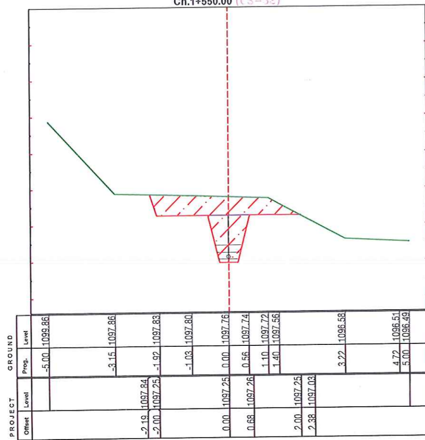
Ch.1+550.00 (CS-32)
