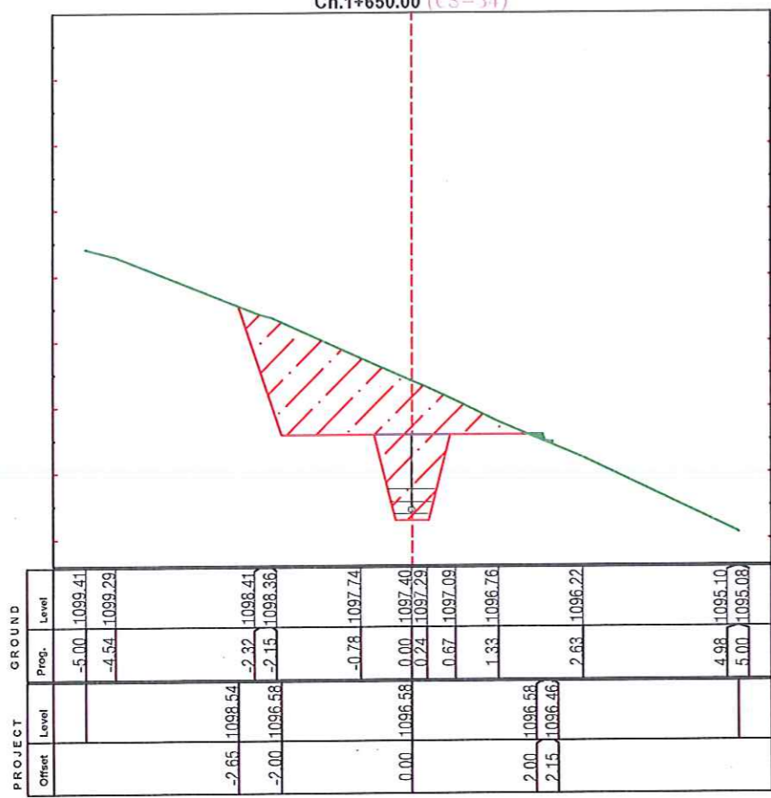
Ch.1+650.00 (CS-31)
