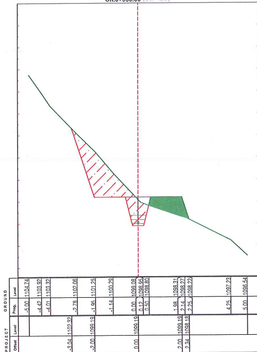
Ch.0+950.00 (CS-20)
