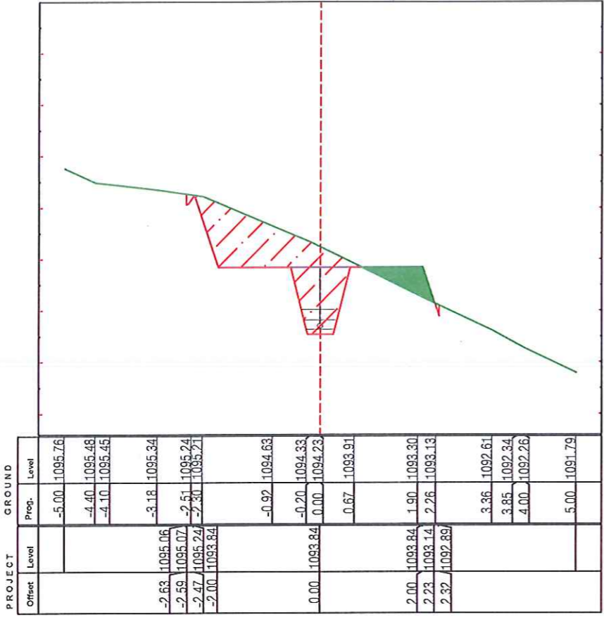
Ch.1+150.00 (CS-24)
