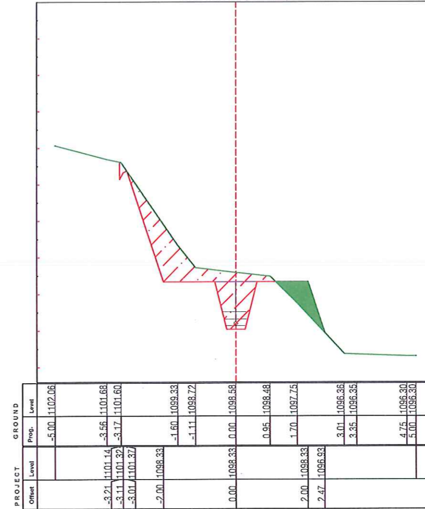
Ch.1+300.00 (CS-27)
