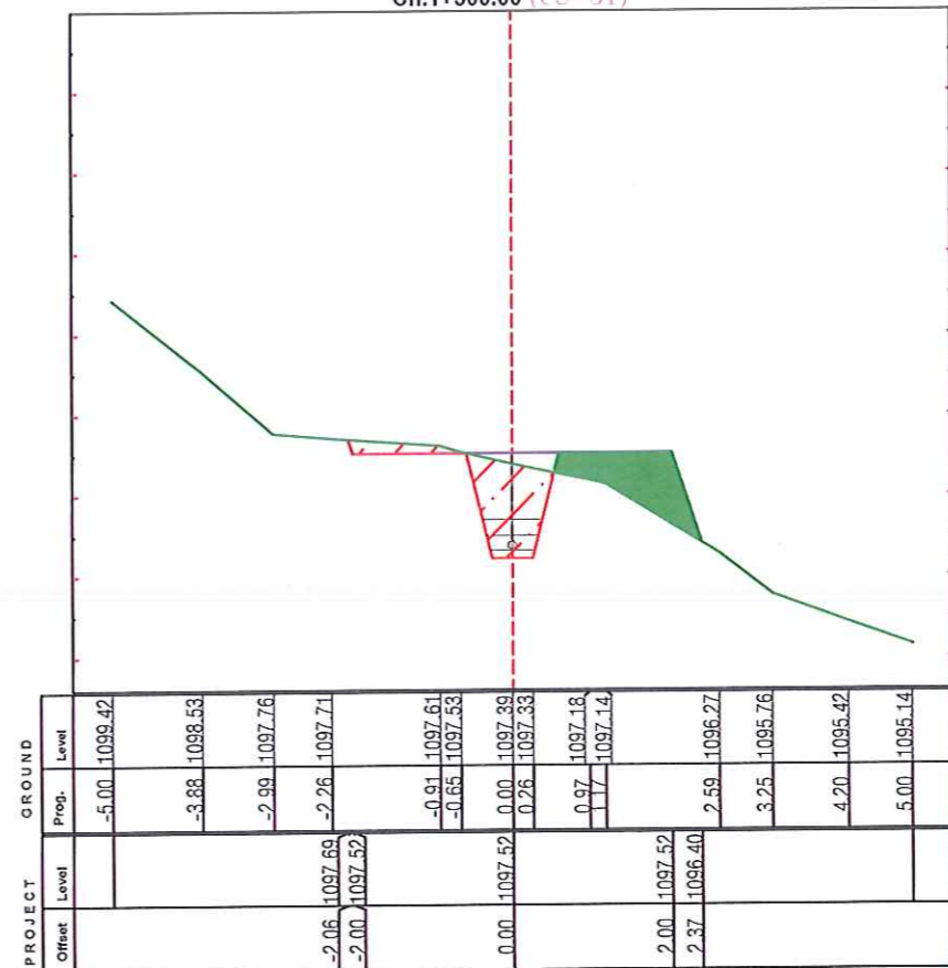
Ch.1+500.00 (CS-31)
