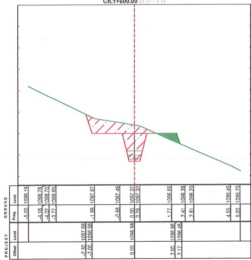
Ch.1+600.00 (CS-33)
