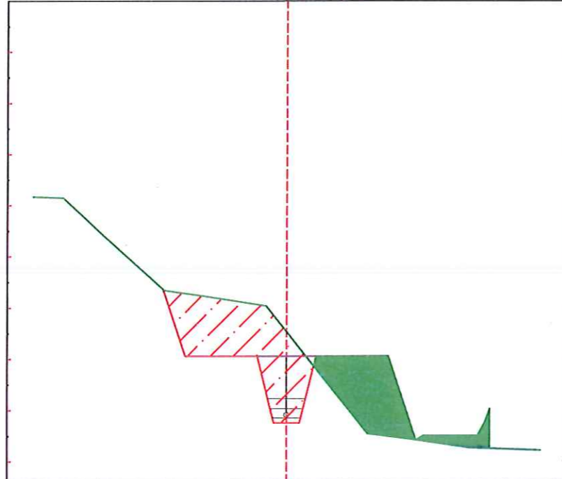
Ch.0+650.00 (CS-14)
