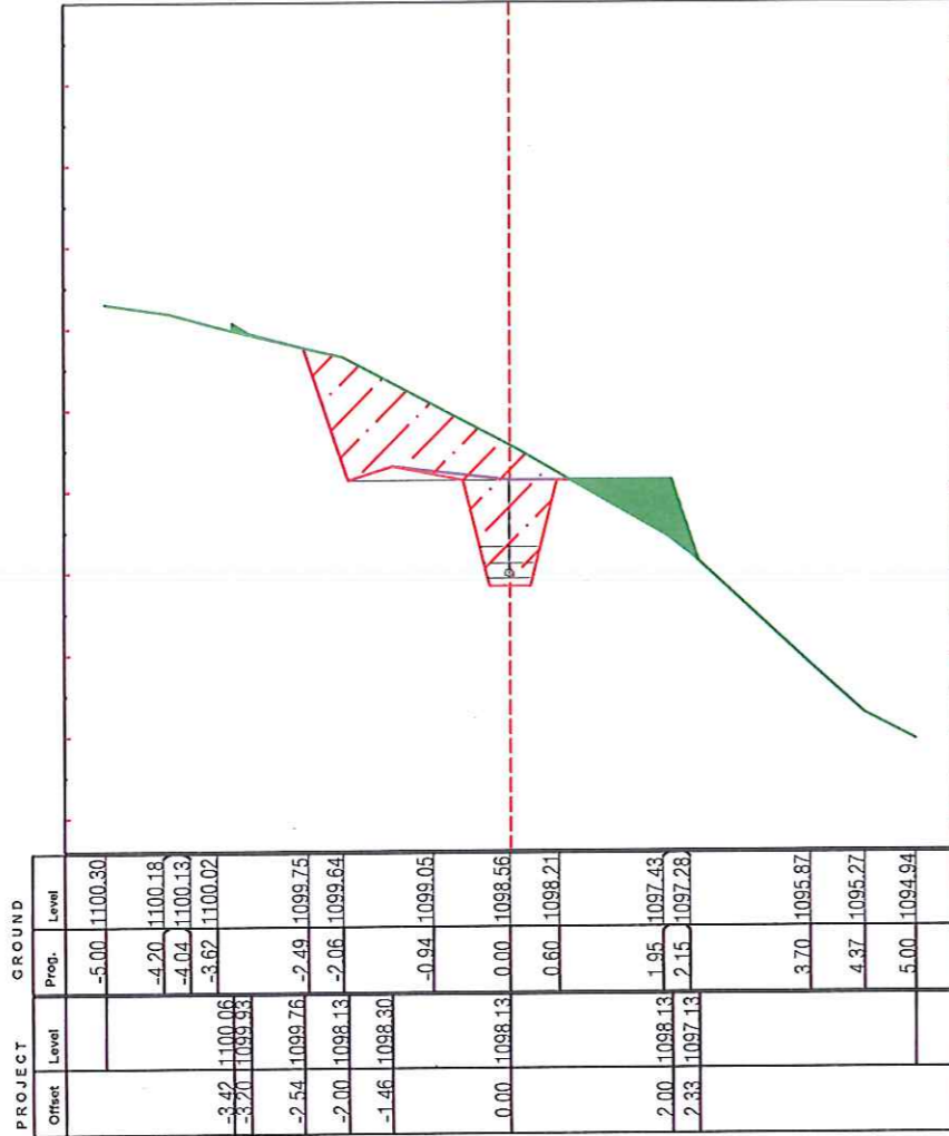
Ch.1+350.00 (CS-28)
