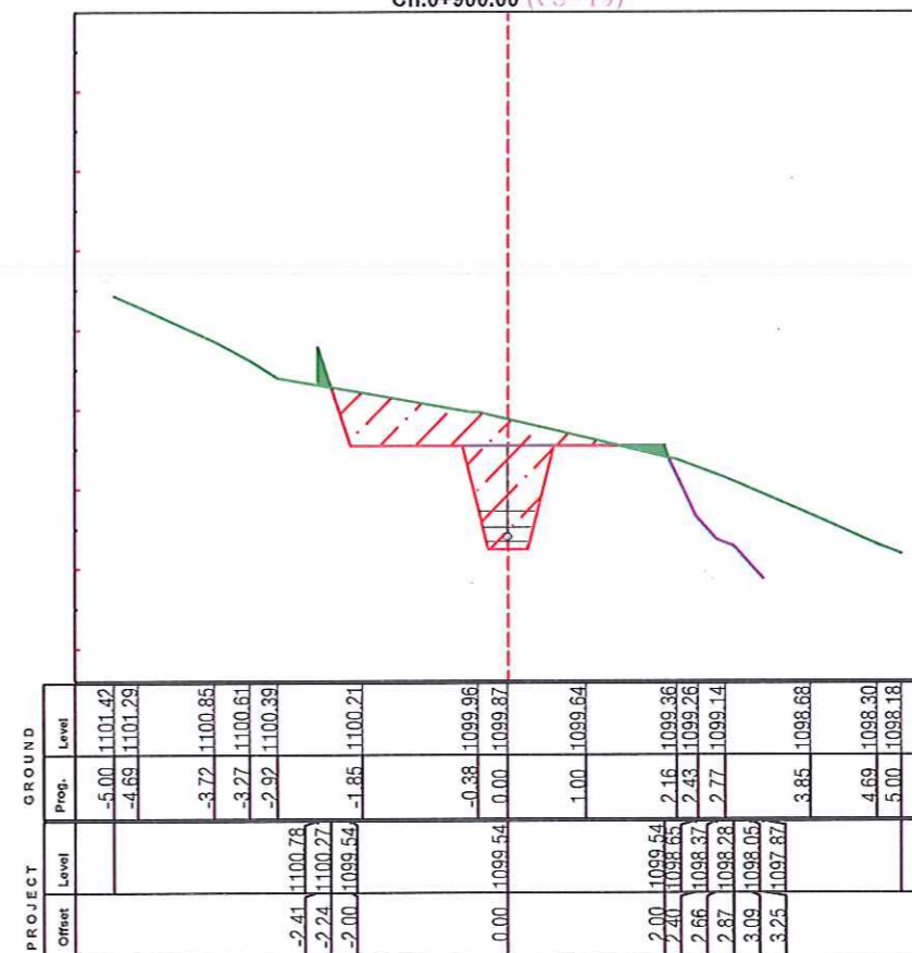
Ch.0+900.00 (CS-19)
