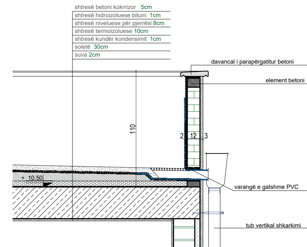
D7: SHITESAT E TARRACËS / sh. 1:15
