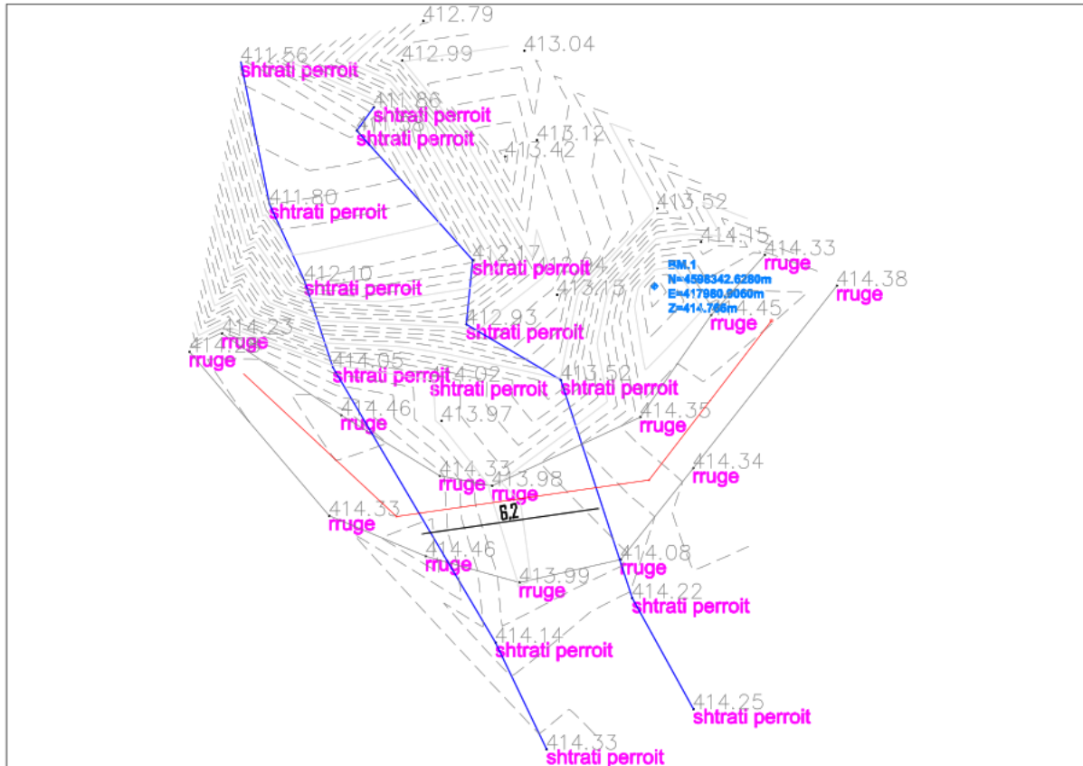
Figura 5: Plani I Rilevimit
