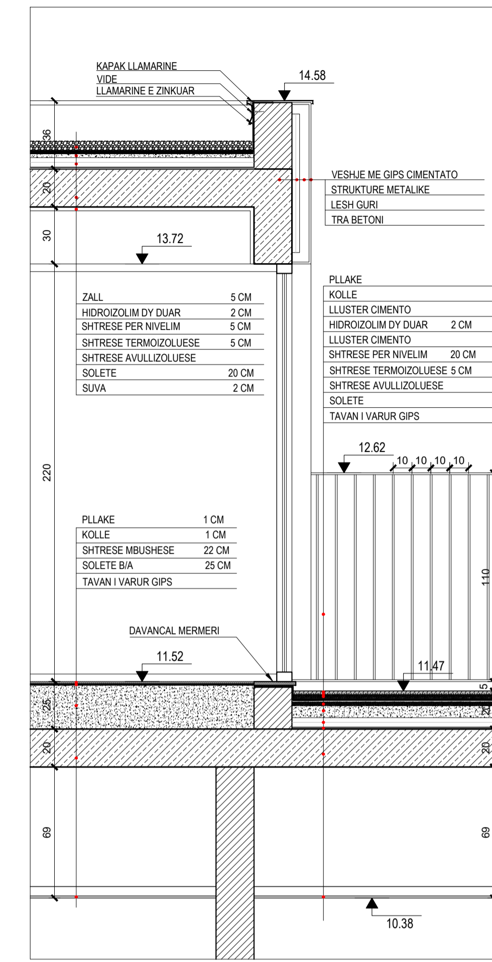
DETAJI 13 SH 1:20
