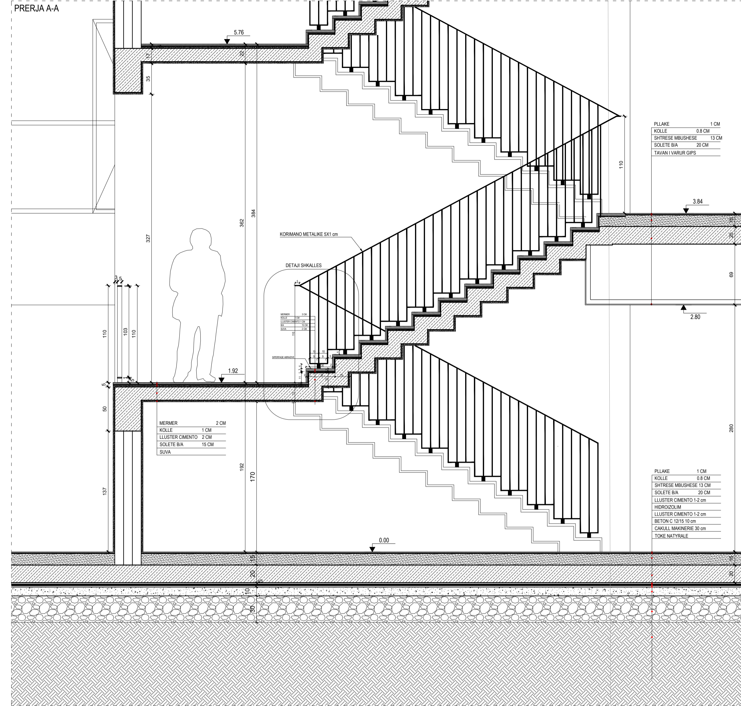
DETAJI 10 SH 1:25
