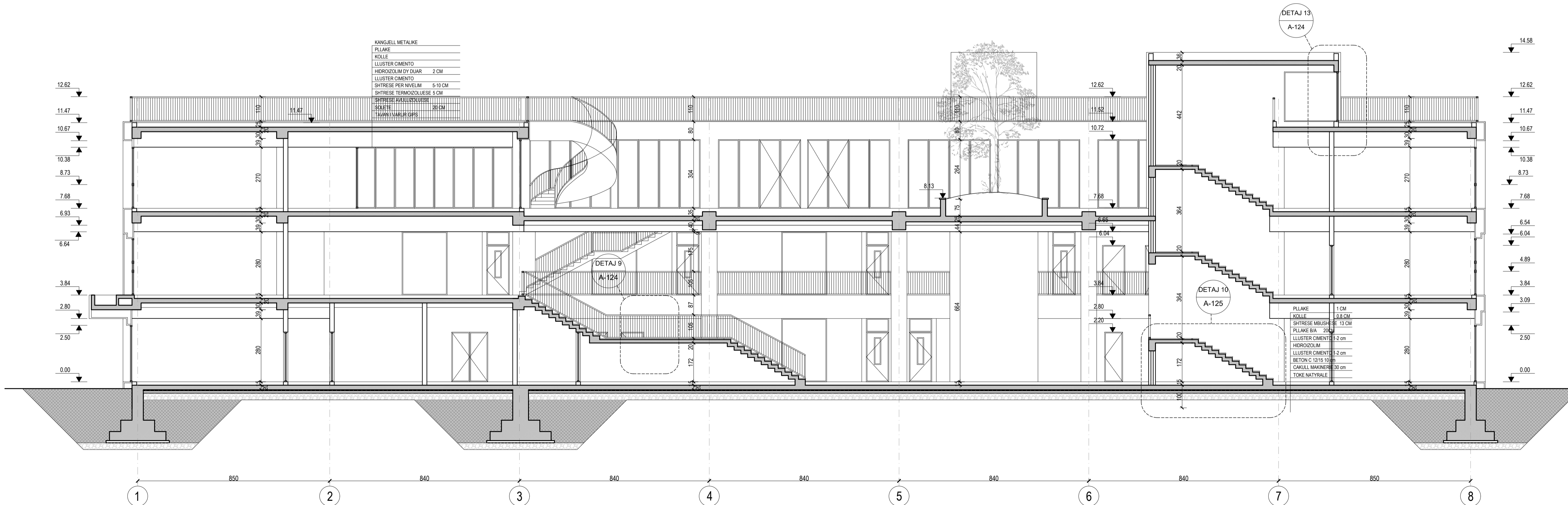
PRERJA 2-2 SH. 1:100
