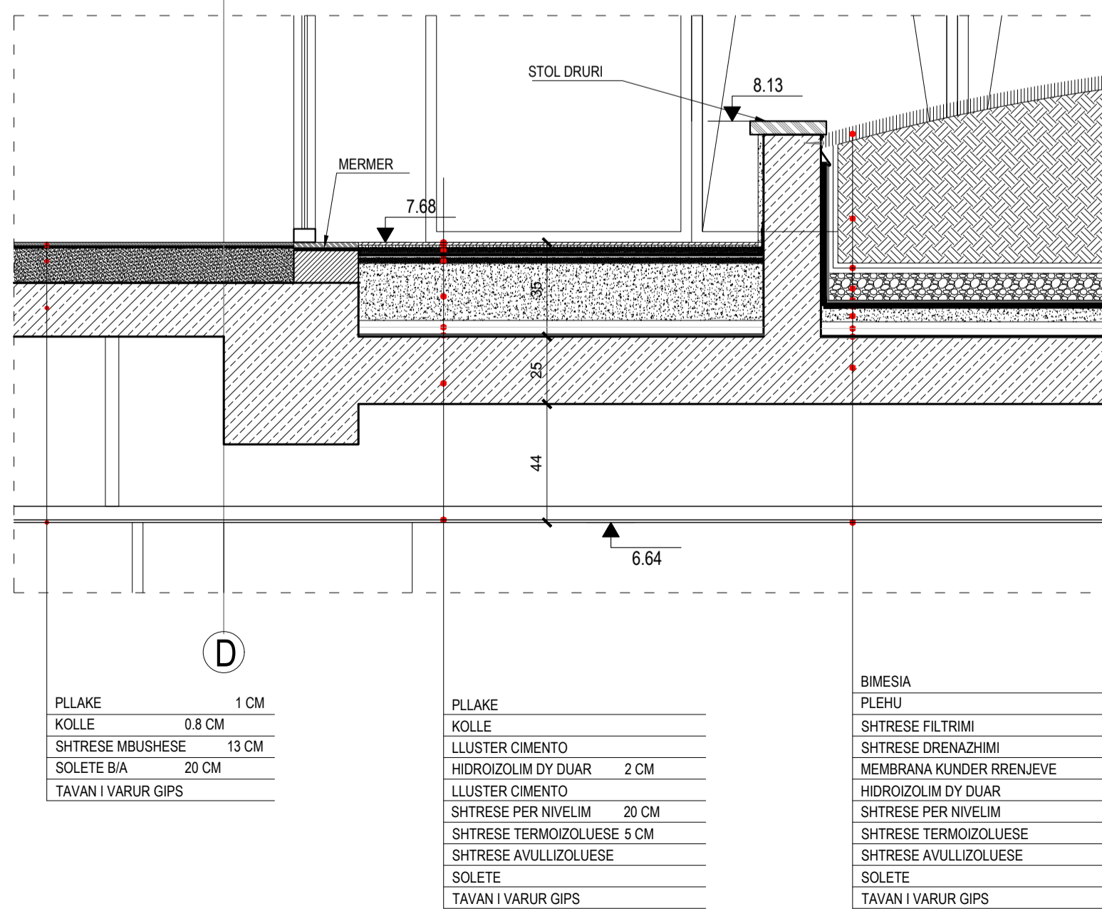
DETAJI 12 SH 1:20
