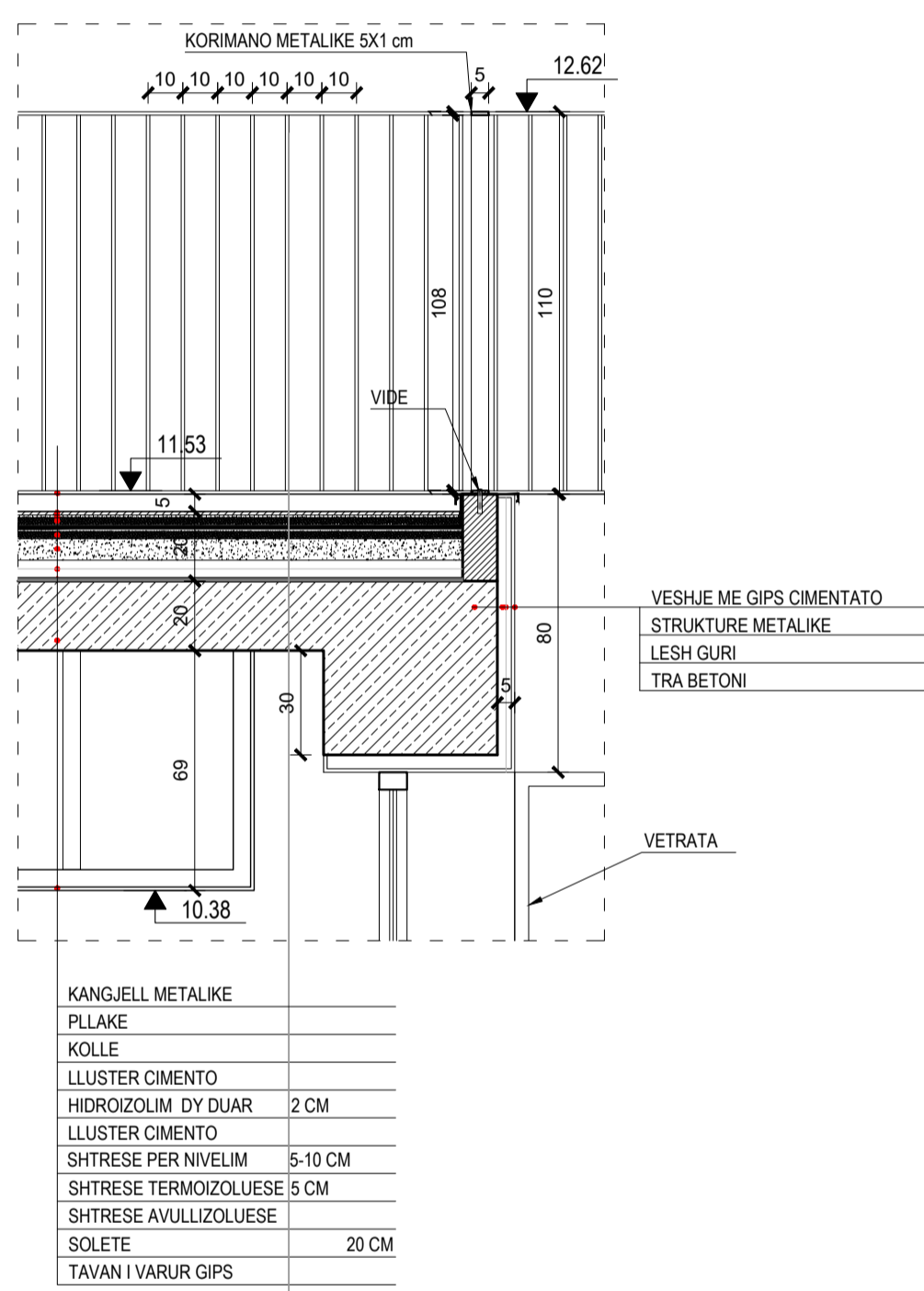
DETAJI 11 SH 1:20
