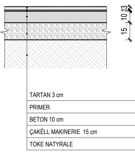
DETAJ 1 SH 1/20 SHITESAT E FUSHAVE
