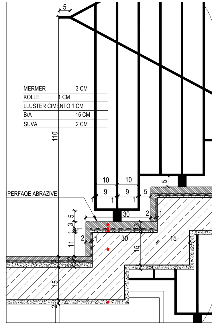
DETAJI SHKALLES SH 1:10
