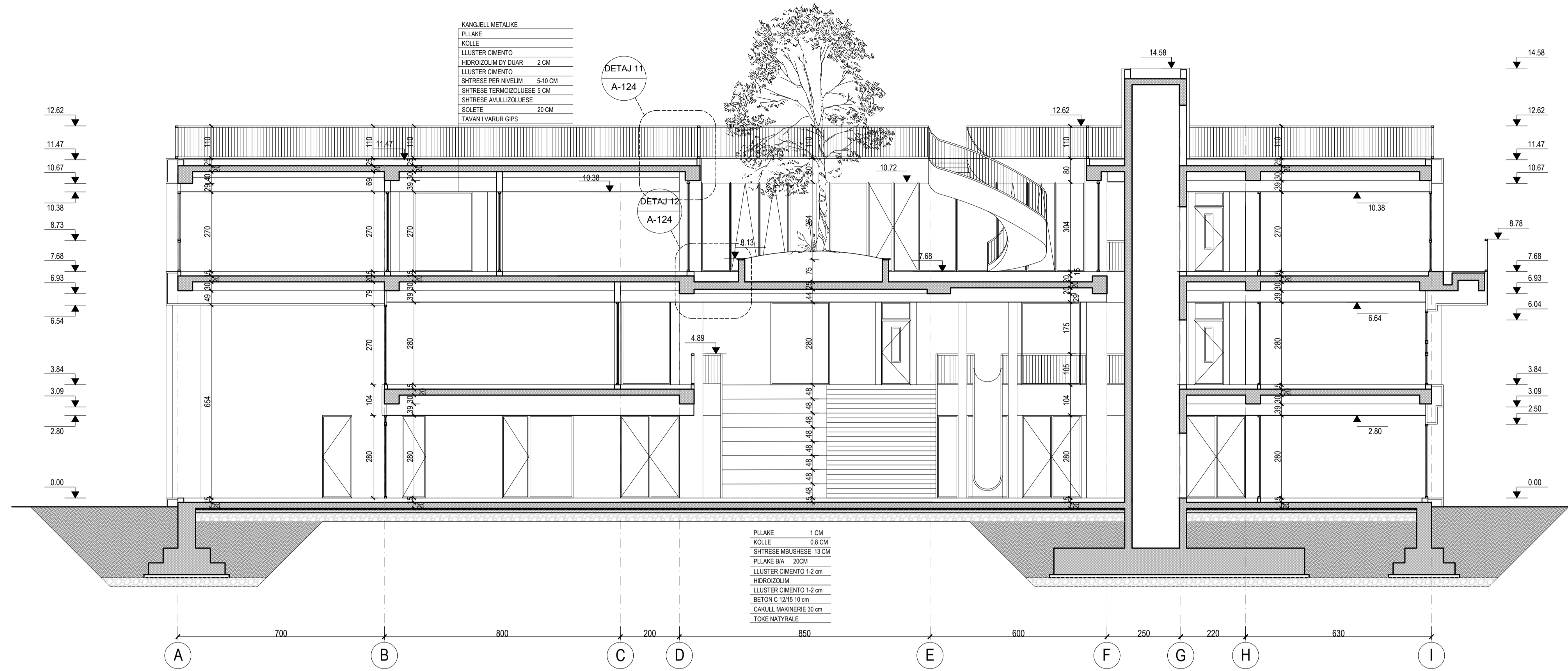
PRERJA C-C SH. 1:100
