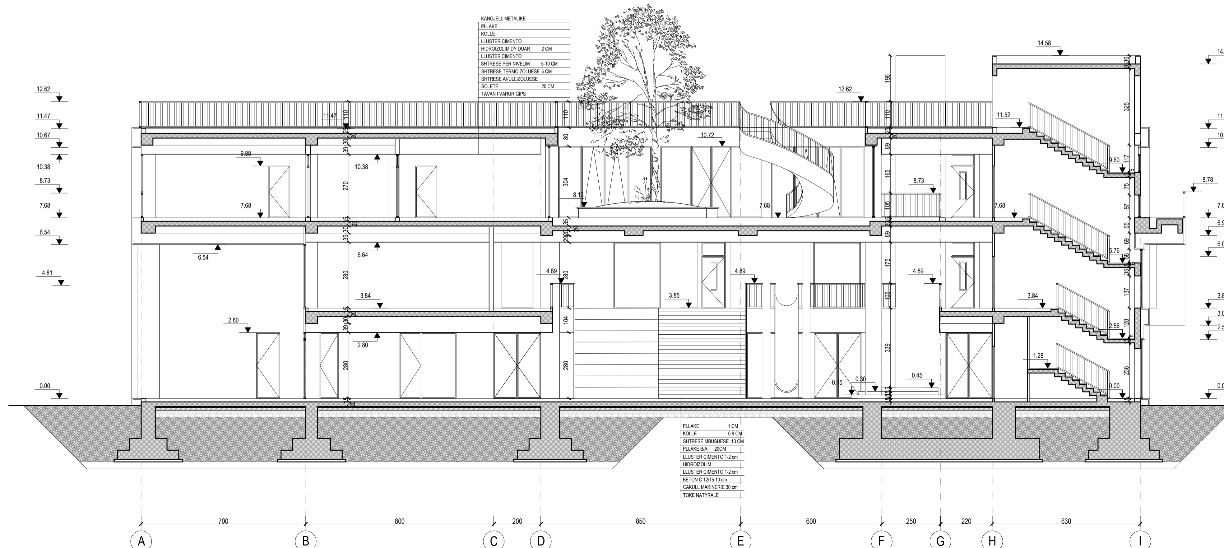
PRERJA D-D SH. 1:100
