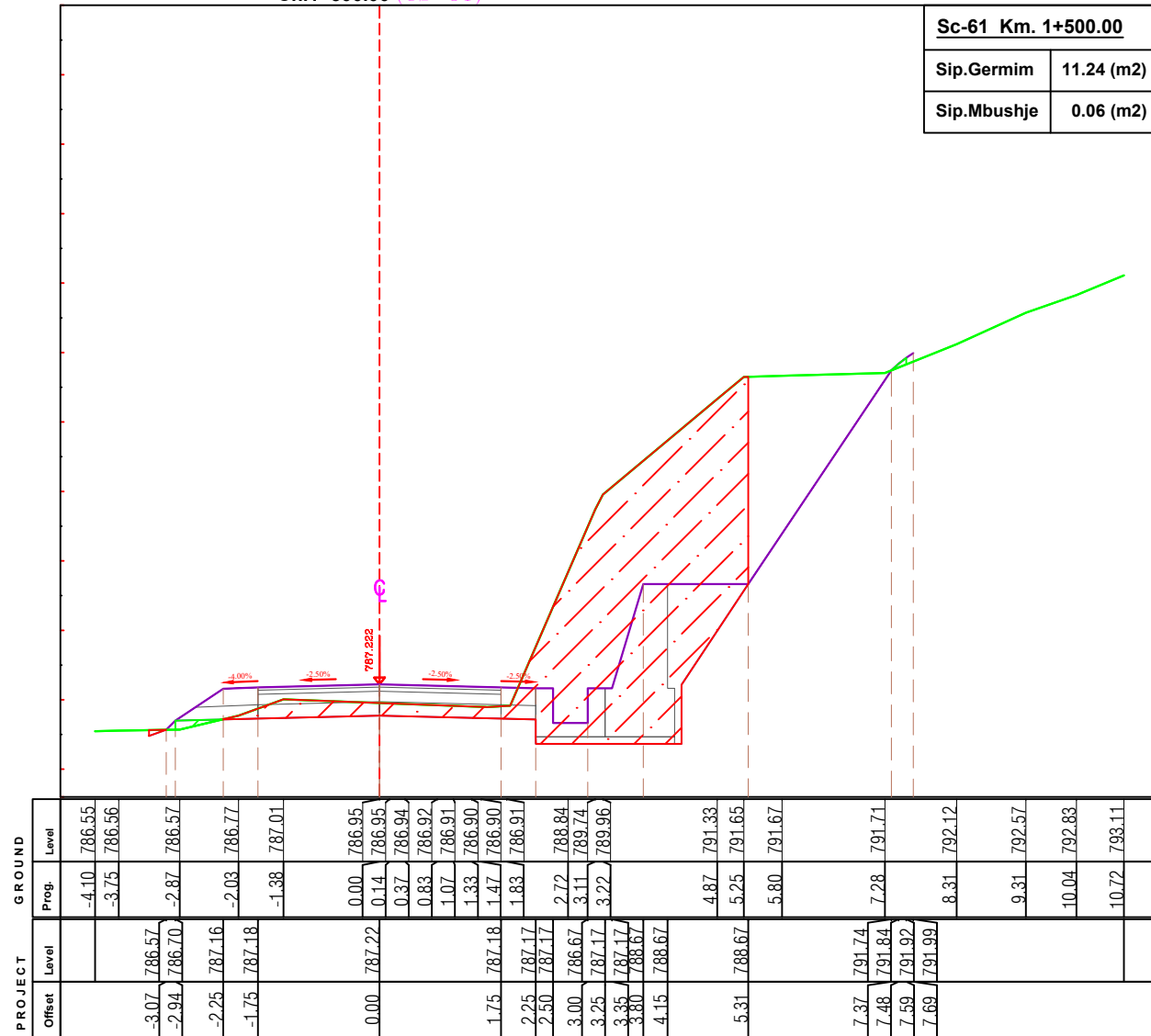
Ch.1+500.00 (CS-61)
