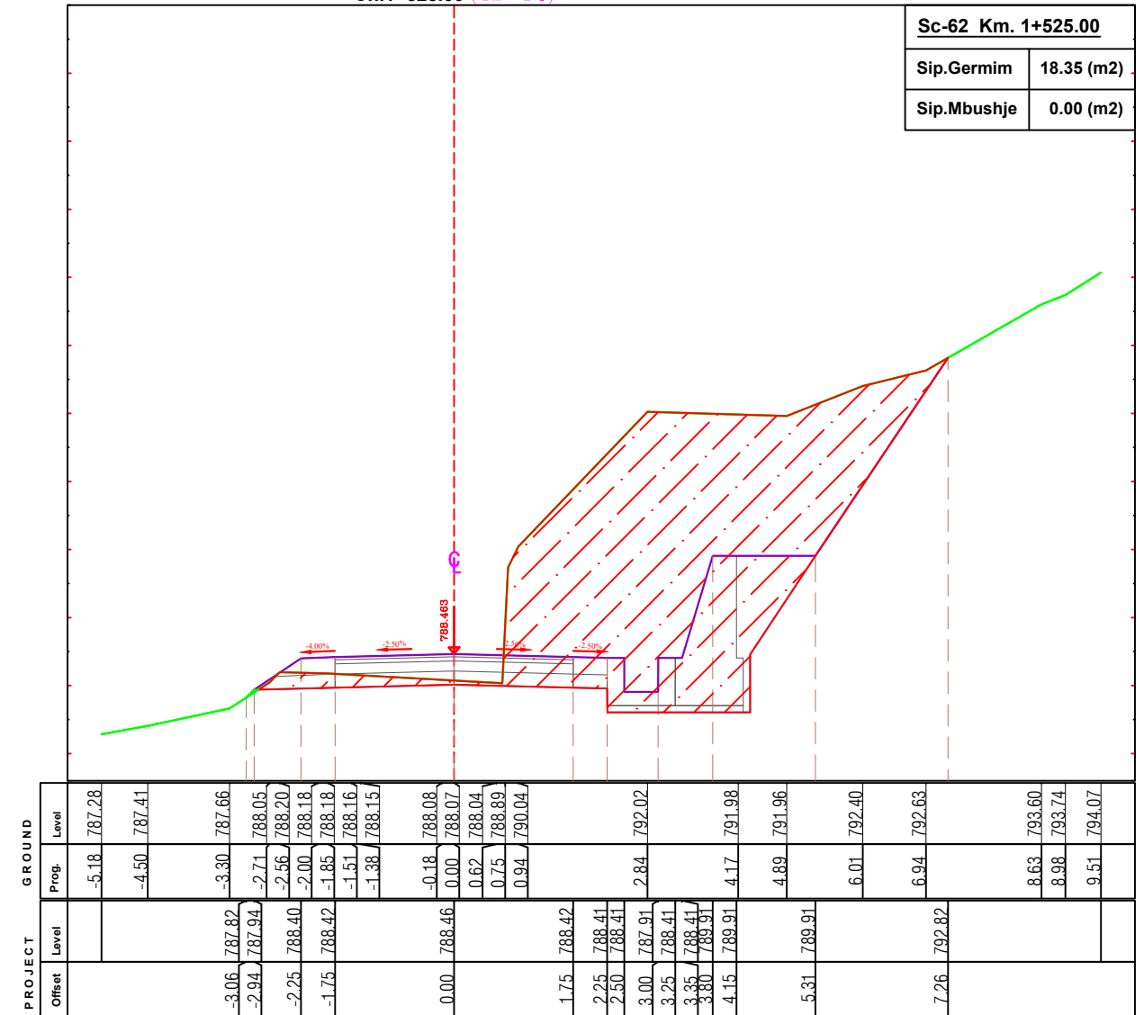
Ch.1+525.00 (CS-62)
