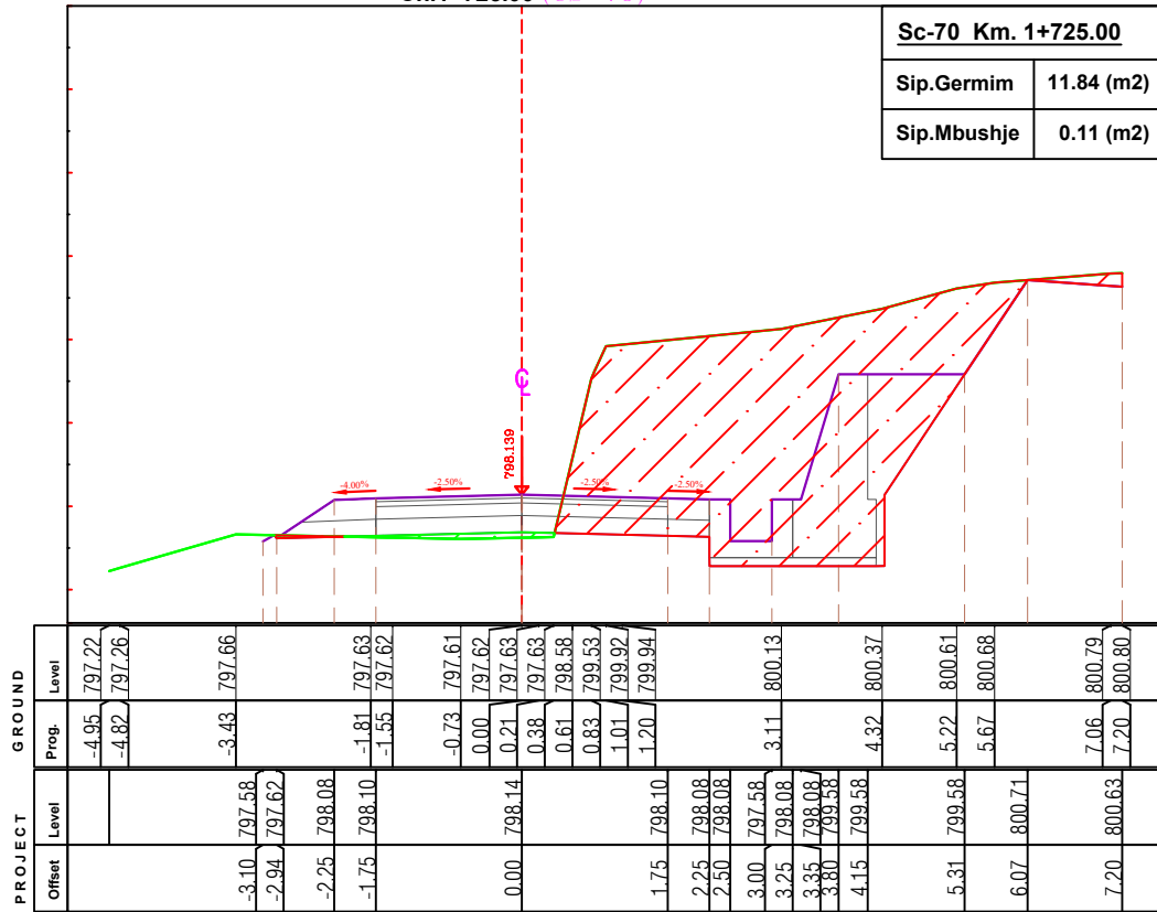
Ch.1+725.00 (CS-70)
