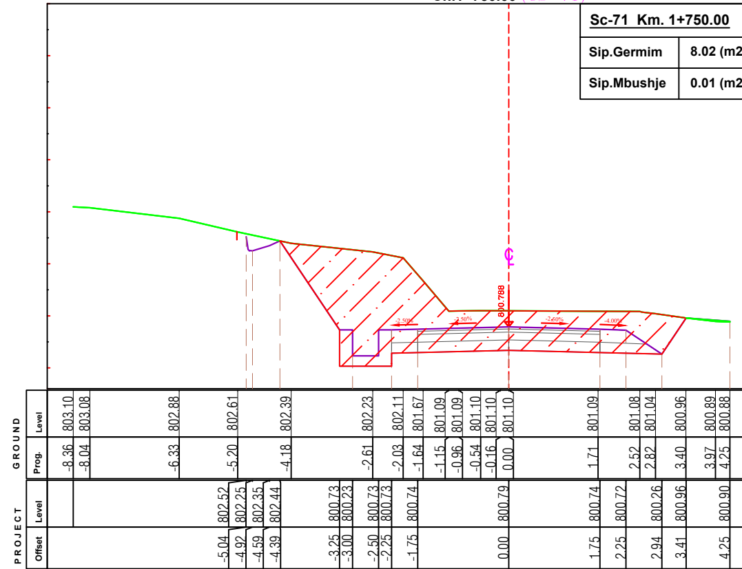
Ch.1+750.00 (CS-71)
