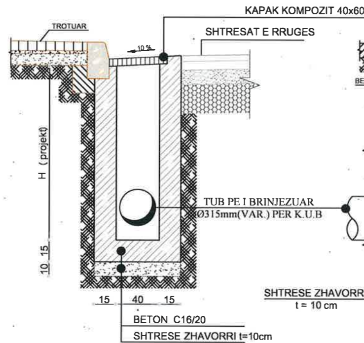
PRERJE B-B (PER TUBA HDPE D=315MM) SH- 1:25
