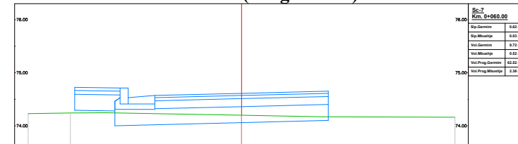
Km.0+060.00 (Progresivi-7)
