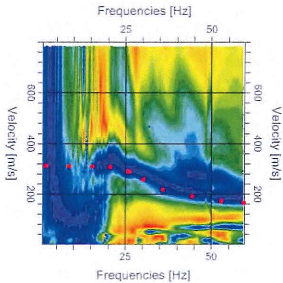
Phase velocity - frequency spectrum
