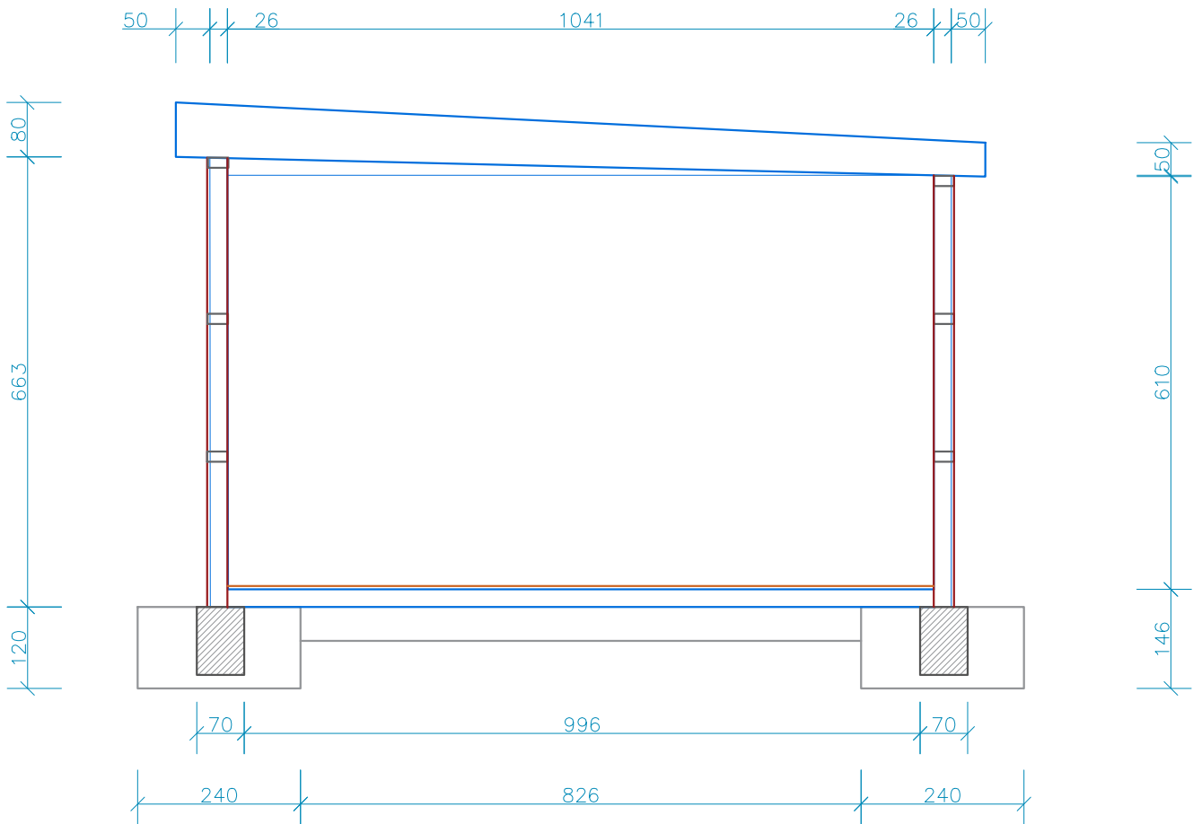
PALESTRA - PRERJE TERTHORE MURE TULLE, SH-1:100
