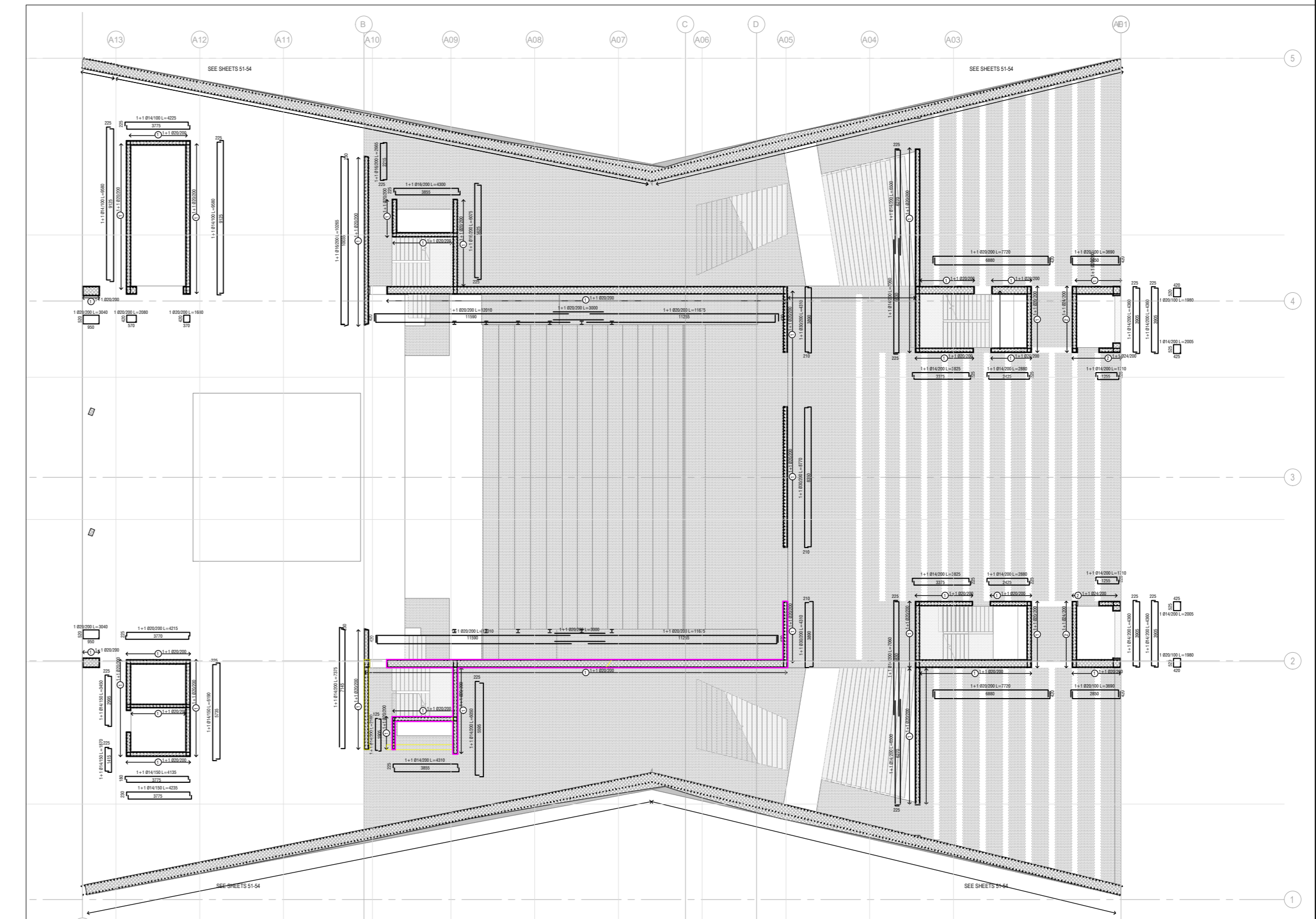
PLANI REFERUES SH 1:200
