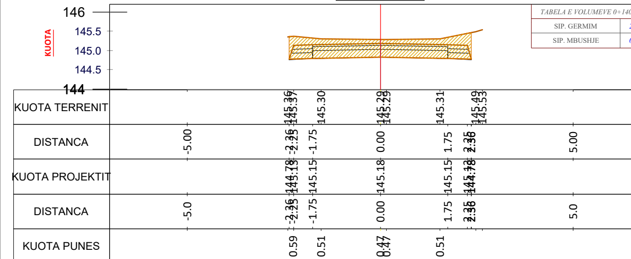
CS - 8 PROG - 0+140.0
