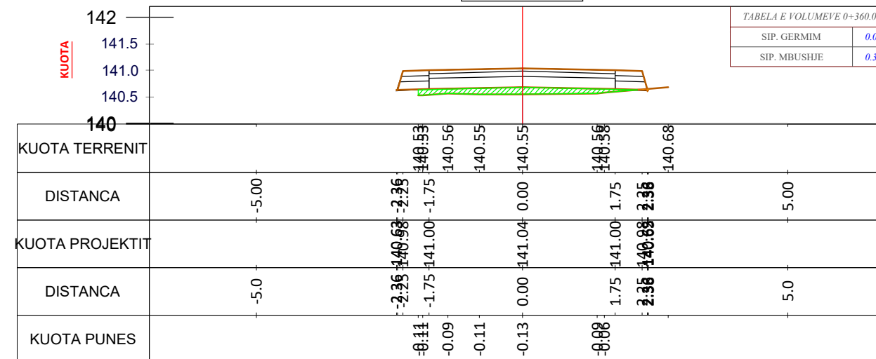
CS - 19 PROG - 0+360.0
