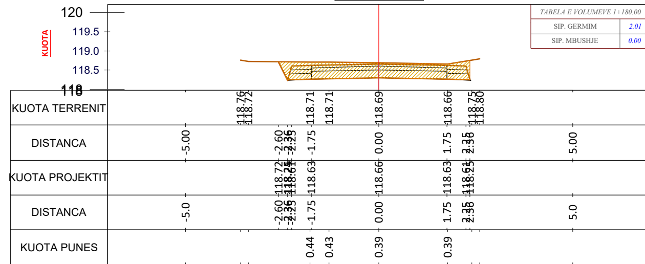
CS - 60 PROG - 1+180.0
