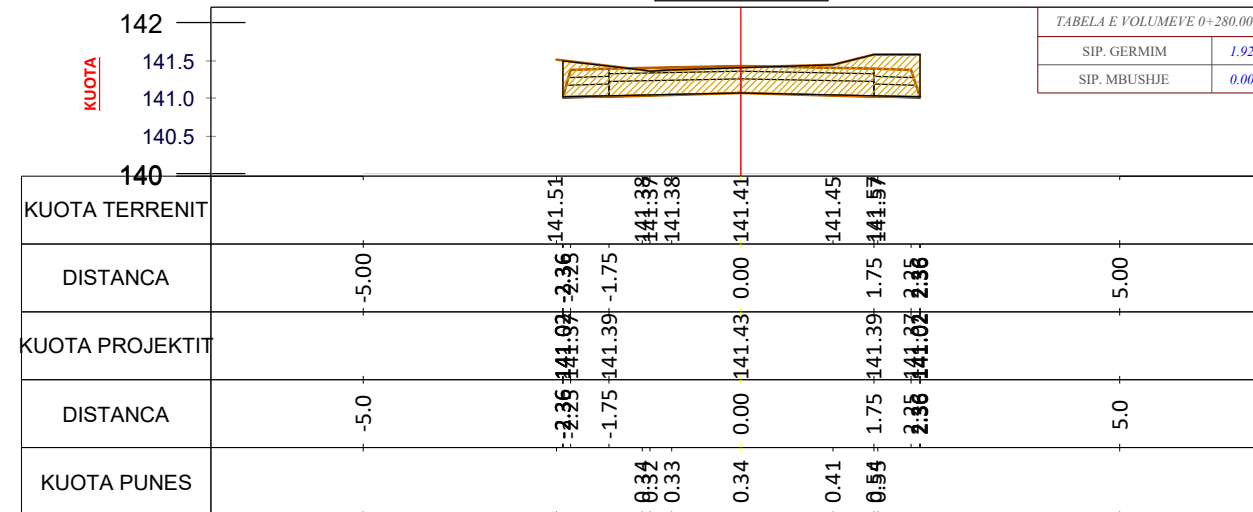
CS - 15 PROG - 0+280.0
