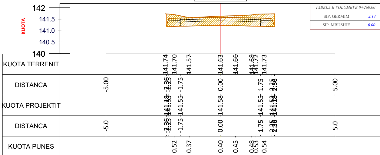
CS - 14 PROG - 0+260.0
