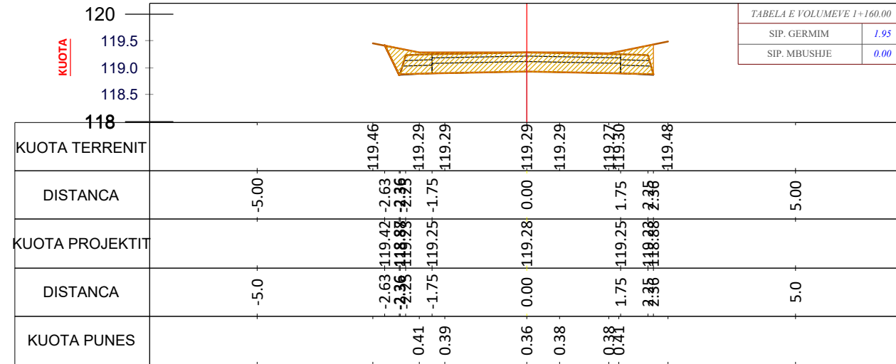
CS - 59 PROG - 1+160.0
