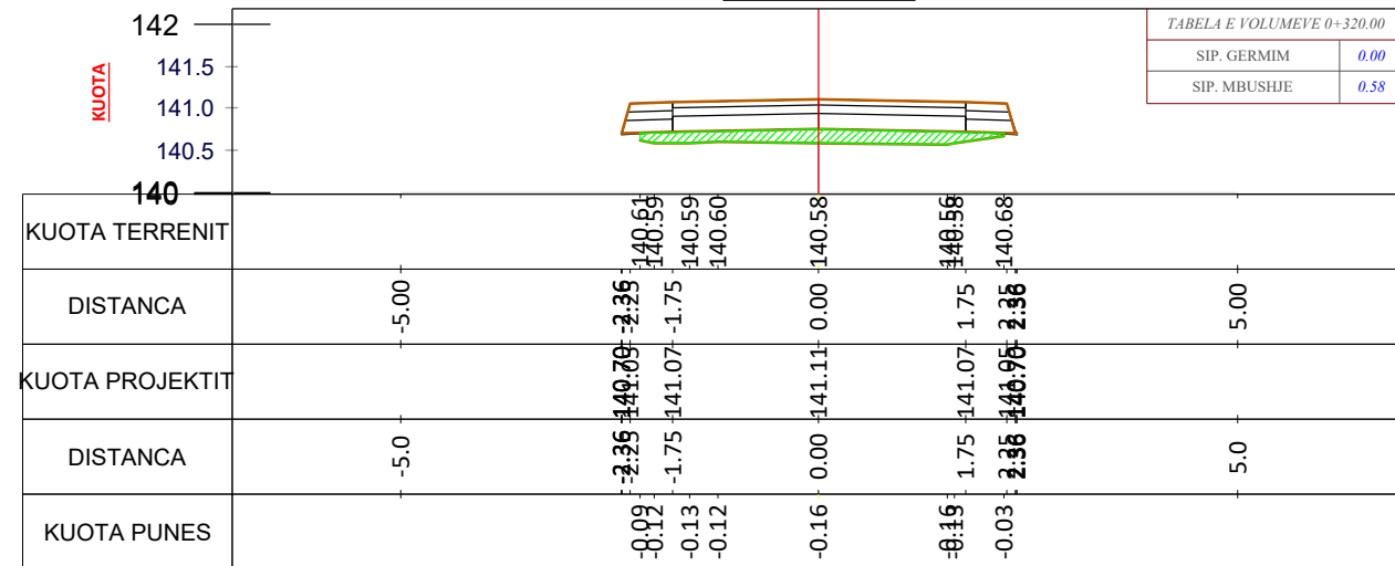
CS - 17 PROG - 0+320.0
