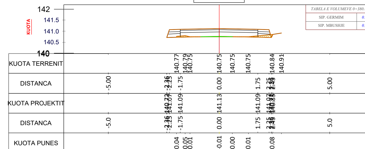
CS - 20 PROG - 0+380.0
