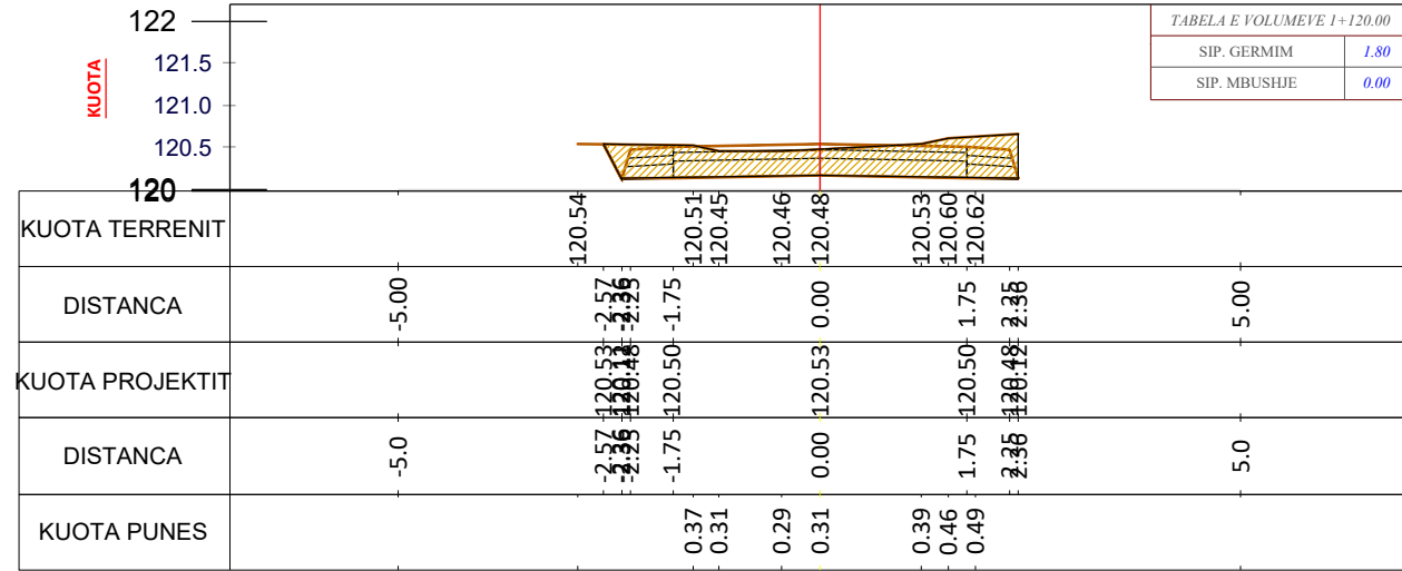
CS - 57 PROG - 1+120.0
