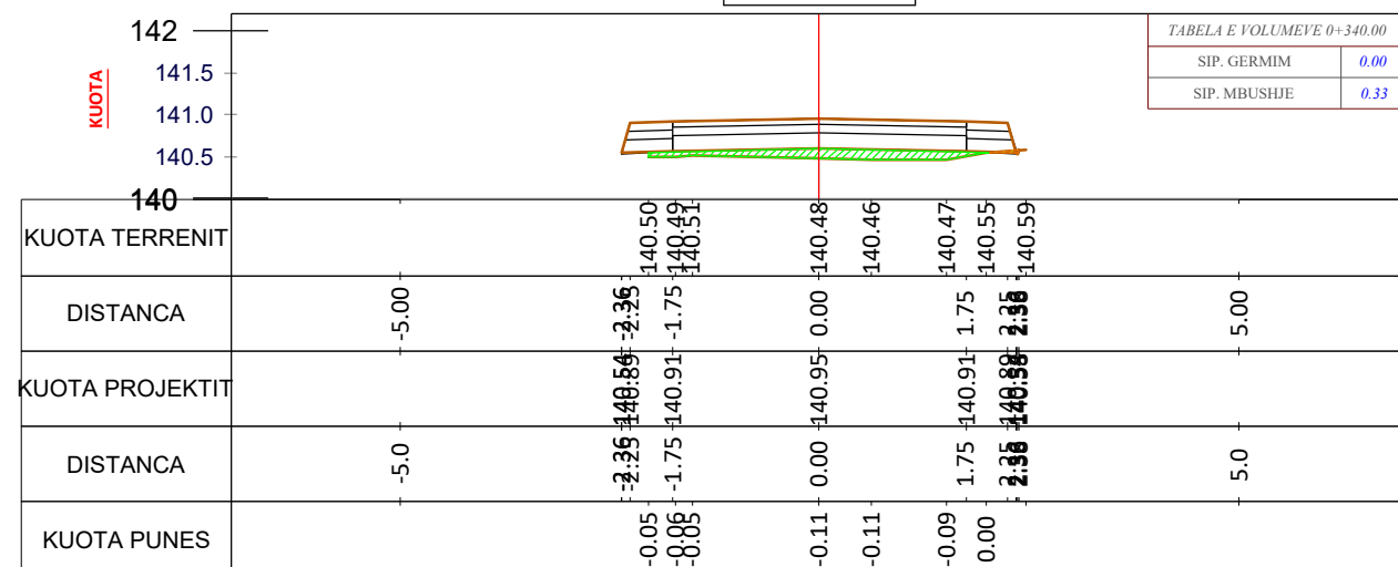
CS - 18 PROG - 0+340.0
