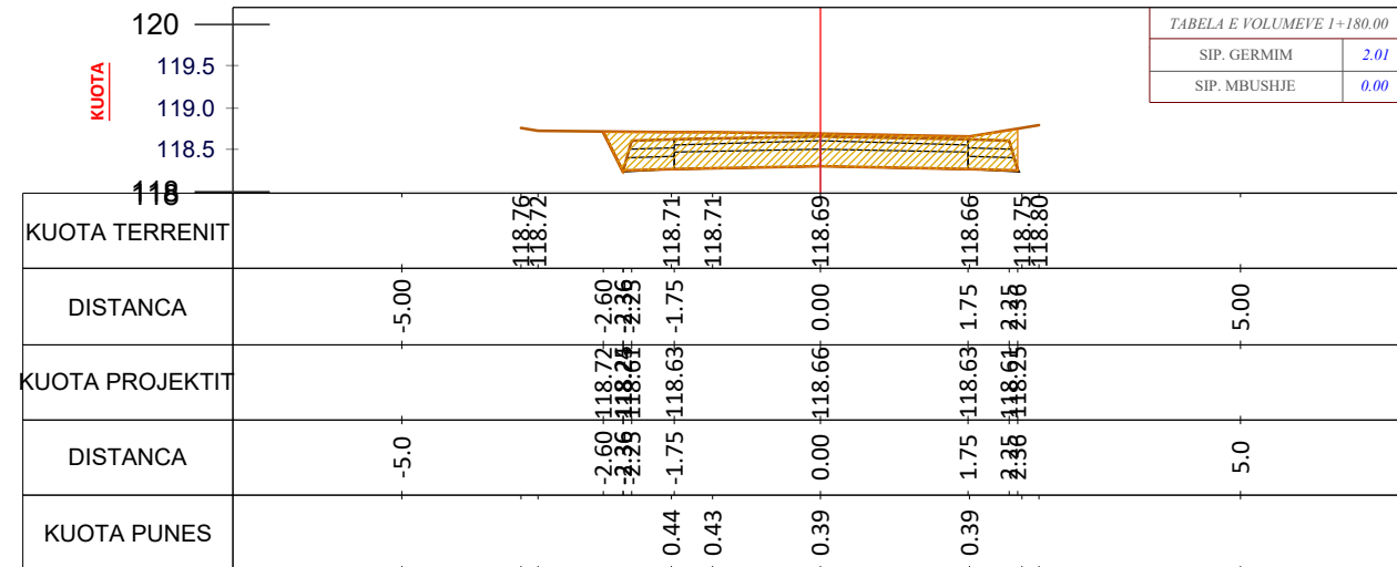
CS - 60 PROG - 1+180.0
