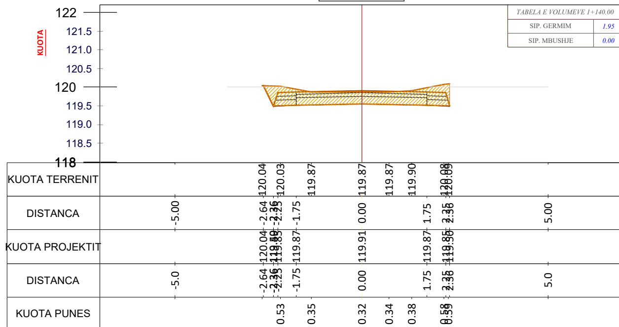
CS - 58 PROG - 1+140.0
