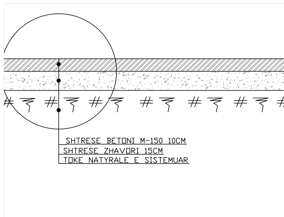
DETAJI A
