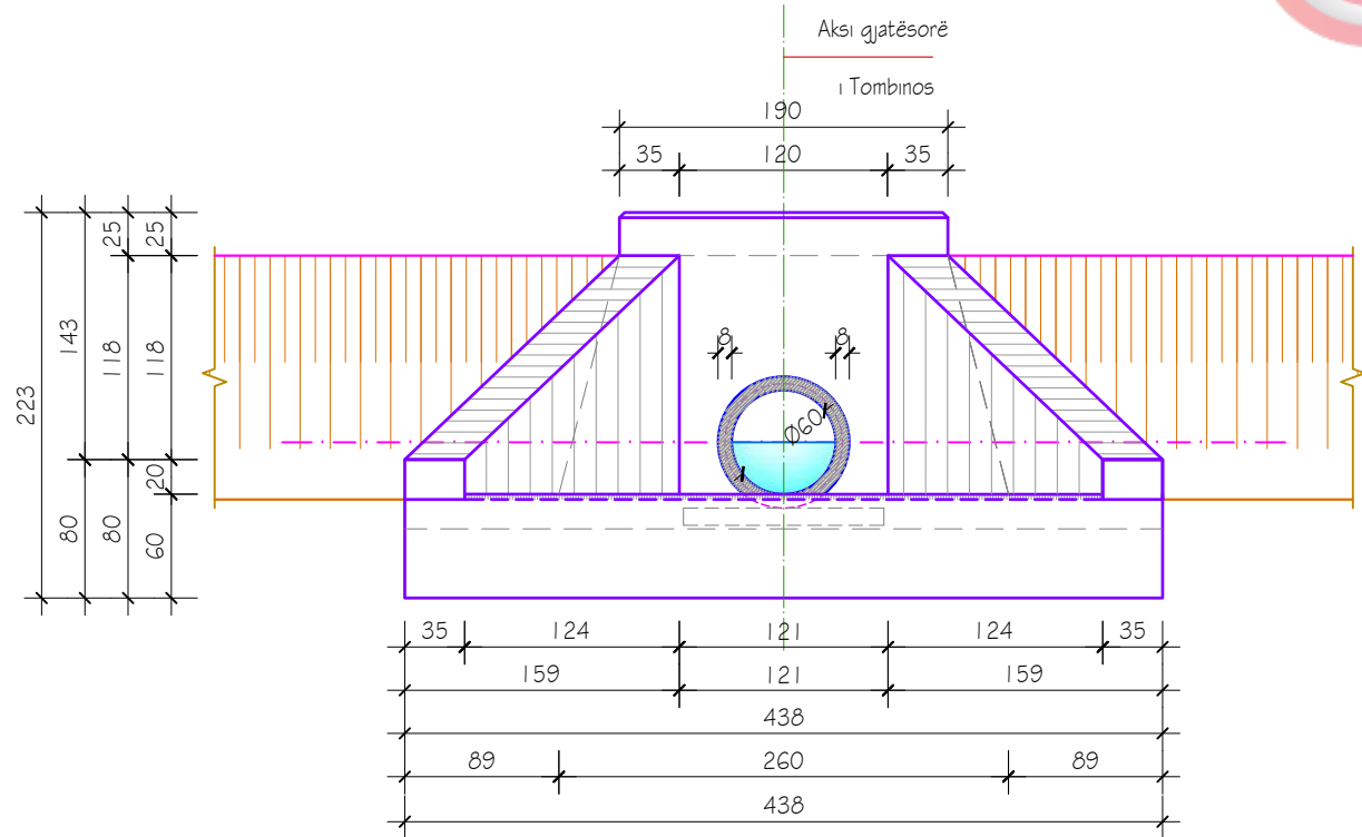
PRERJA B-B, Sh. 1:50
