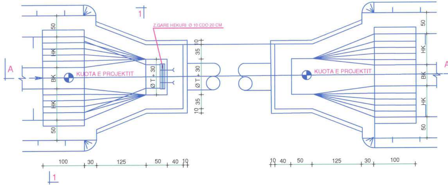
PLANIMETRIA SH. 1:50
