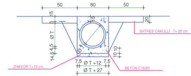
PRERJA 3-3 SH. 1:50
