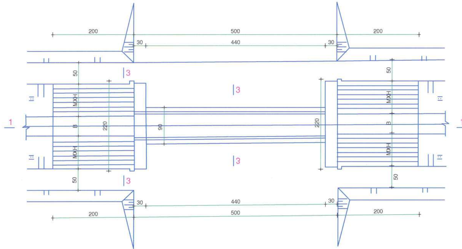
PLANIMETRIA SH. 1:50
