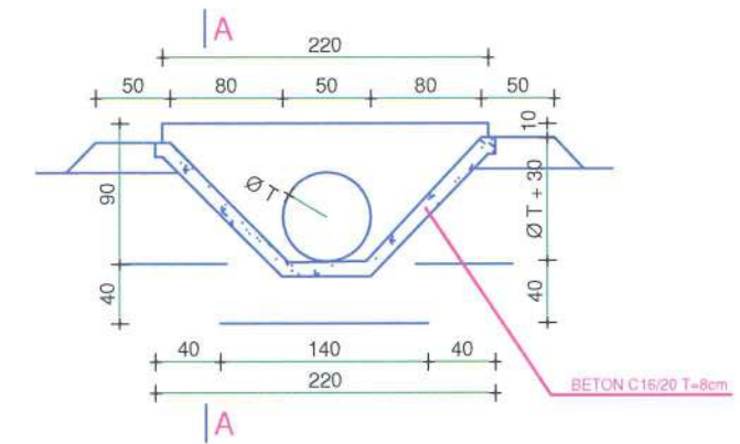
PRERJA 2-2 SH. 1:50
