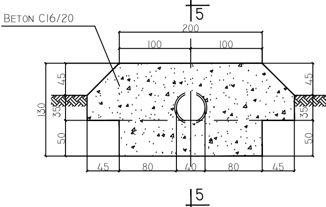
PRERJA 4 - 4 SH. 1:50
