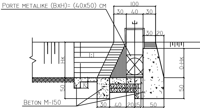
PRERJA 2 - 2 SH. 1:50
