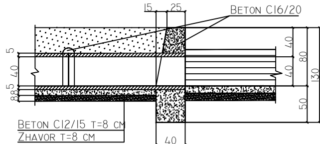
PRERJA 5 - 5 SH. 1:50
