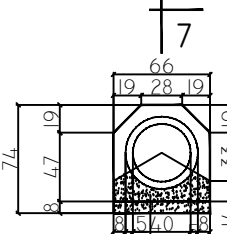
BETON C12/15 T=8 CM ZHAVOR T=8 CM /
