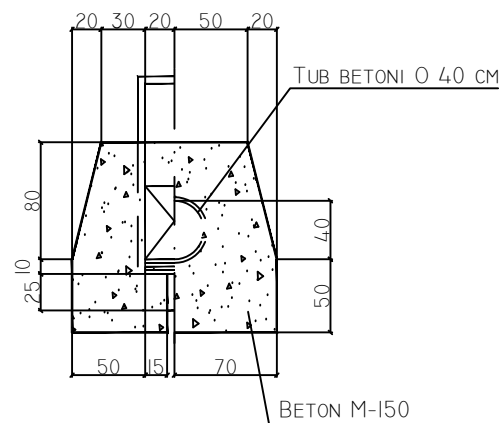
PRERJA 3 - 3 SH. 1:50
