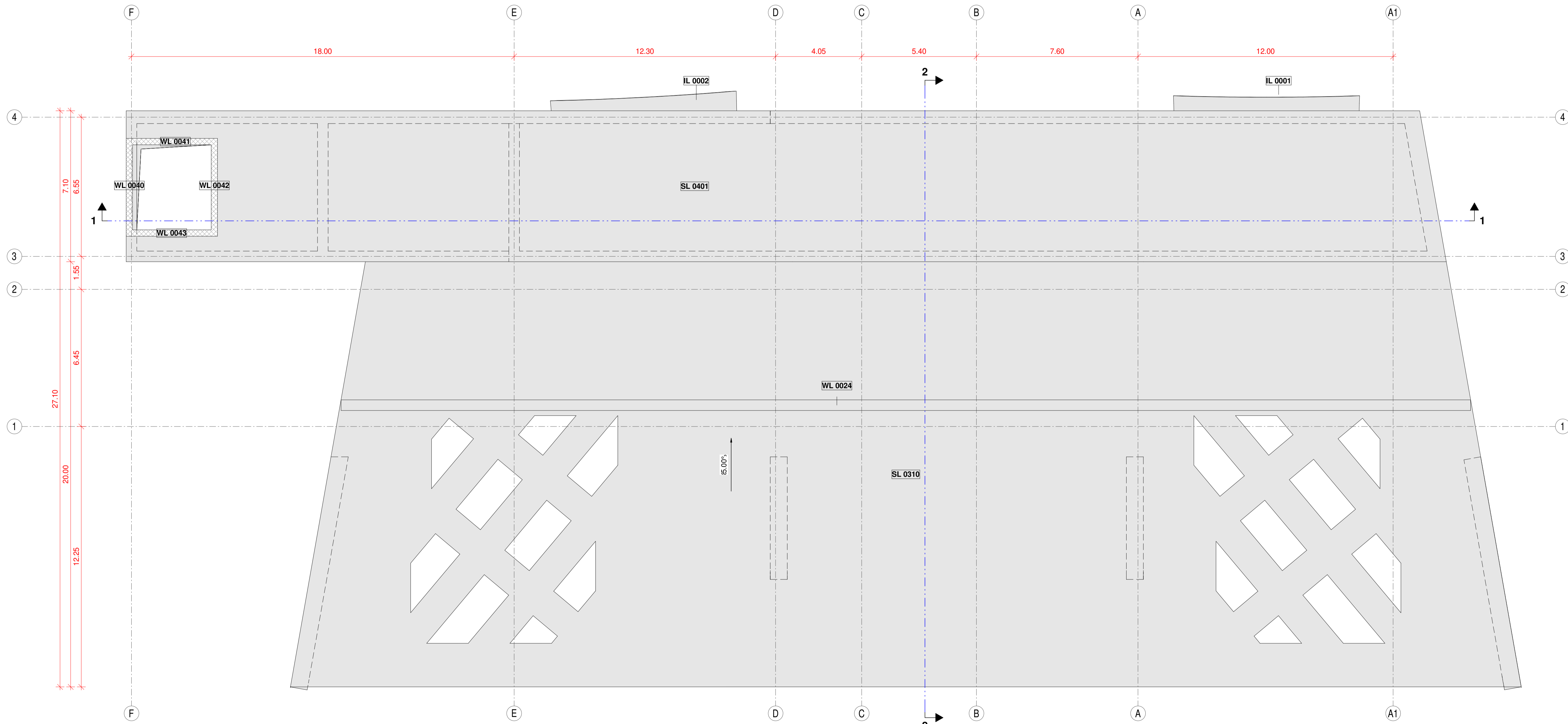
Plani +11.50 m / Plan View +11.50 m 1 : 100
