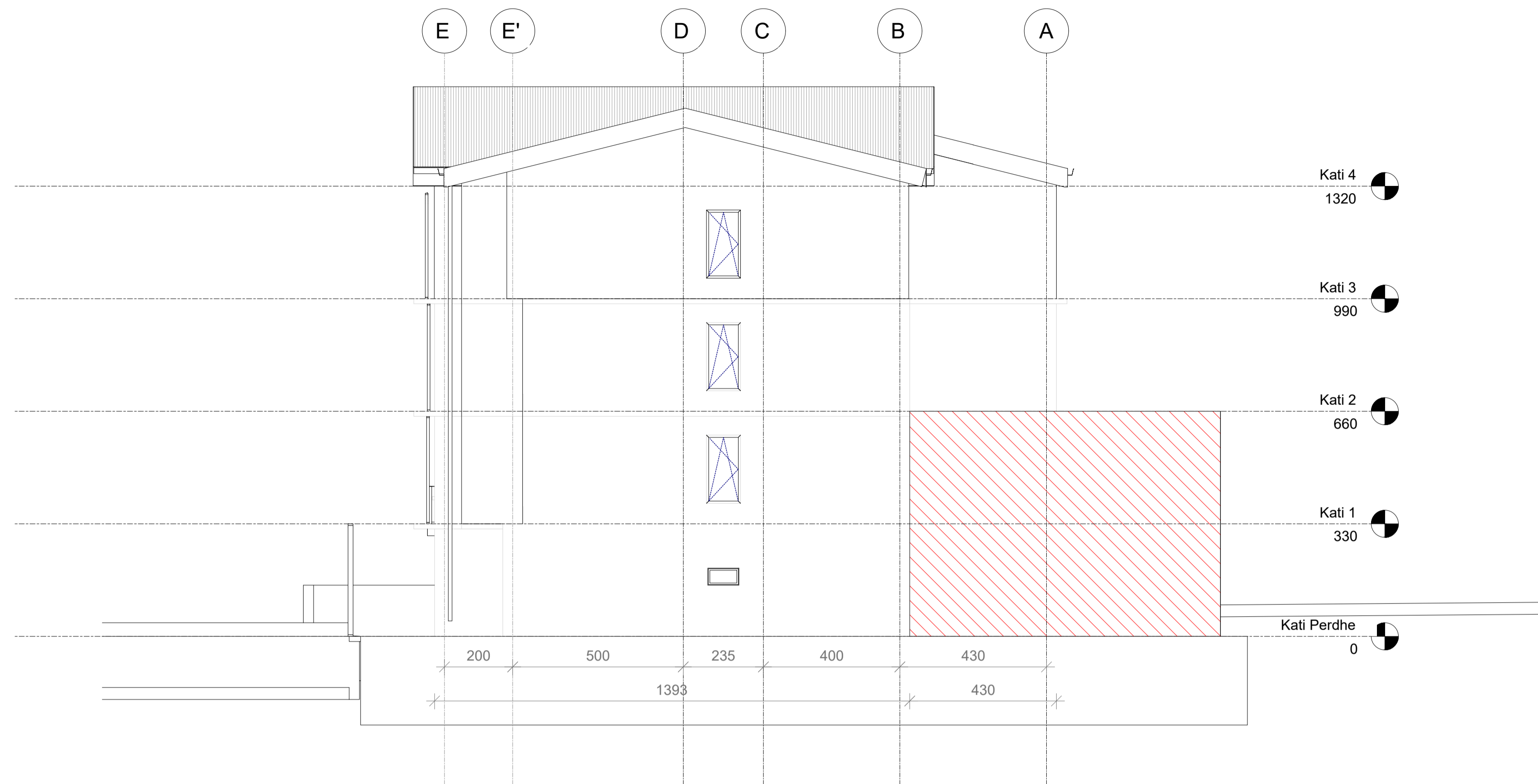
FASADA LINDORE
