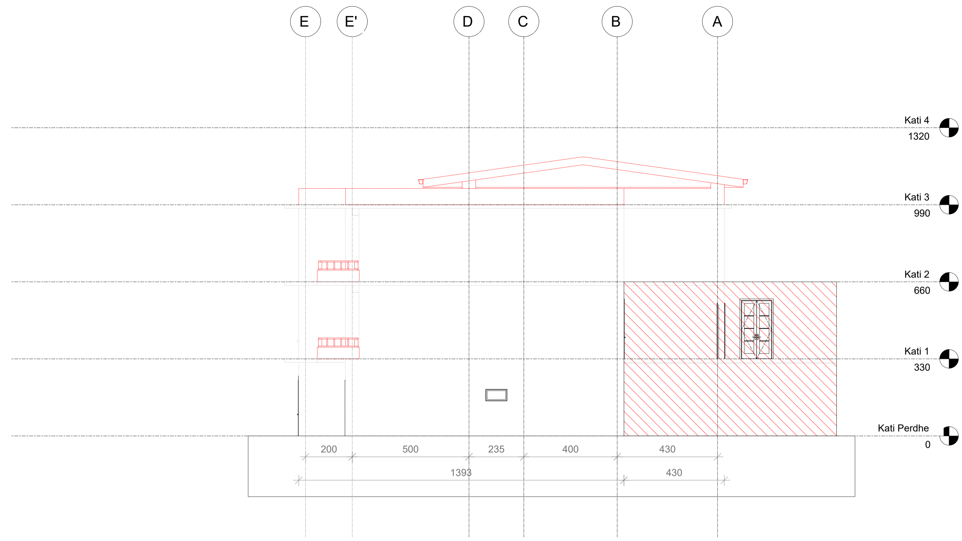
FASADA LINDORE
