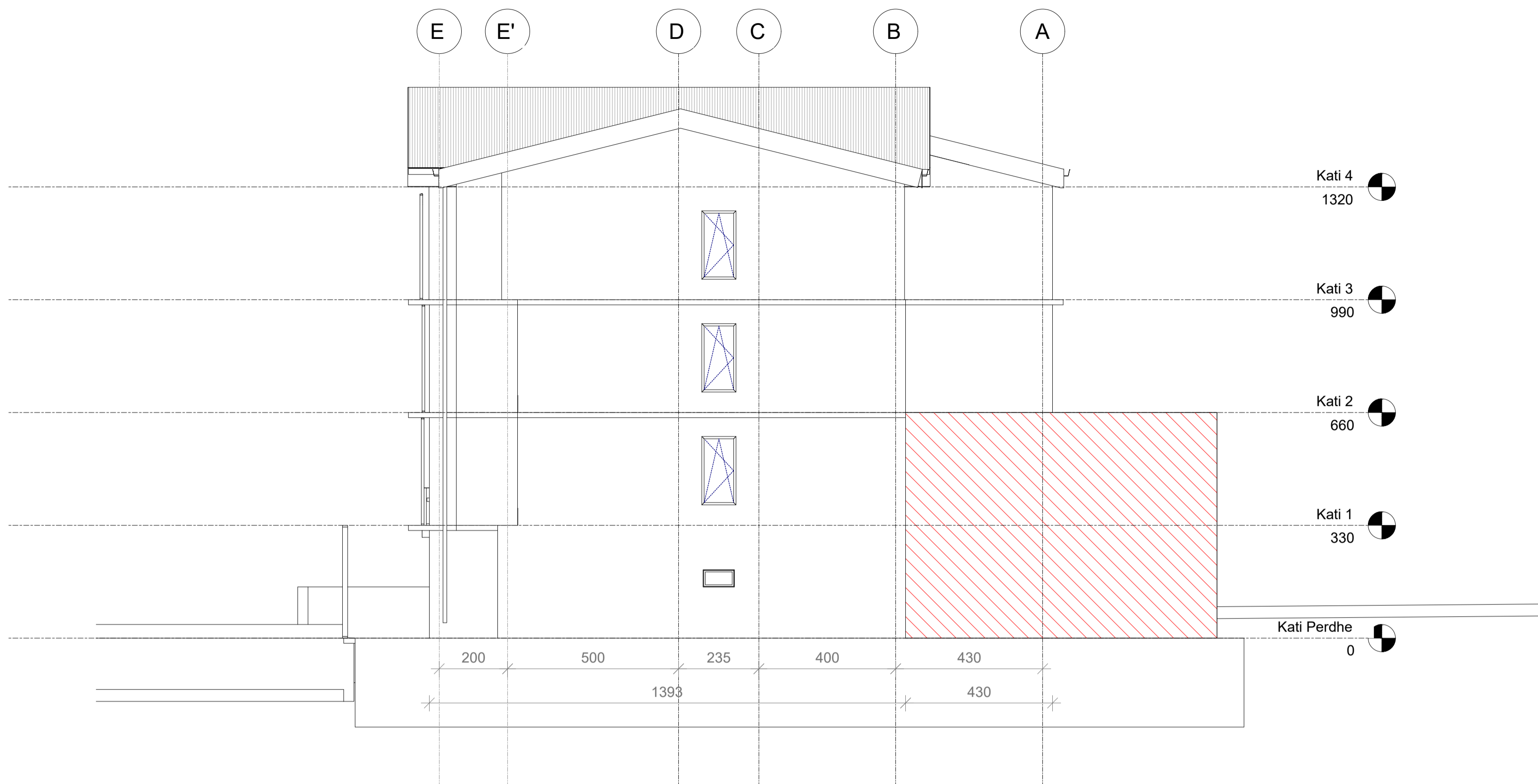
FASADA LINDORE
