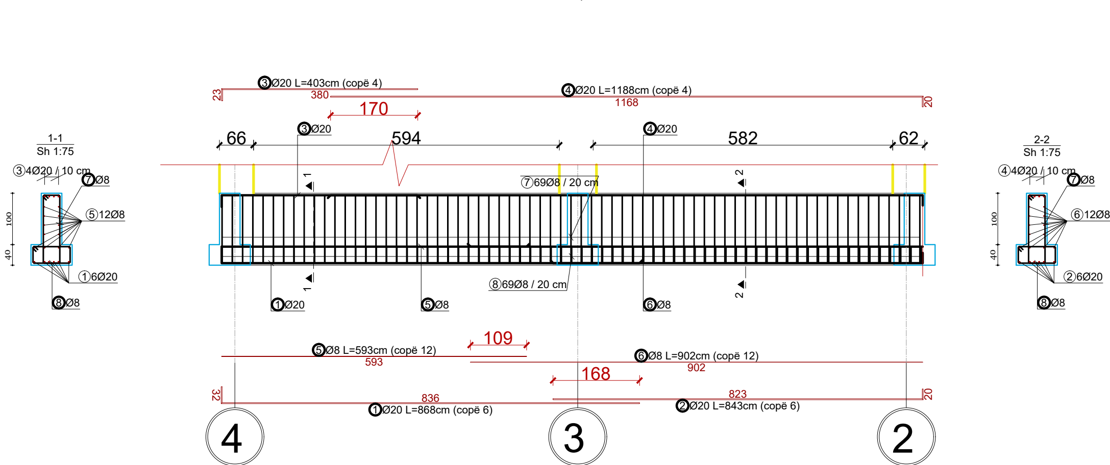
AKSI 4-3-2, Tra themeli T-2
