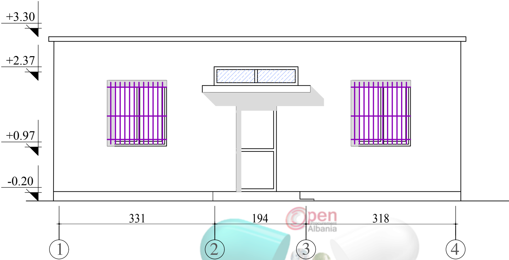
FASADA VERI - LINDORE SH. 1:50
