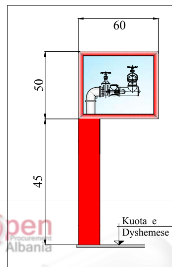
Kollona mbi toke per lidhjen me motopompen e MKZ
