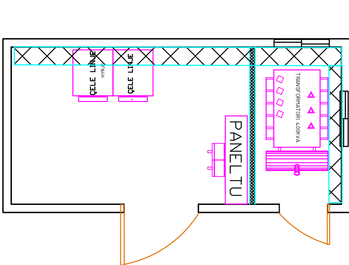
PLANIMETRIA EGZISTUESE KABINES "K2/A21" TR 250 KVA 20\0.4 KV
