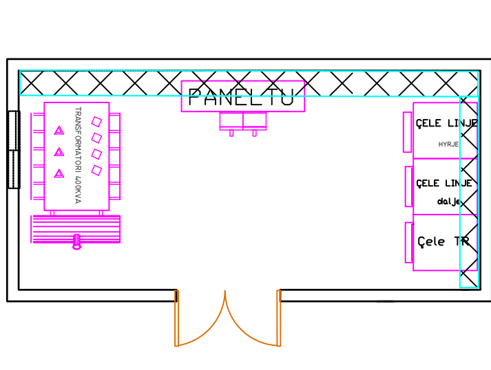
PLANIMETRIA EGZISTUESE KABINES "MAGAZINA E TREGTISE FA1" TR 800KVA 20\0.4 KV
