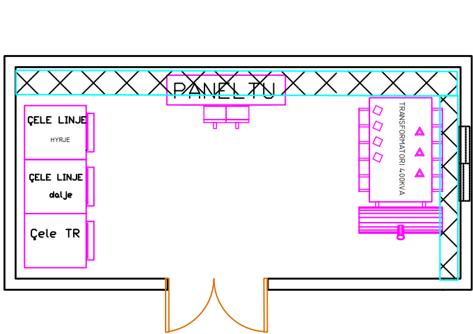
PLANIMETRIA EGZISTUESE KABINES "S.ZORBA 1/FC.4" TR 630KVA 20\0.4 KV
