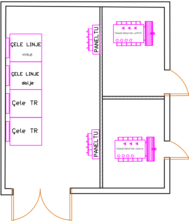
PLANIMETRIA EGZISTUESE KABINES "AL-MAK" FIDERI A4 RAJONAL TR 400/630KVA 20\0.4 KV
