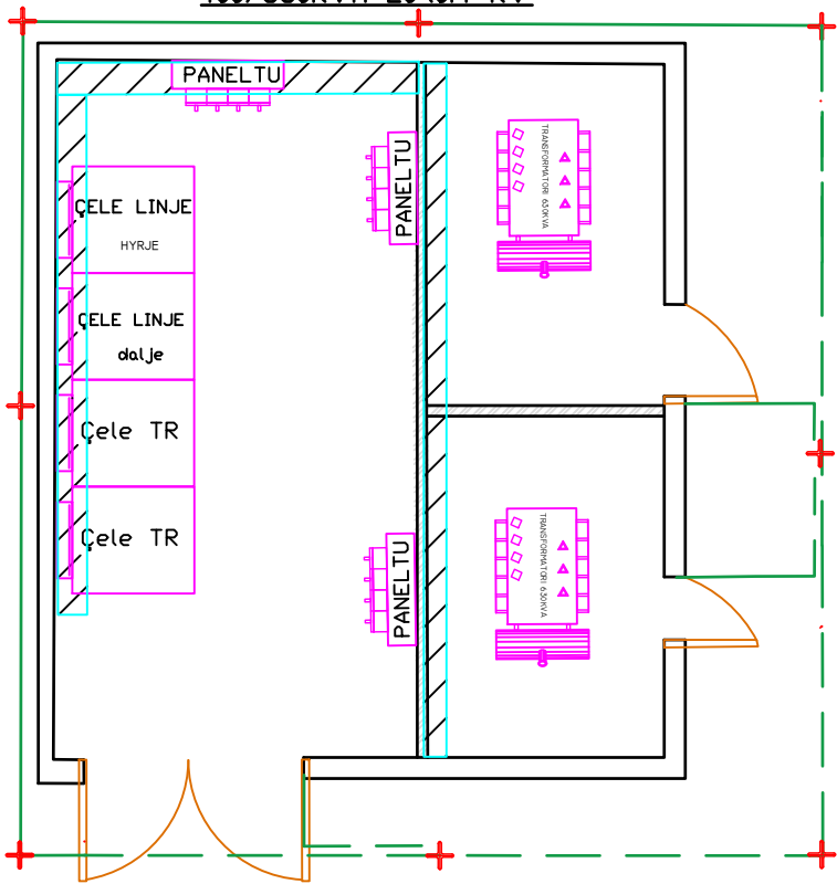
PLANIMETRIA EGZISTUESE KABINES "AL-MAK" FIDERI A4 RAJONAL TR 400/630KVA 20\0.4 KV
