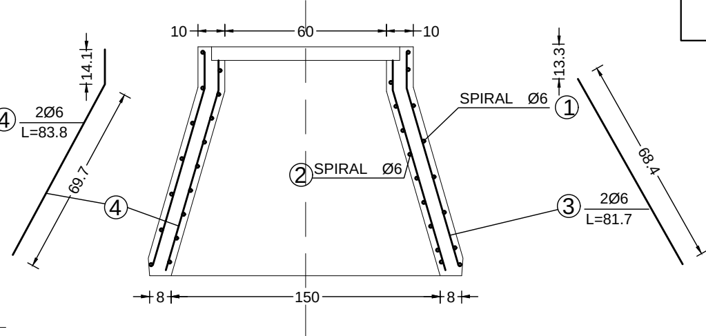
ELEMENT BETONI
