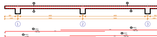
Armimi i soletes S2 Aksi A-A SH. 1:50
