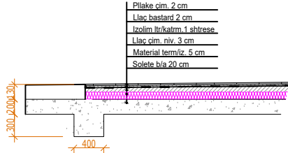
DETAJI I ÇATISE SH 1:25
