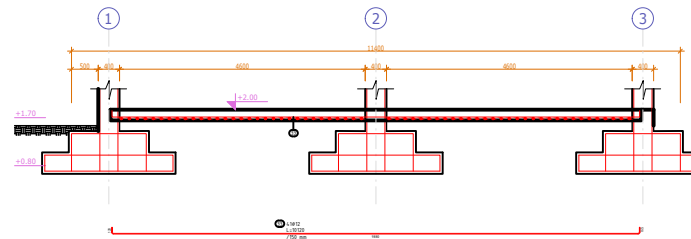
Armimi i soletes S1 Aksi A-A SH. 1:50
