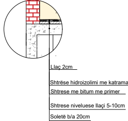
DETAJET E SHITESAVE TE DYSHEMESE +2.00 SH 1:25
