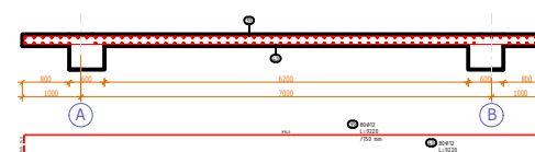
Armimi i soletes S2 Aksi 1-1 SH. 1:50
