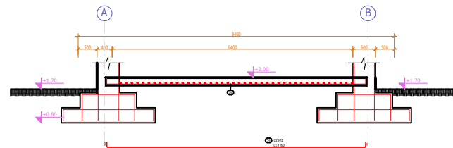
Armimi i soletes S1 Aksi 1-1 SH. 1:50
