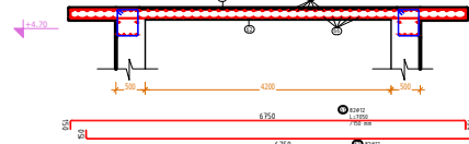
Armimi i Soletes S3 Prerja 3-3 SH. 1:50
