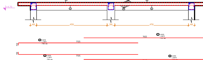
S3 Slab Reinforcement /Armimi i Soletes S3 Section/Prerja B-B Sc/SH 1:50
