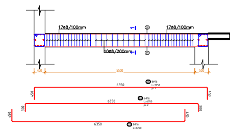
Armimi i Traut T6 (Cope 2) SH 1:50
