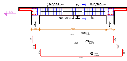
Armimi i Traut T6 (Cope 2) SH 1:50
