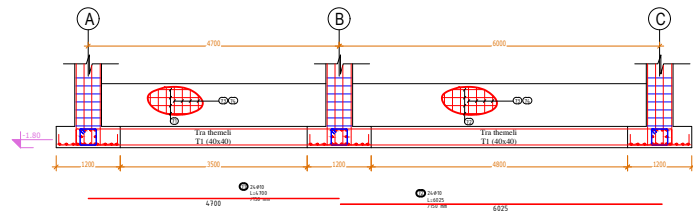
Armimi i Murit (Cope 2) Aksi 1-1SH. 1:50
