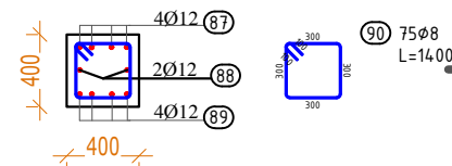
Prerja 1-1 Trau T9 Sh.1:25
