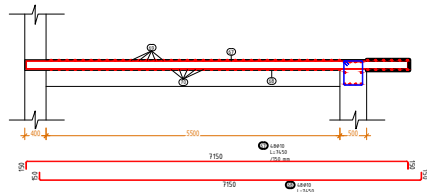
Armimi i Soletes S4 Prerja 2-2 SH. 1:50
