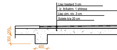
Detaji i Soletes SH 1:25
