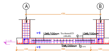
Armimi i Themelit Trau T3 (Cope 1) Aksi 3-3 SH.1:50
