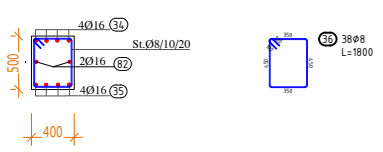
Prerja 1-1 trau T8 Sh 1:25
