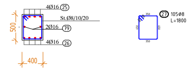
Prerja 1-1 trau T5 Sh 1:25
