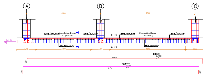
Armimi i Themelit Trau T1 (Cope 2) Aksi 1-1 SH.1:50
