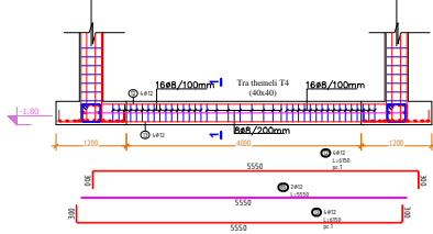
Armimi i Themelit Trau T4 (Cope 1) Aksi C-C SH.1:50
