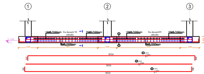
Armimi i Themelit Trau T9 (Cope 1) Aksi D-D SH.1:50
