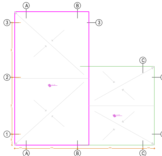
PLANI I KULLIMIT TE SOLETES SH. 1:75
