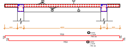
Armimi i Soletes S4 Prerja C-C SH. 1:50
