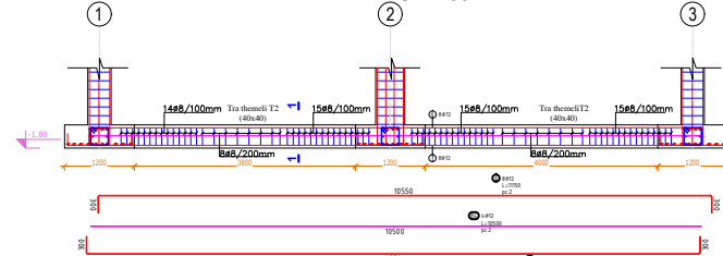
Armimi i Themelit Trau T2 (Cope 2) Aksi A-A SH.1:50
