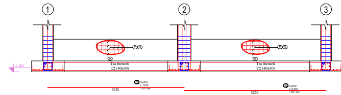
Armimi i Murit (Cope 2) Aksi A-A SH. 1:50
