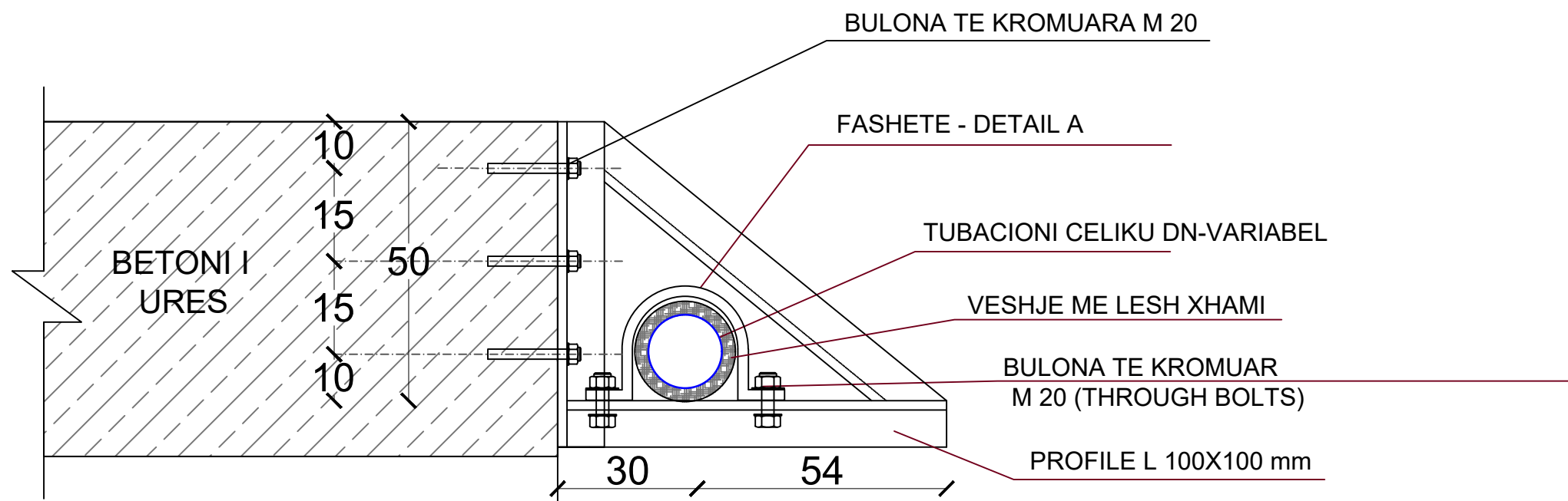
Detail A / Detaji A
