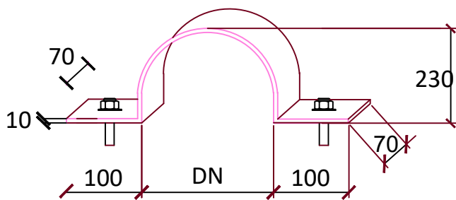
Detail A / Detaji A
