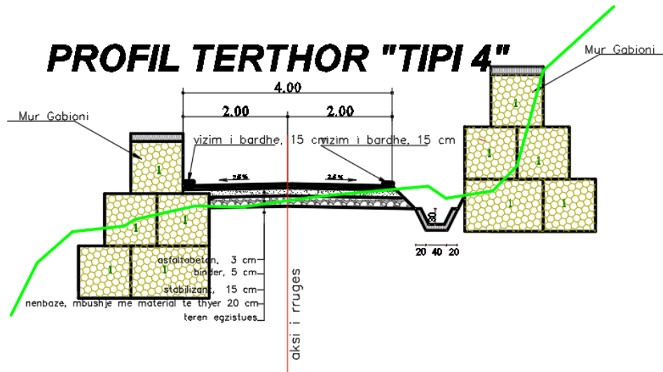
Figure II-6 - Profil terthor tip 4
