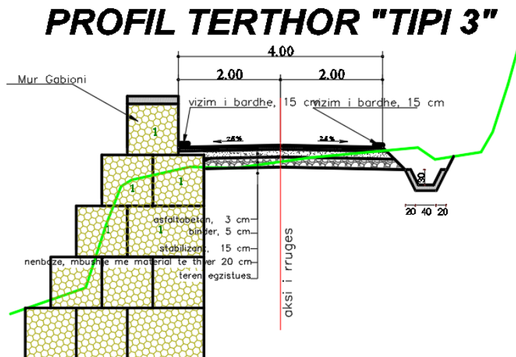
Figure II-5 - Profil terthor tip 3
