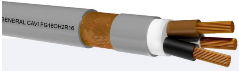
Figura 8-4: Kabllo FG16H2R16, 0.6/1KV
