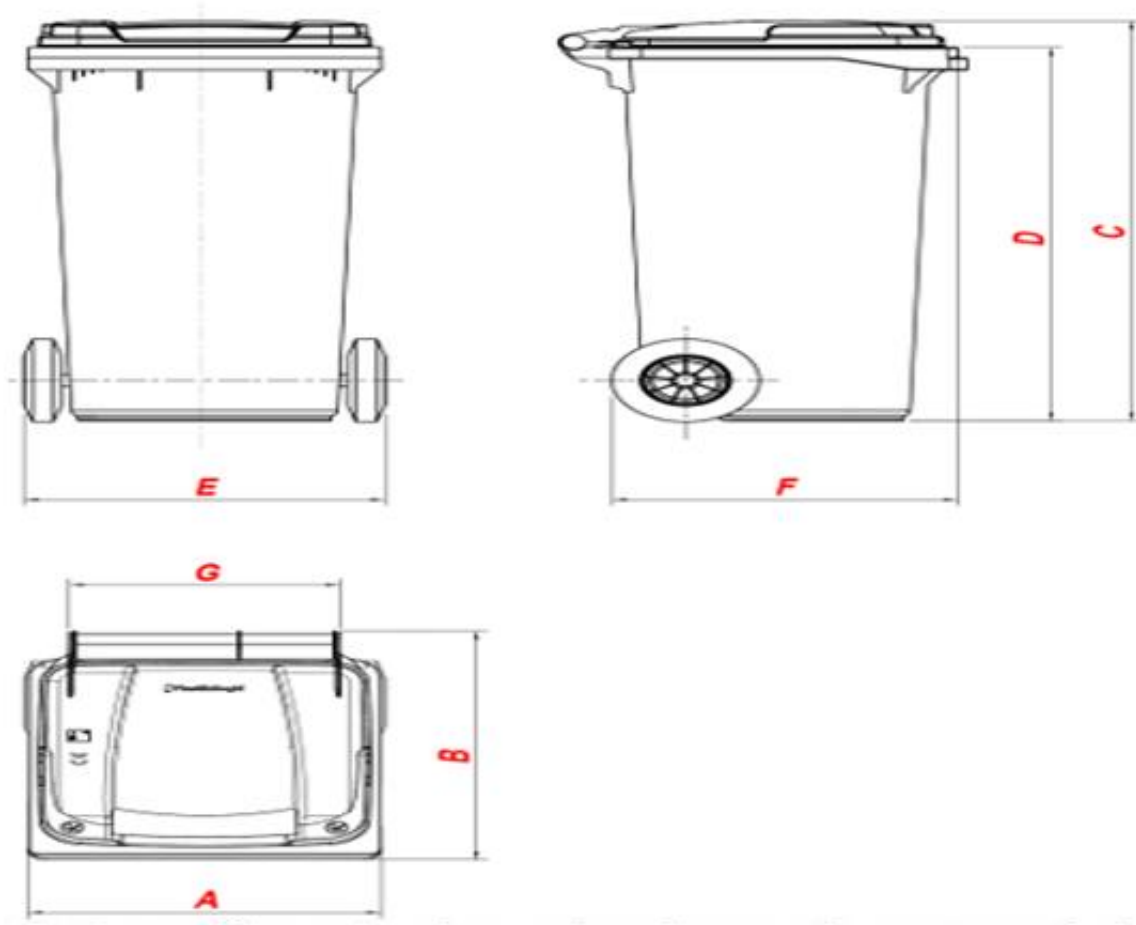
Skicë orientuese e koshit plastik 120 L
