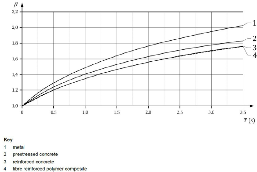
Figure 1 — Coefficient \beta for the dynamic behaviour of columns
