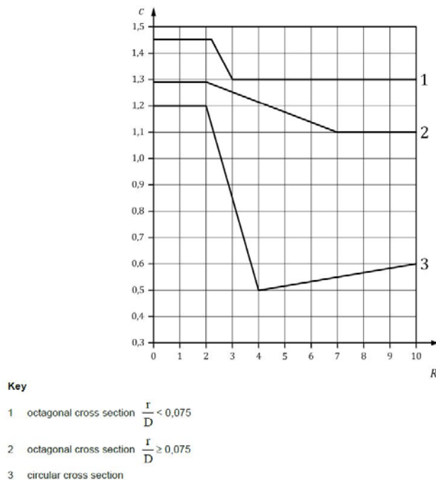
Figure 3 — Shape coefficient for circular and octagonal cross-sections
