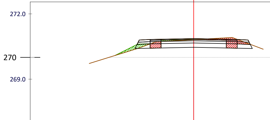
CS - 70 PROG - 1+380.0
