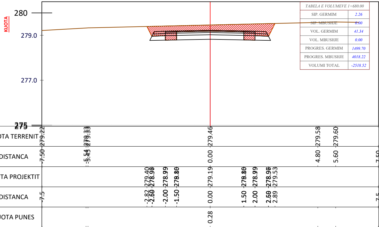
CS - 85 PROG - 1+680.0
