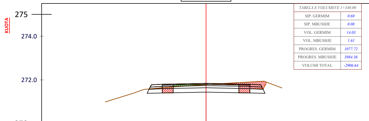
CS - 68 PROG - 1+340.0
