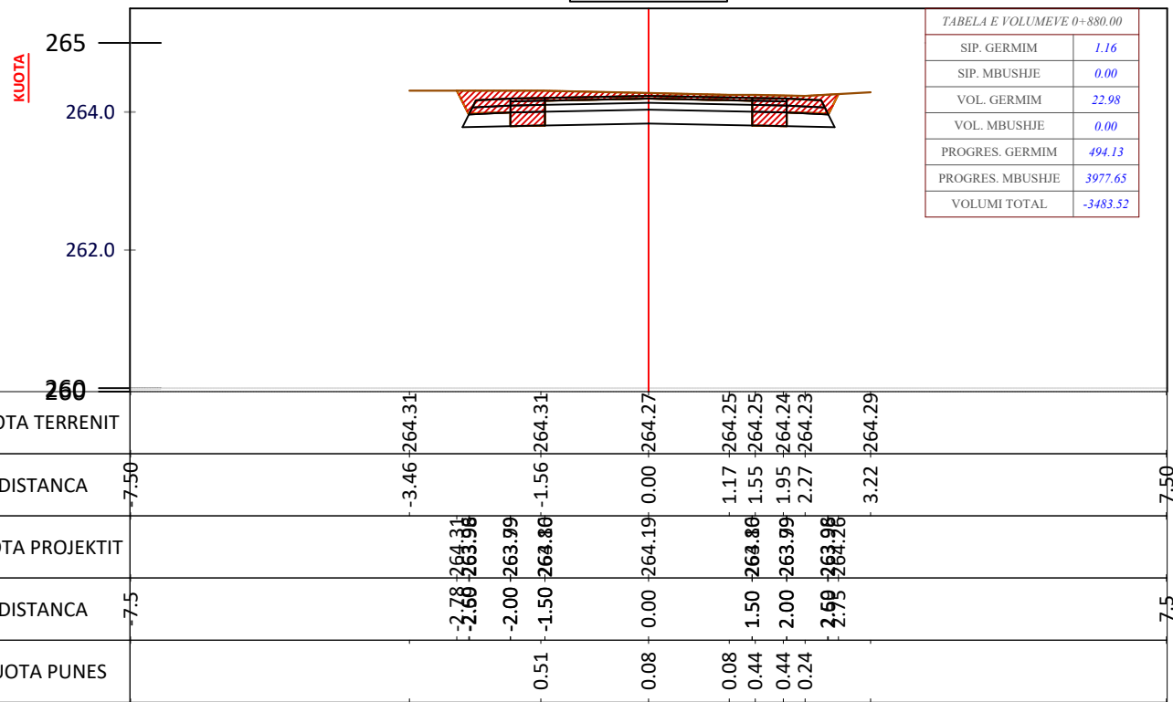
CS - 45 PROG - 0+880.0
