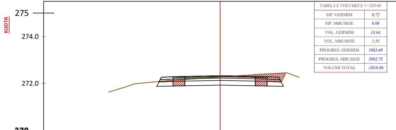
CS - 67 PROG - 1+320.0
