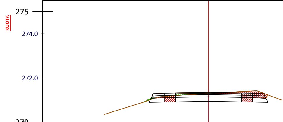
CS - 69 PROG - 1+360.0
