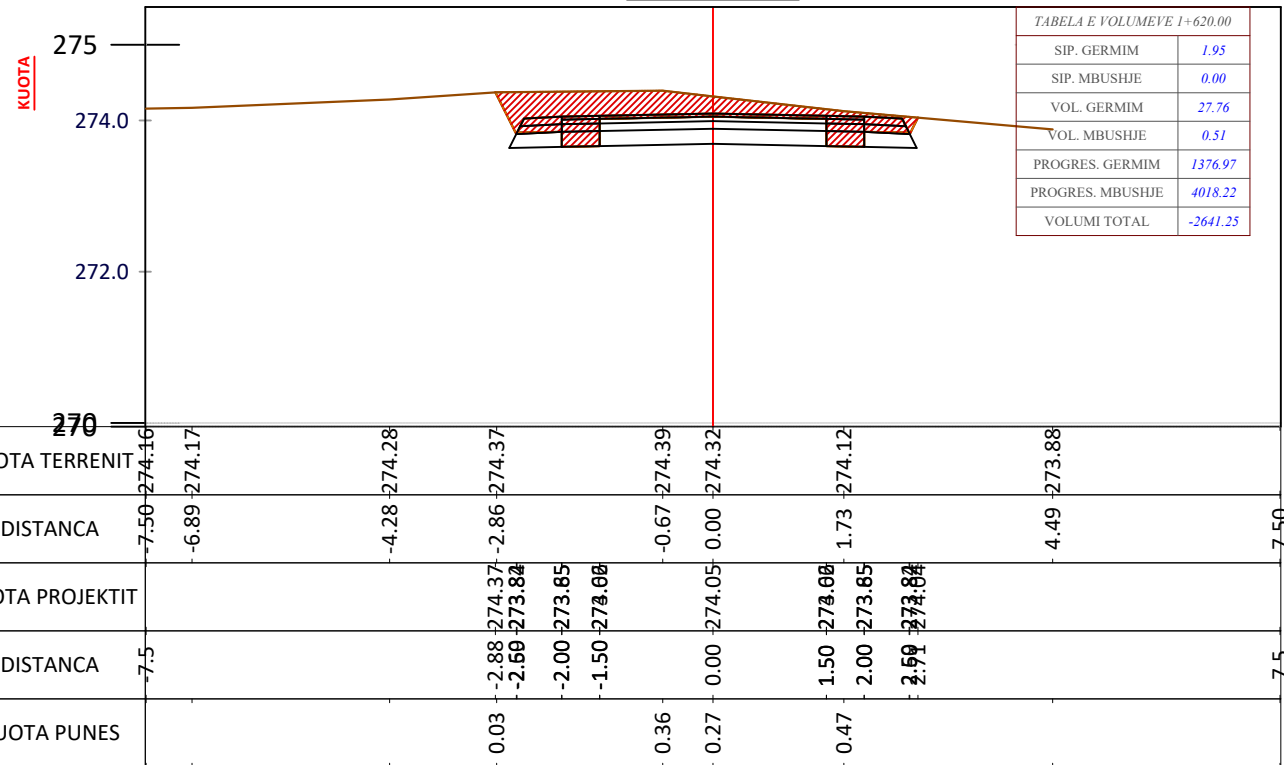
CS - 82 PROG - 1+620.0
