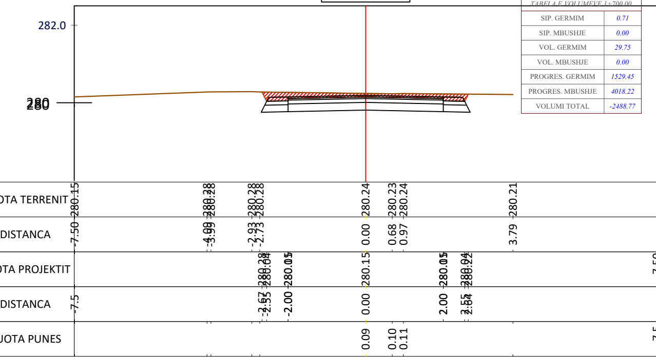
CS - 86 PROG - 1+700.0
