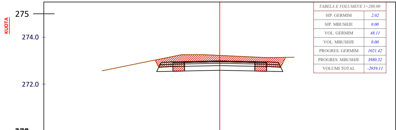
CS - 65 PROG - 1+280.0
