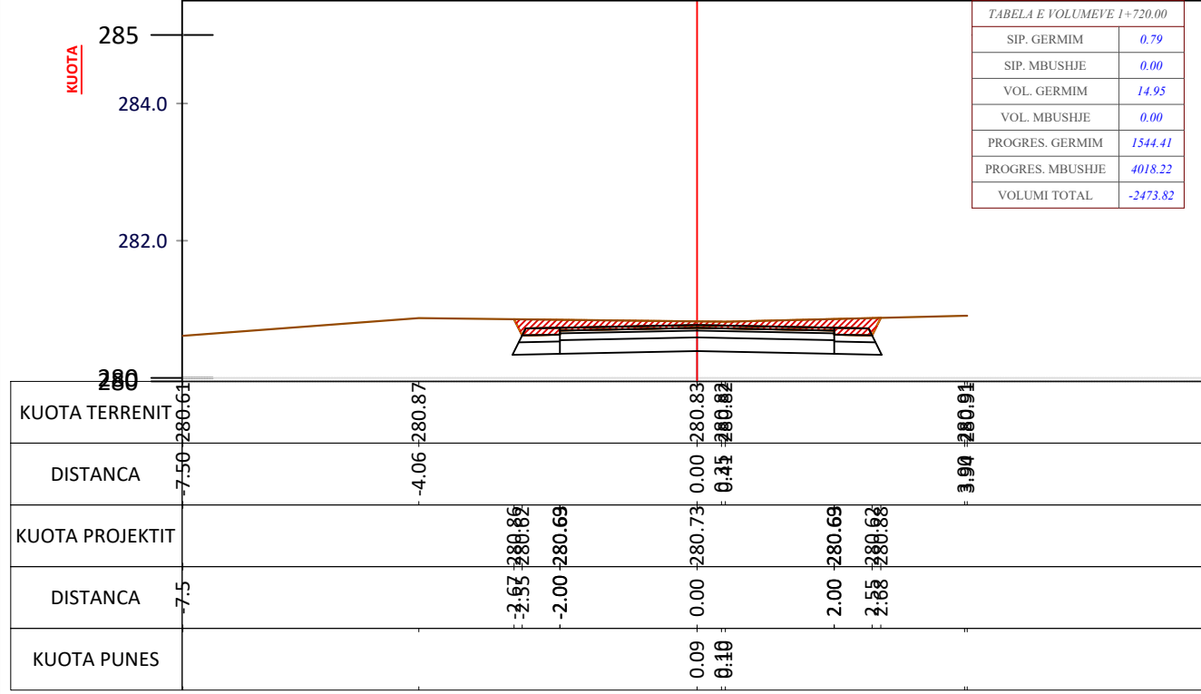
CS - 87 PROG - 1+720.0
