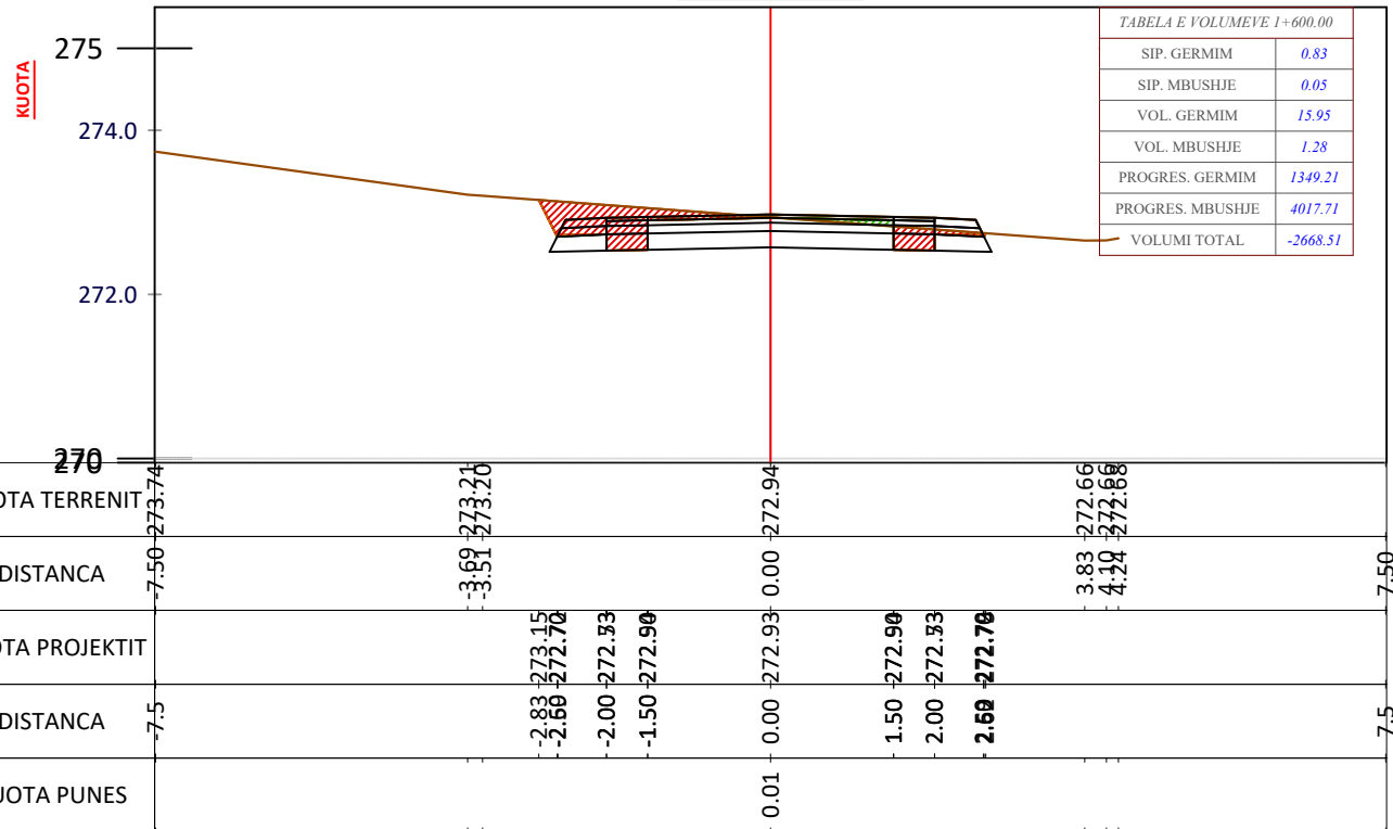
CS - 81 PROG - 1+600.0
