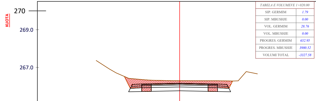
CS - 52 PROG - 1+020.0
