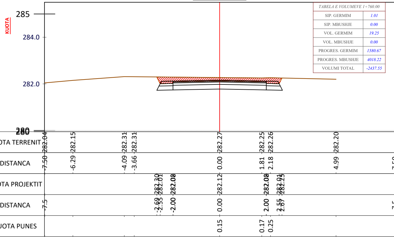
CS - 89 PROG - 1+760.0
