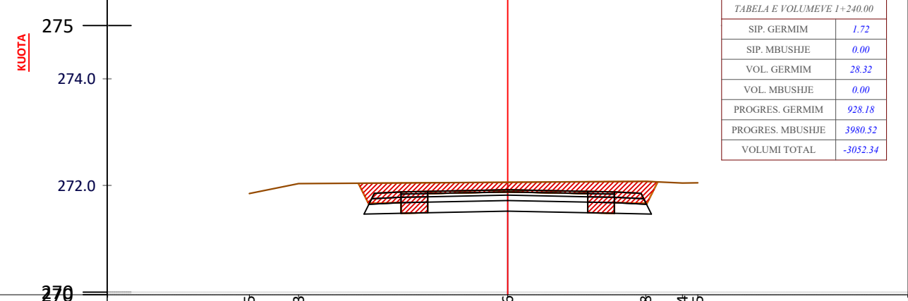
CS - 63 PROG - 1+240.0
