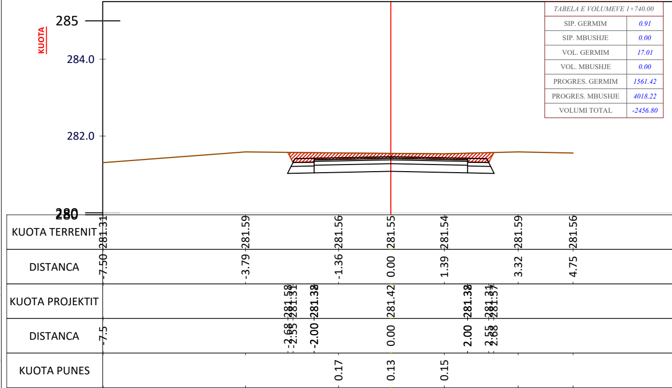
CS - 88 PROG - 1+740.0
