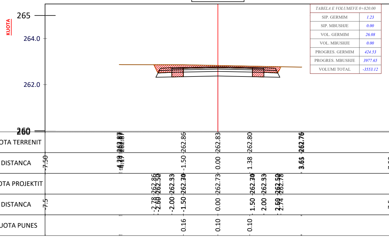
CS - 42 PROG - 0+820.0
