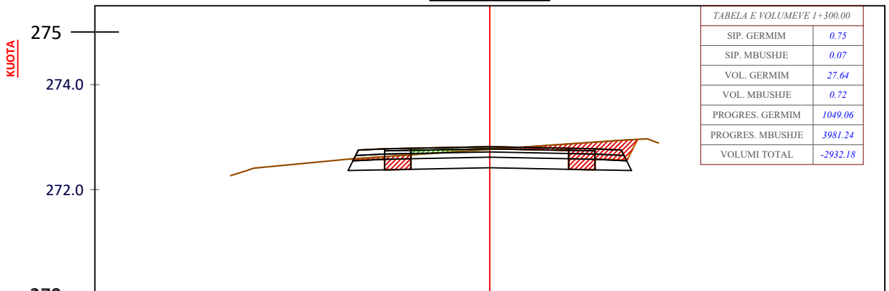
CS - 66 PROG - 1+300.0
