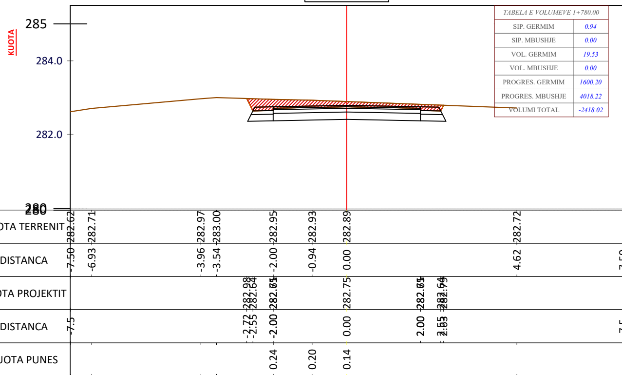
CS - 90 PROG - 1+780.0
