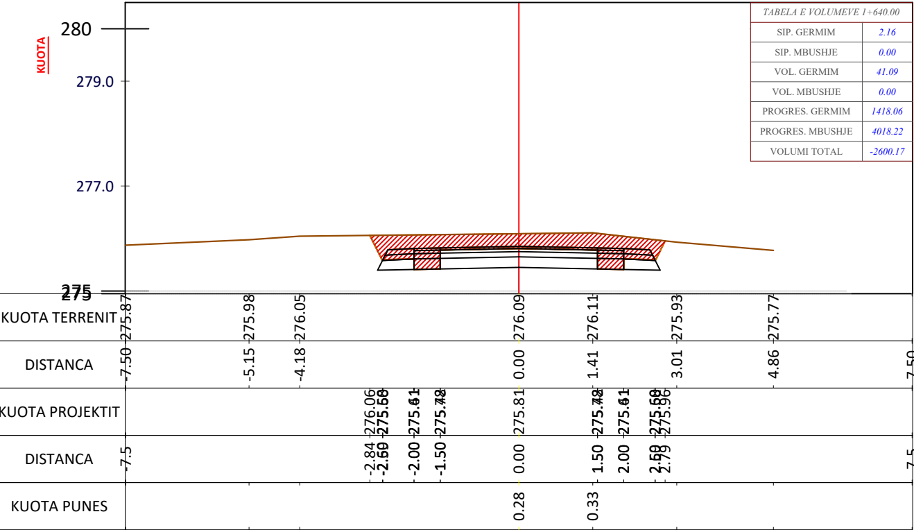
CS - 83 PROG - 1+640.0
