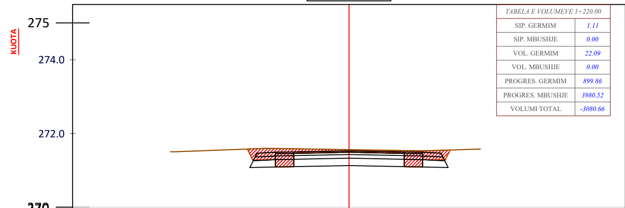
CS - 62 PROG - 1+220.0
