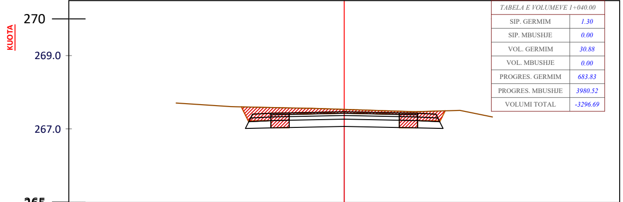
CS - 53 PROG - 1+040.0
