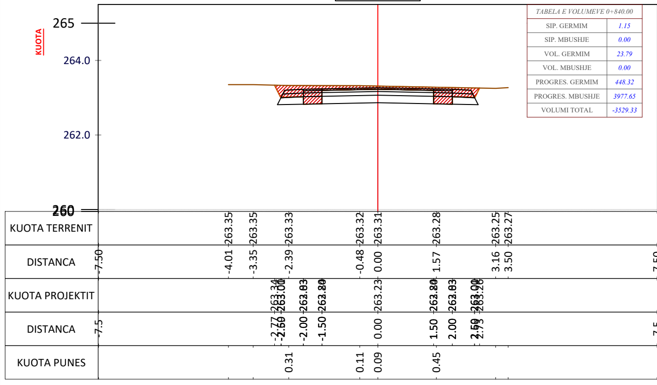
CS - 43 PROG - 0+840.0
