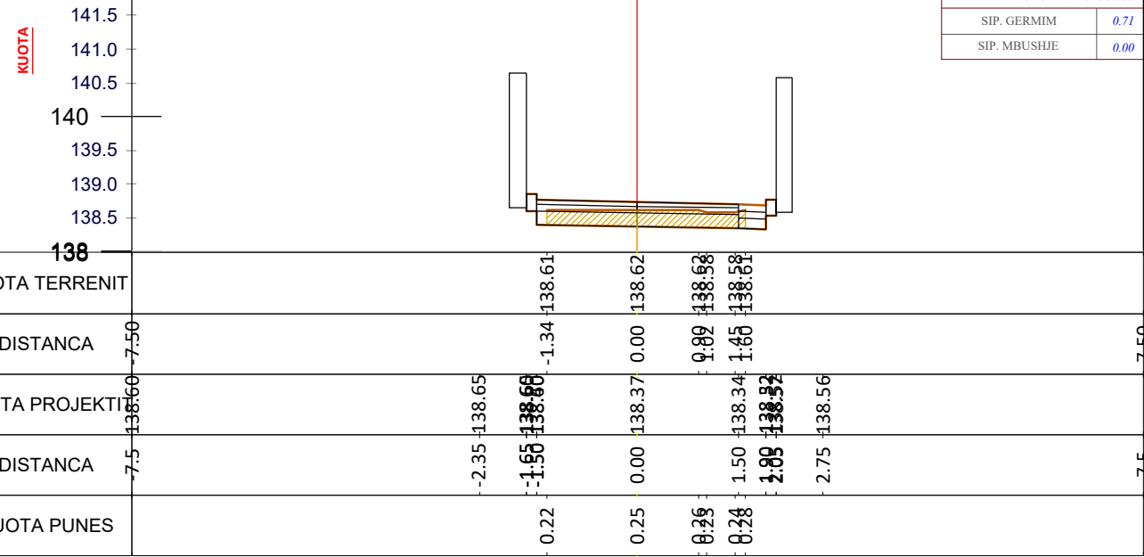
CS - 20 PROG - 0+380.0
