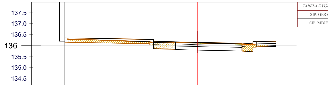
CS - 8 PROG - 0+140.0
