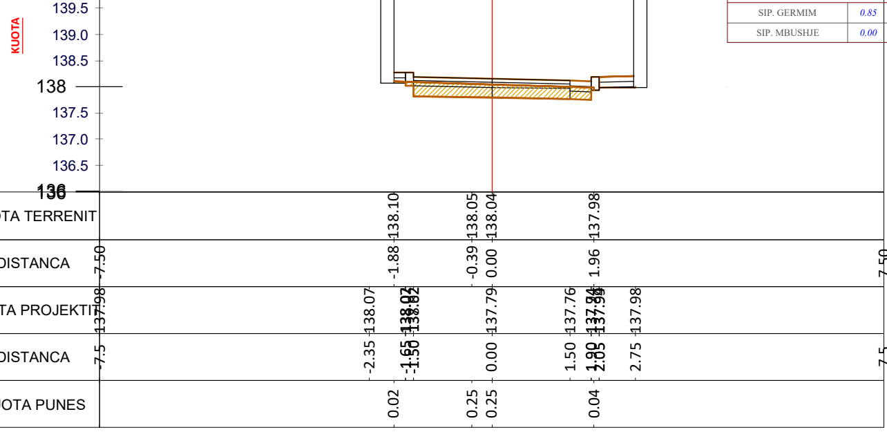
CS - 19 PROG - 0+360.0
