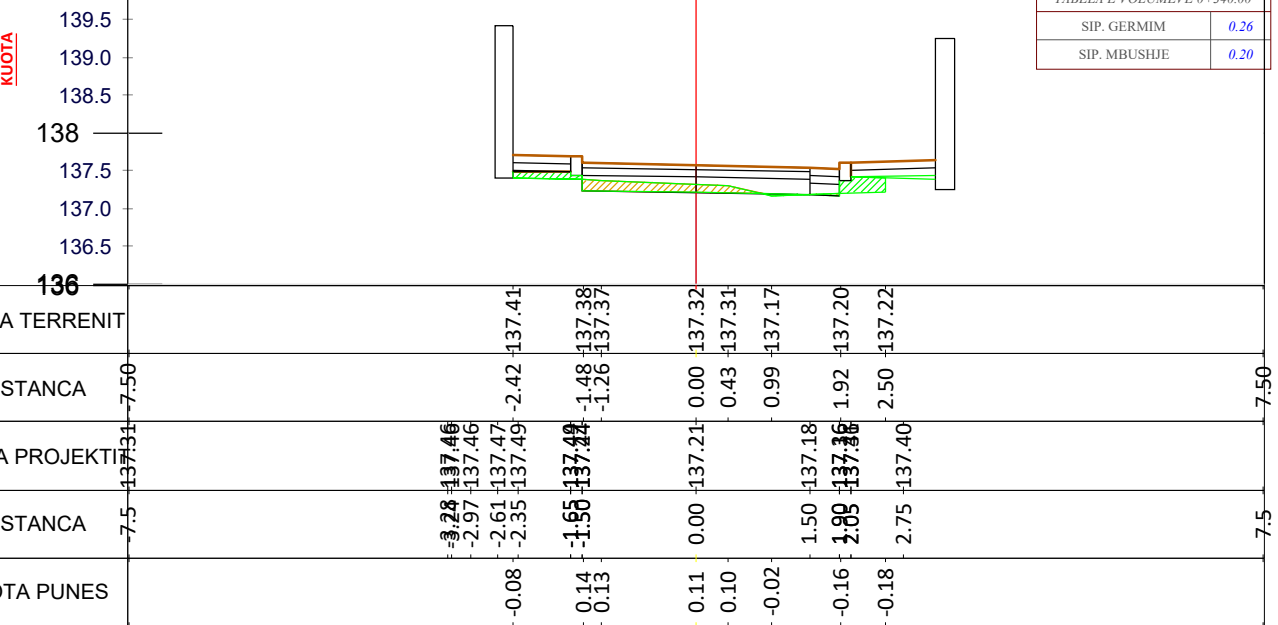
CS - 18 PROG - 0+340.0
