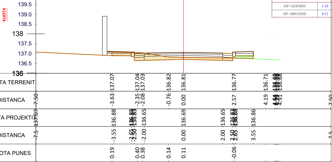
CS - 17 PROG - 0+320.0
