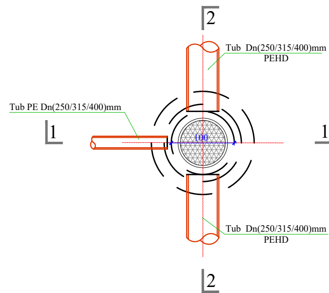
PLAN SH.1:50
