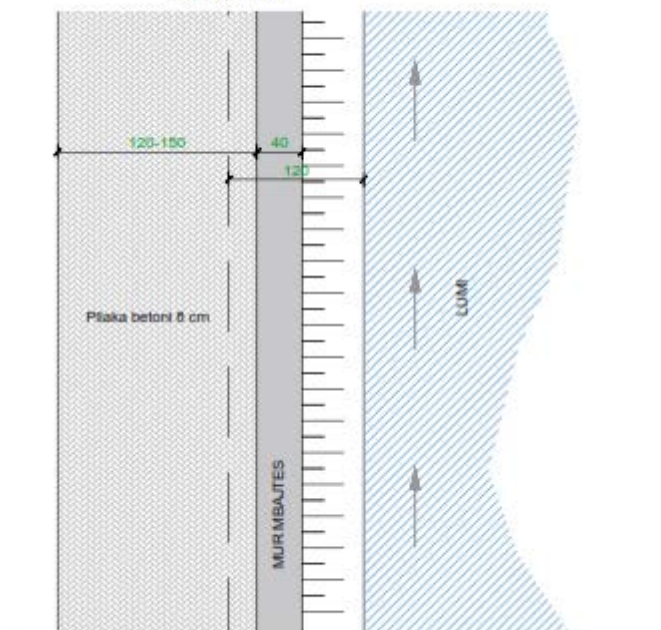
FRAGMENT PLANIMETRIE SHK. 1 :50
