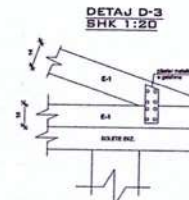
DETAJI 1
