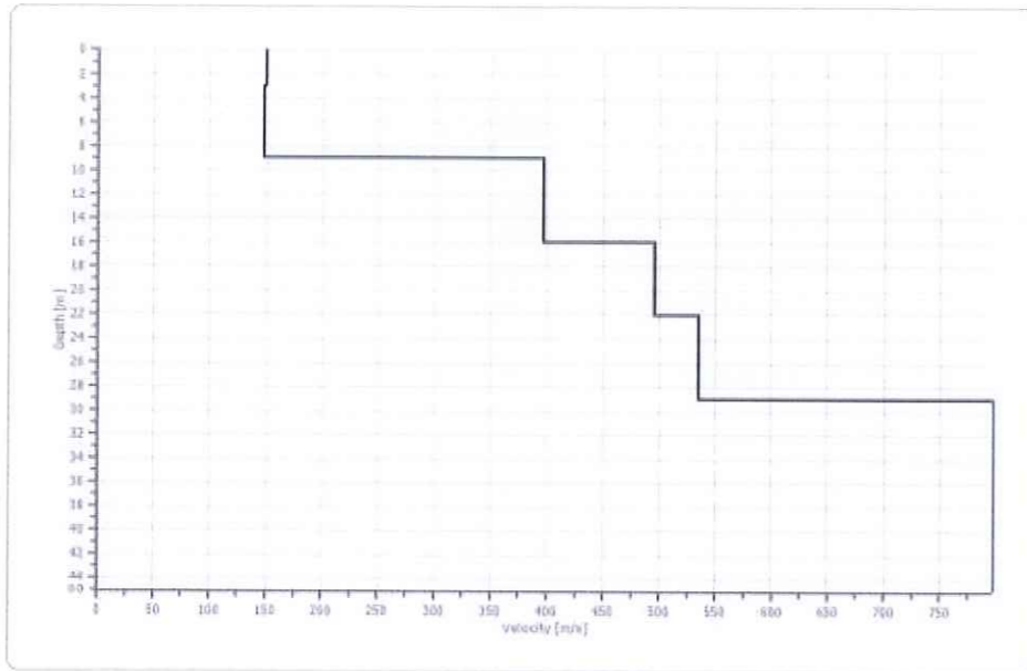
Velocity profile
