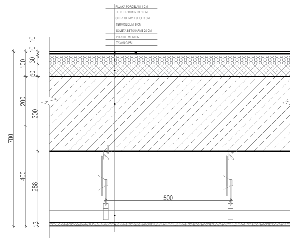
5 TERRACE DETAIL / DETAJ TARRACE 1:8
