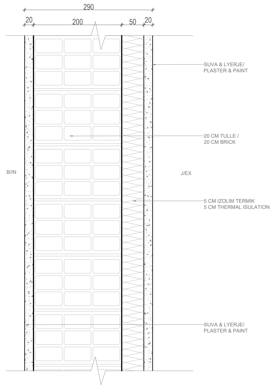
1 DETAIL EXTERNAL WALL / DETAJ MURI I JASHEM 1:5
