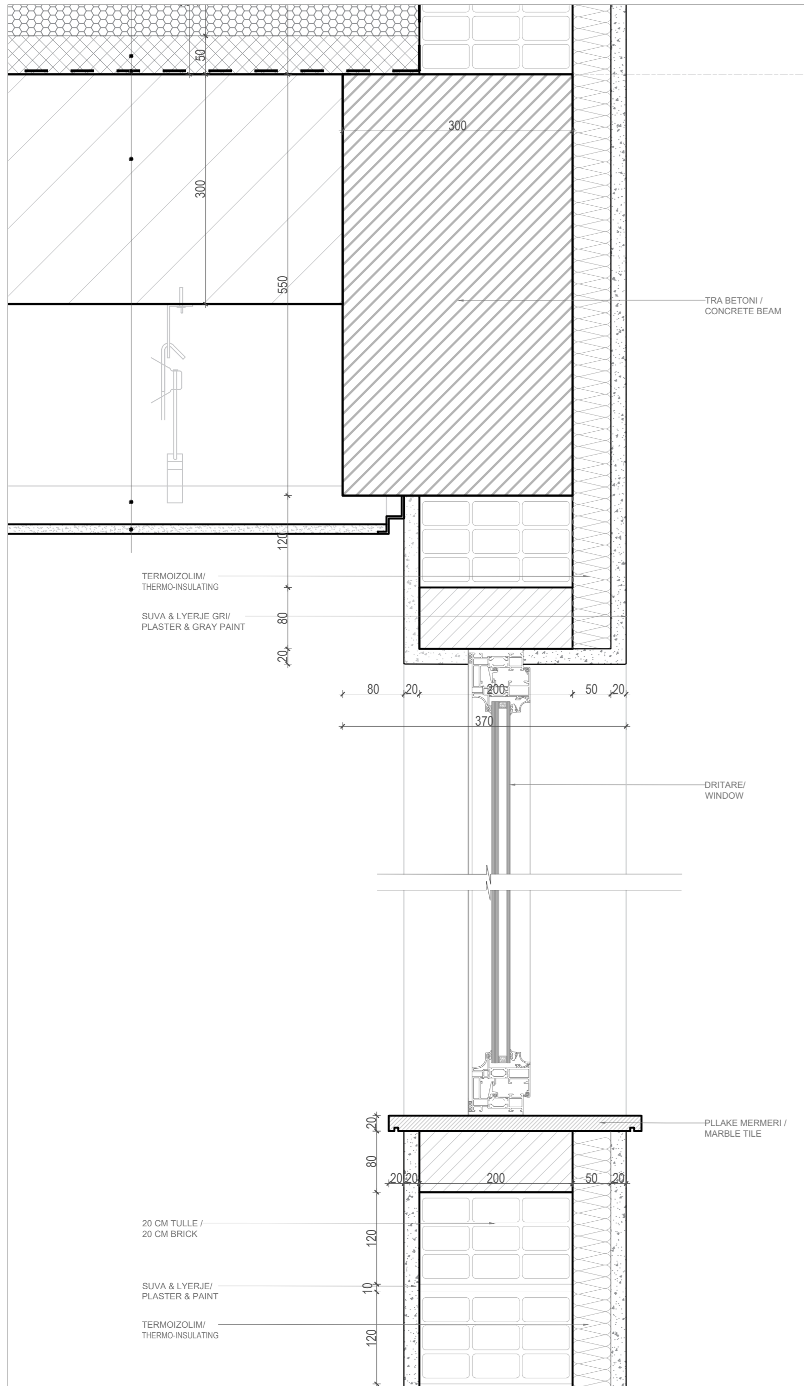
1 DETAJ I DRITARES / WINDOW DETAIL SHK 1:5
