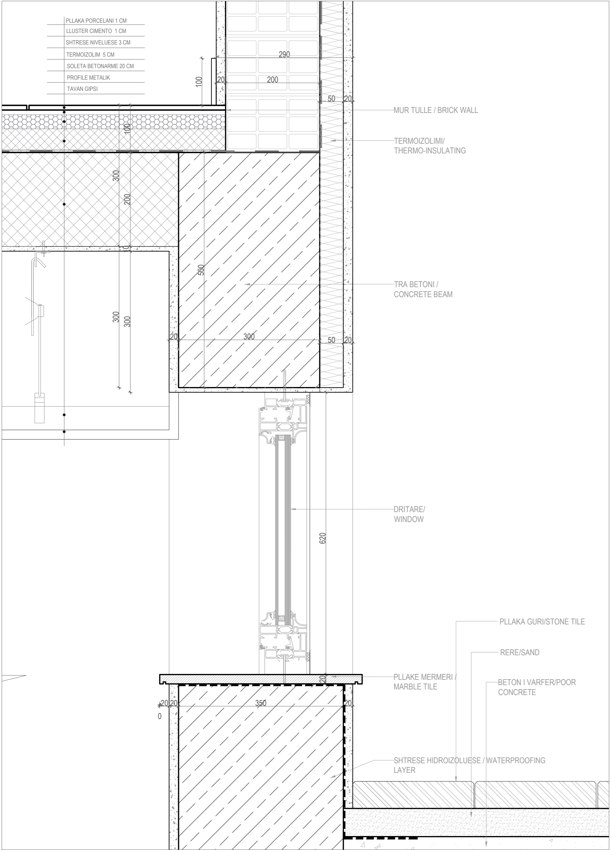
1 DETAIL UNDERGROUND / DETAJ NENTOKE SHK 1:5
