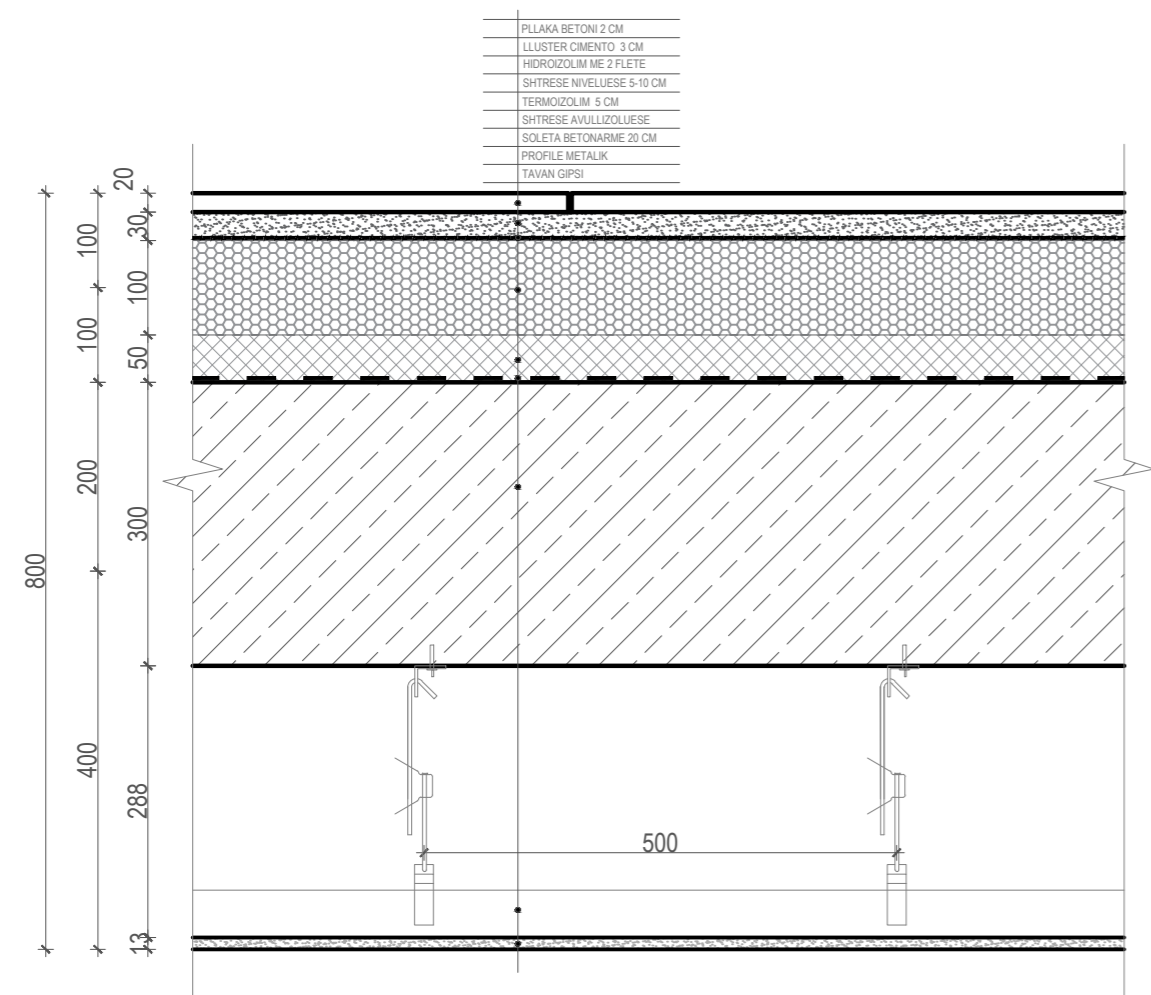
5 FLOOR DETAIL / DETAJ DYSHEMEJE 1:8
