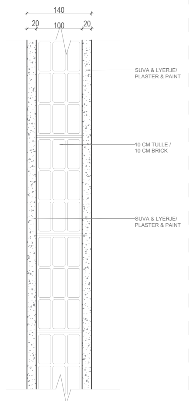
3 DETAIL INTERNAL WALL / DETAJ MUR I BRENDSHEM 1:5
