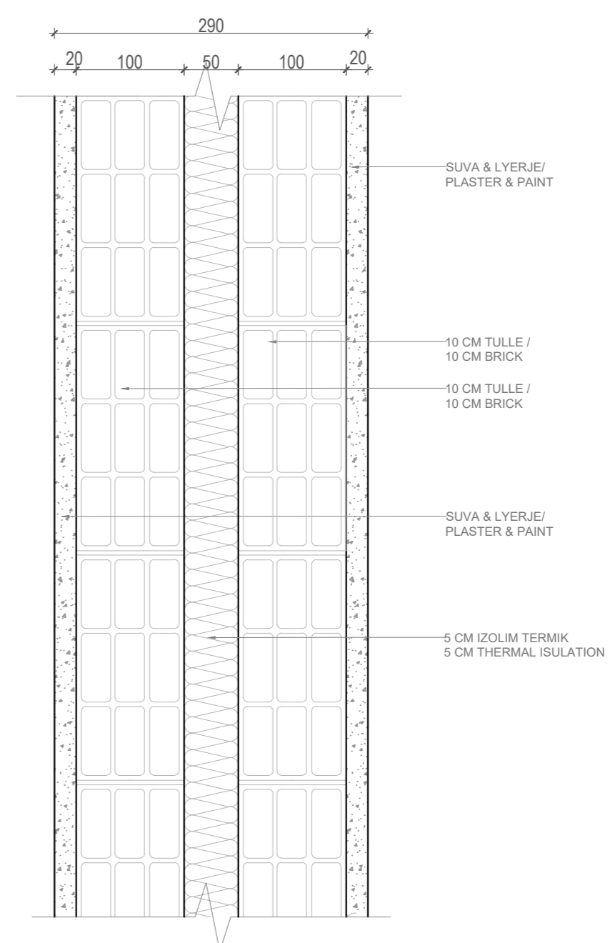
4 DETAIL CLASS WALL / DETAJ MUR KLASHE 1:5
