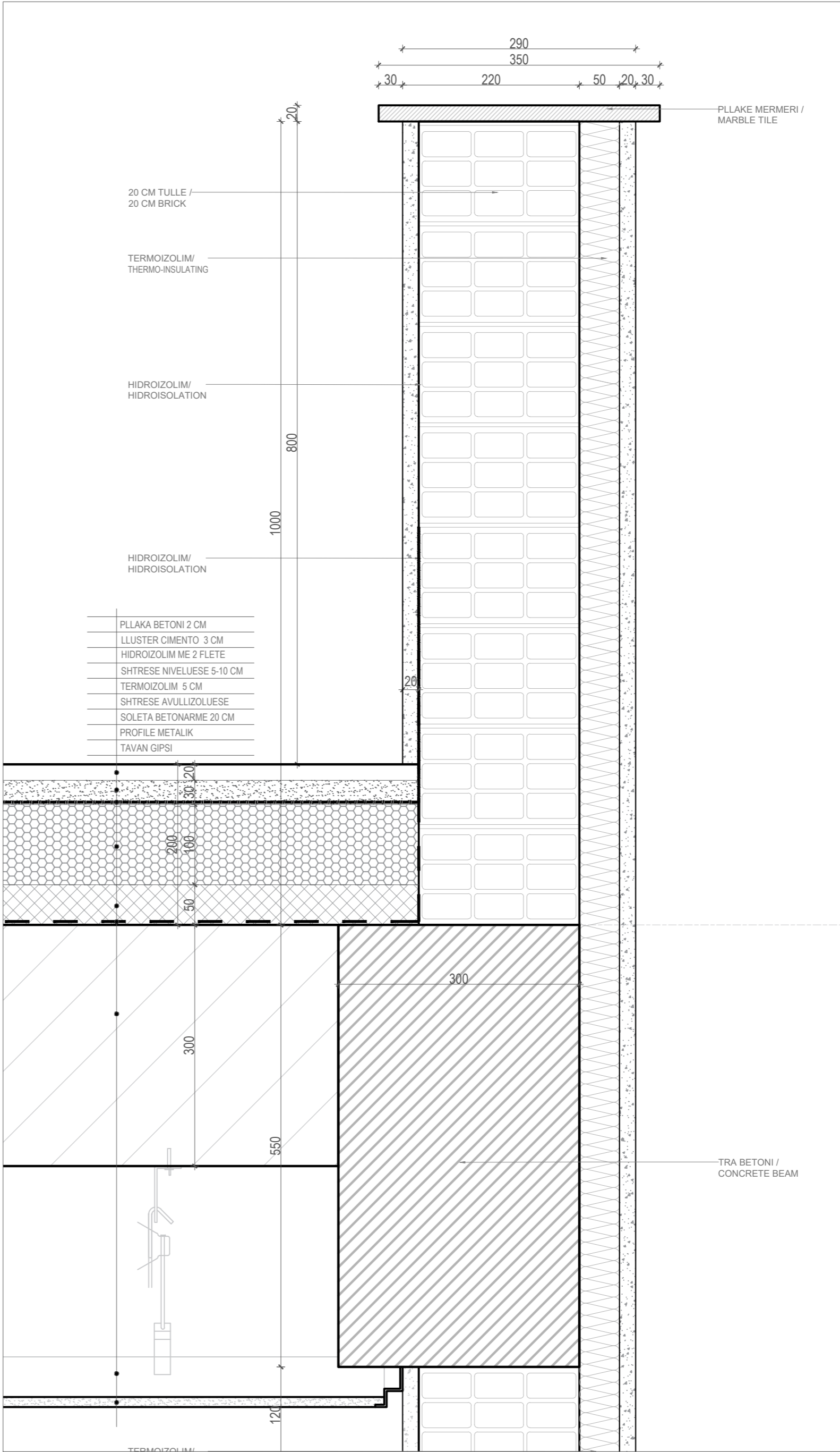
2 DETAIL TERRACE / DETAJ TARRACE SHK 1:5
