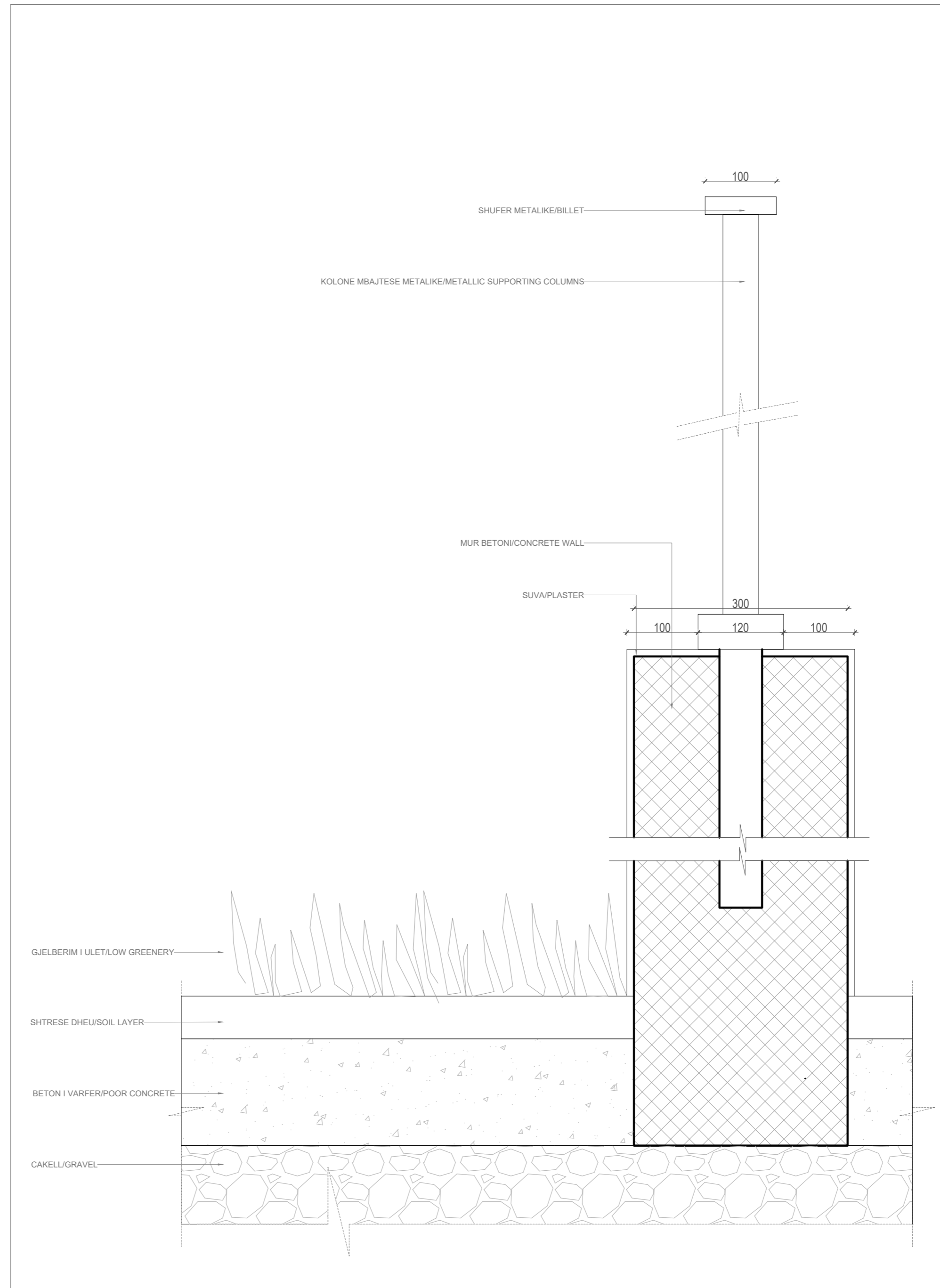
2 DETAJ I MURI RRETHUES / SURROUNDING WALL DETAIL SHK 1:5
