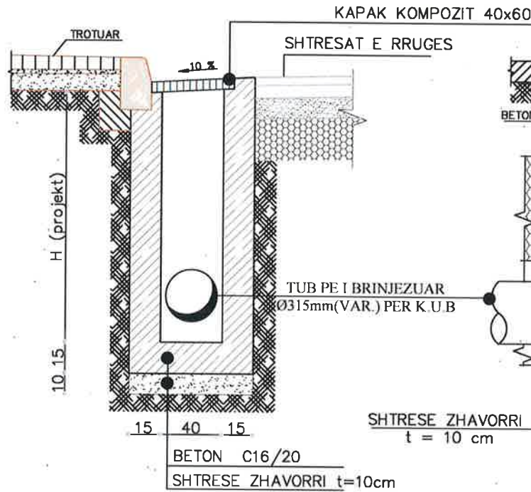
PRERJE B-B (PER TUBA HDPE D=315MM) SH- 1:25
