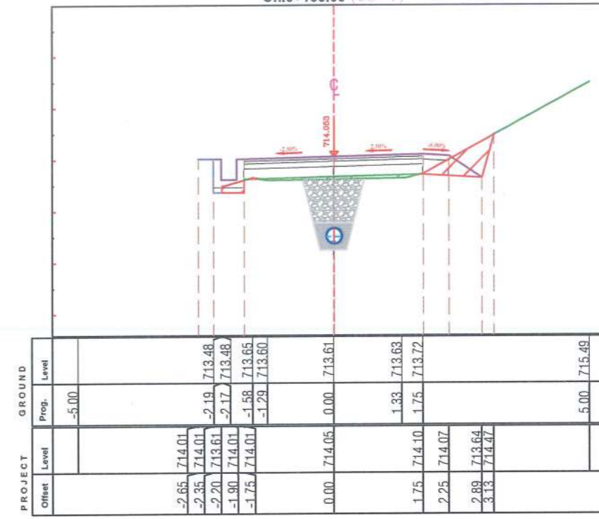
Ch.0+150.00 (CS-7)
