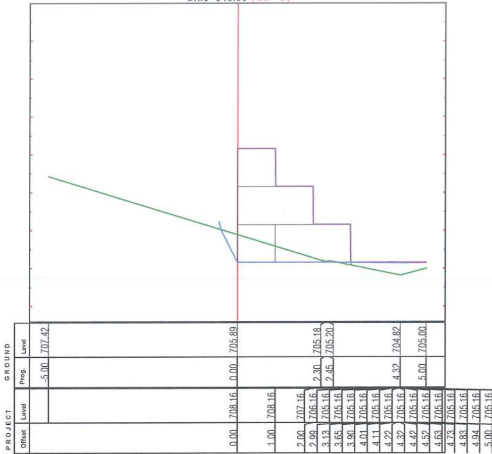
Ch.0+040.00 (CS-3)
