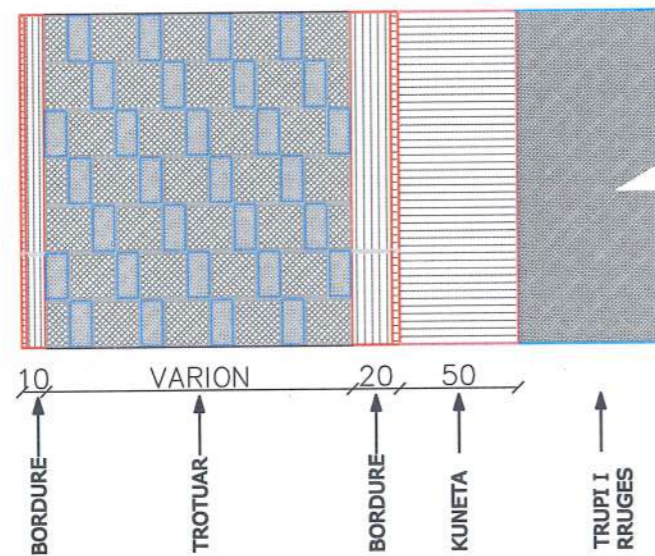
PLAN PLANIMETRIA
