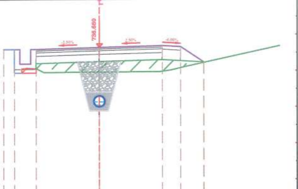
Ch.0+375.00 (CS-16)
