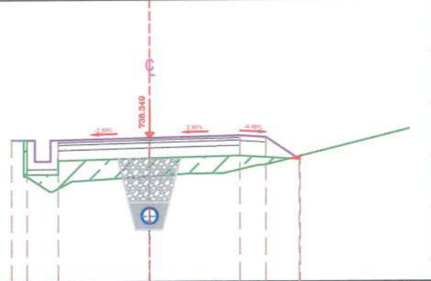
Ch.0+400.00 (CS-17)
