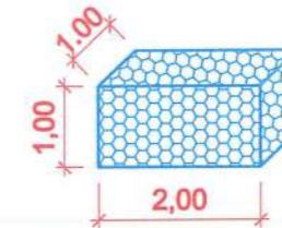
Mattress Gabions At Base of Wall Gabionet e Qilimit Ne Bazen e Murit
