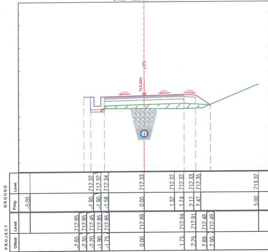
Ch.0+125.00 (CS-6)
