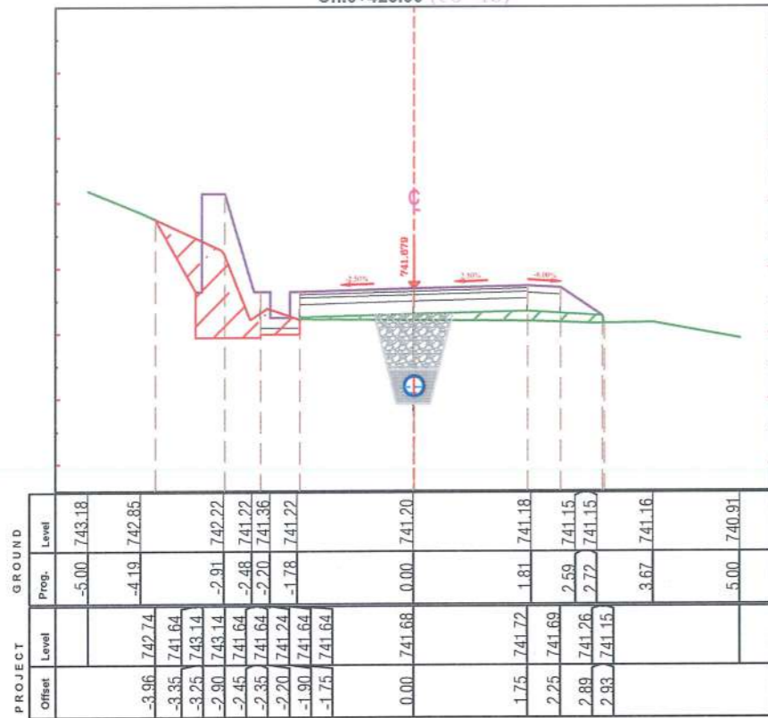
Ch.0+425.00 (CS-18)
