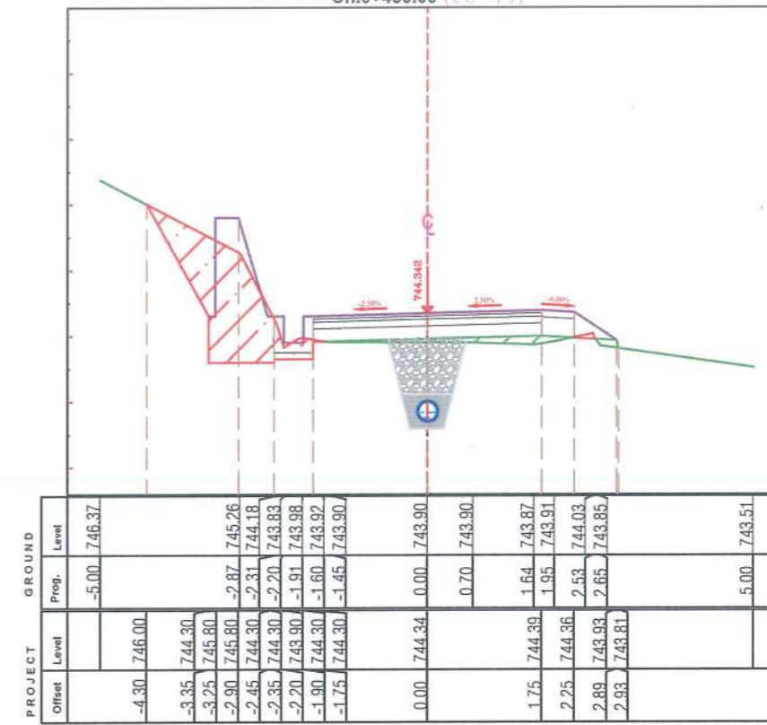
Ch.0+450.00 (CS-19)
