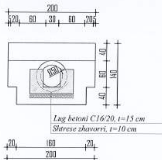
PRERJA B-B SH. 1:50
