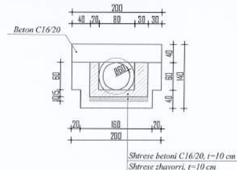
PRERJA D-D SH. 1:50
