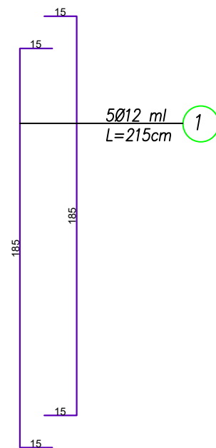
PRERJA B-B SH:1/25
