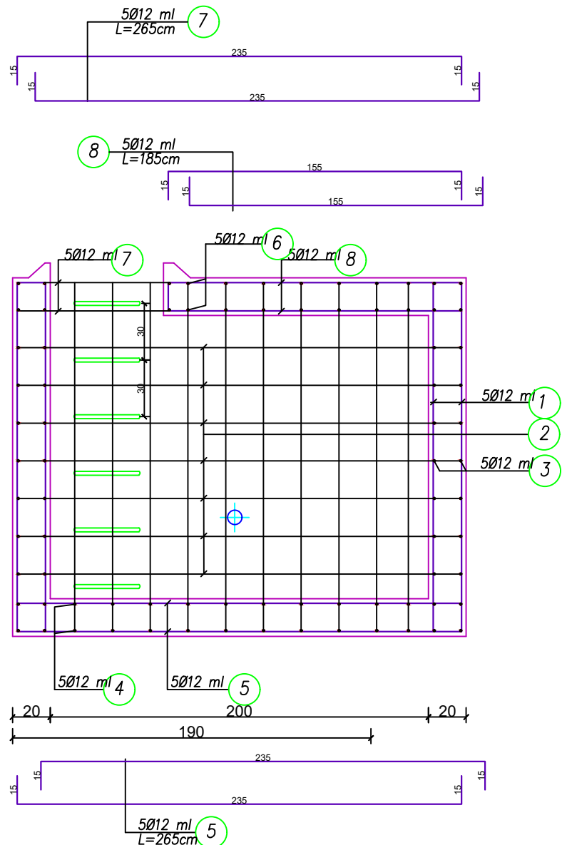
PRERJA B-B SH:1/25
