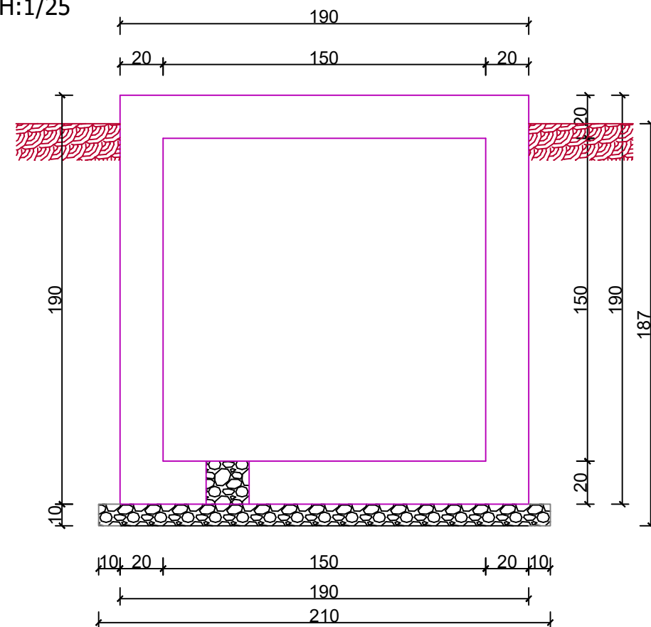
PRERJA B-B SH:1/25
