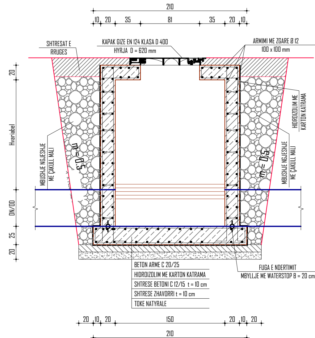
KAPAKU | GIZES
