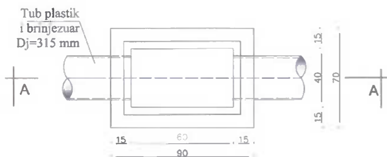
PLANIMETRIA SH. 1:20
