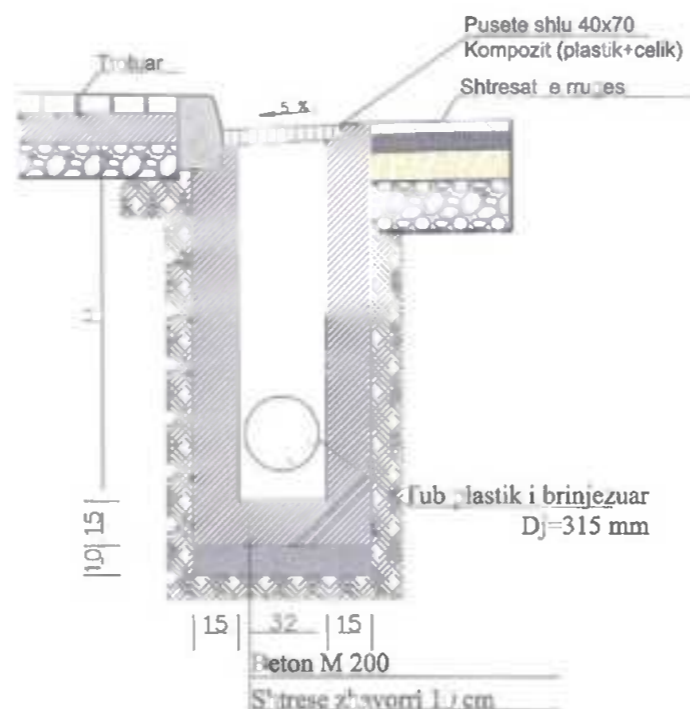
PRERJE B-B SH. 1:20
