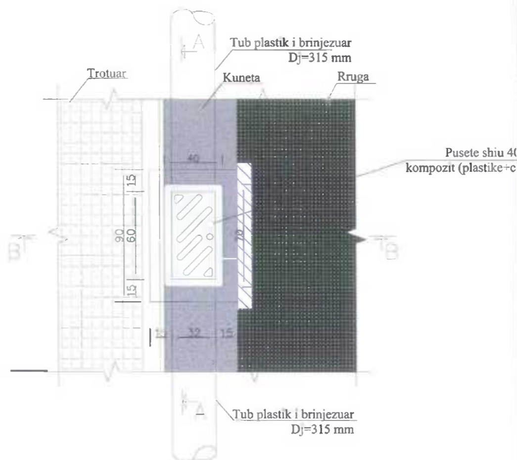
PLAN SH. 1:20
