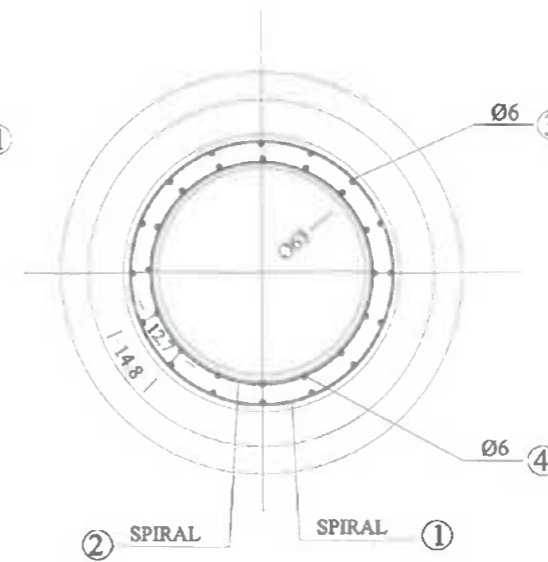
PLAN SHK.1:20
